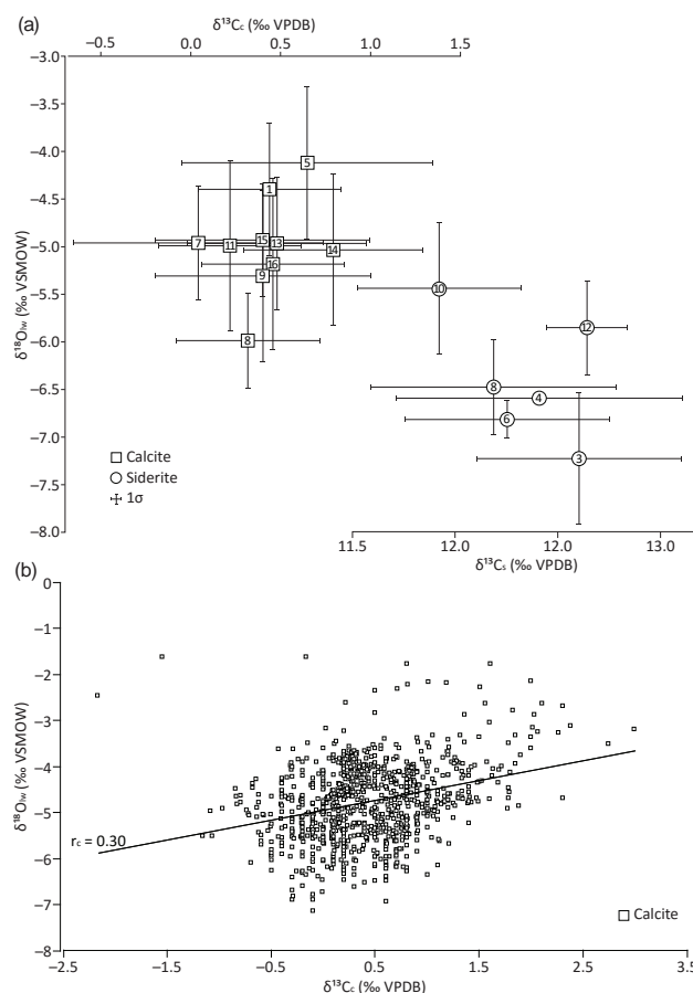
Figure 7. (a) \delta^{18}\text{O}_{\text{lw}}-\delta^{13}\text{C}_{\text{c}} and \delta^{18}\text{O}_{\text{lw}}-\delta^{13}\text{C}_{\text{s}} cross-plot showing the average and standard deviation ( 1\sigma ) of each MIS (numbered centre points) for both calcite and siderite data; (b) \delta^{18}\text{O}_{\text{lw}}-\delta^{13}\text{C}_{\text{c}} cross-plot showing all calcite data and linear regression with Pearson correlation ( r ) (calcite r_{\text{c}} , p < 0.001 ). (a) and (b) both include the Lini site Holocene Co1262 calibration data set (Lacey et al., 2015).
