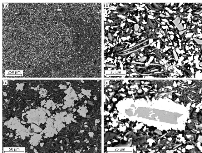
Figure 6. Backscatter scanning electron microscopy images of glacial sediment thin sections, showing (a) areas of high (brighter) and low (darker) siderite concentration in “burrow-like” structure, (b) areas of high siderite concentration (white euhedral crystals) in an open-packed matrix (note: central diatom appears split by siderite crystal), (c) individual siderite crystals amalgamating to form a larger siderite crystal cluster, and (d) siderite overgrowth fringing a rare detrital dolomite grain.
