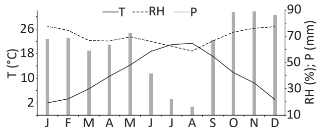
Figure 2. Recent climate data from the town of Ohrid (WMO station 135780: 41.1170^{\circ}\text{N} , 20.8000^{\circ}\text{E} ; 761 m a.s.l.) showing monthly averages over the period 2010–2014 for average temperature ( T ), precipitation ( P ), and relative humidity (RH) (data available from WMO, 2015).
