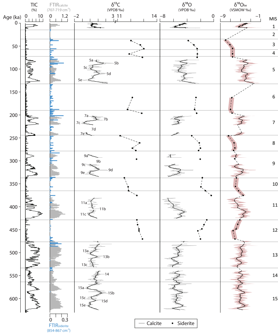
Figure 3. Isotope results from calcite ( \delta^{18}\text{O}_c , \delta^{13}\text{C}_c ), siderite ( \delta^{18}\text{O}_s , \delta^{13}\text{C}_s ), and calculated lake water ( \delta^{18}\text{O}_{lw} ) from Lake Ohrid, also showing TIC (Francke et al., 2016), the Holocene Co1262 calibration data set ( \delta^{18}\text{O}_c , \delta^{13}\text{C}_c ; Lacey et al., 2015), and MIS stratigraphy (Railsback et al., 2015). FTIR results are shown for calcite (grey bars; calcite area = 707\text{--}719\text{ cm}^{-1} ) and siderite (blue bars; siderite area = 854\text{--}867\text{ cm}^{-1} ). Calcite data are given as raw (grey line) and lowess as smooth (span = 0.02; black line); siderite data are presented as individual points (black dots). For calculation of \delta^{18}\text{O}_{lw} , +18^\circ\text{C} was assumed for calcite data (red shaded area = \pm 3^\circ\text{C} ) and +6^\circ\text{C} for siderite data (red shaded area = \pm 2^\circ\text{C} ); see text for further detail.
