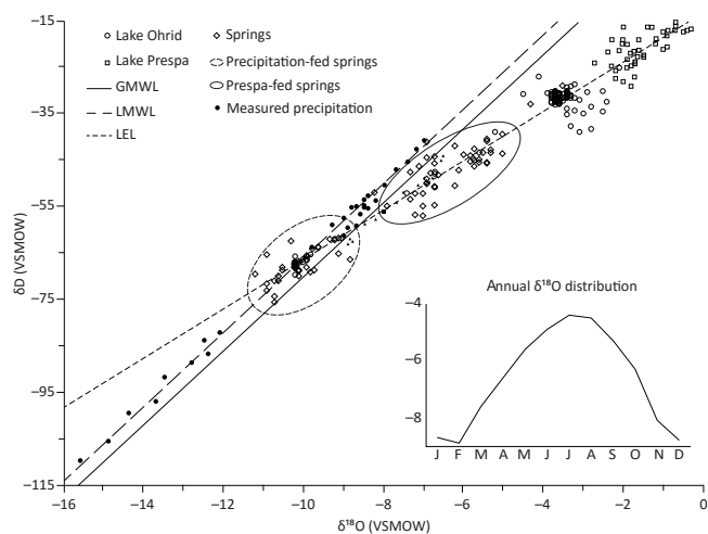
Figure 4. Modern isotope composition ( \delta^{18}\text{O} and \delta\text{D} ) of waters from lakes Ohrid and Prespa, springs, and local rainfall (Anovski et al., 1980, 1991, 2001; Eftimi and Zoto, 1997; Matzinger et al., 2006a; Jordanoska et al., 2010; Leng et al., 2010a). The Global Meteoric Water Line (GMWL; Craig, 1961), local meteoric water line (LMWL; Anovski et al., 1991; Eftimi and Zoto, 1997), and calculated local evaporation line (LEL) are given. The annual distribution of \delta^{18}\text{O} was calculated using the Online Isotopes in Precipitation Calculator (OIPC; Bowen et al., 2005; Bowen, 2015).
