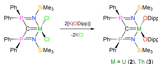
Scheme 1. Synthesis of 2 and 3 . For the synthesis of 1 see reference 18.
