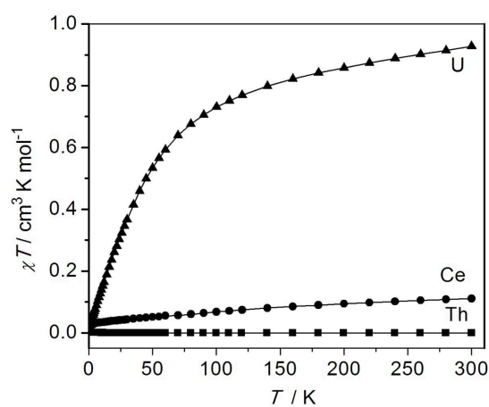
Figure 2. Magnetic data of solid samples of 1-3 , measured in 5000 G applied magnetic field. Diamagnetic corrections for 1 and 2 were estimated from the data for 3 ; the weak paramagnetism from samples of 1 is due to an impurity. 24
