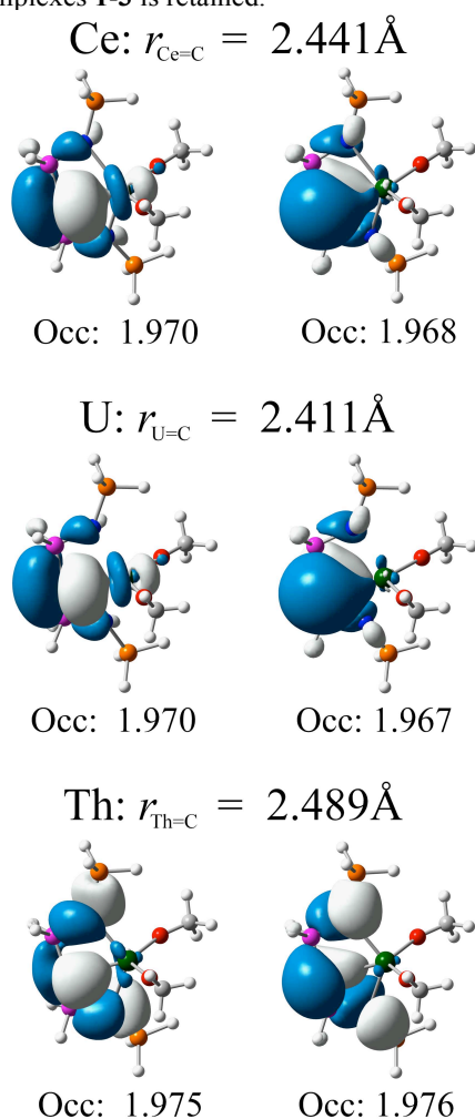
Figure 4. Relevant natural orbitals and corresponding occupancies obtained from RASSCF calculations on the truncated complexes. All orbitals rendered using an isosurface value of 0.04.
