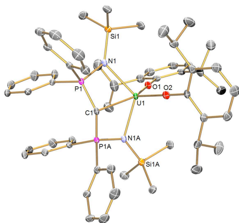
Figure 1. Molecular structure of 2 . Displacement ellipsoids set to 40% and hydrogen atoms omitted for clarity. Complexes 1 and 3 are isostructural and therefore essentially identical in appearance. Selected bond lengths (Å) for 1 : Ce1-C1 2.441(5), Ce1-N1 2.374(3), Ce1-N1A 2.374(3), Ce1-O1 2.137(4), Ce1-O2 2.130(4), C1-P1 1.692(2), C1-P1A 1.692(2), P1-N1 1.626(3), P1A-N1A 1.626(3). For 2 : U1-C1 2.414(3), U1-N1 2.349(2), U1-N1A 2.349(2), U1-O1 2.124(2), U1-O2 2.144(2), C1-P1 1.681(2), C1-P1A 1.681(2), P1-N1 1.640(2), P1A-N1A 1.640(2). For 3 : Th1-C1 2.508(5), Th1-N1 2.416(3), Th1-N1A 2.416(3), Th1-O1 2.187(4), Th1-O2 2.205(4), C1-P1 1.670(2), C1-P1A 1.670(2), P1-N1 1.640(3), P1A-N1A 1.640(3).
