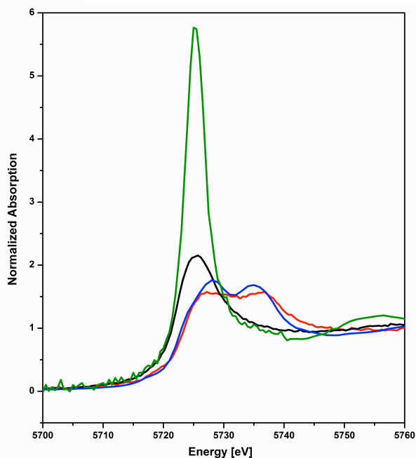
Figure 3. Cerium L III -edge XANES spectrum of the cerium(IV) complex 1 (red trace) in comparison to its cerium(III) precursor [Ce(BIPM TMS )(ODipp) 2 K(THF)] (black trace). As references, spectra of 0.01 M cerium(III) nitrate in water (green trace), and of cerium(IV) dioxide (blue trace) are given. The XANES spectra of 1 and its precursor were recorded at 15 K and the references were recorded at 298 K.
