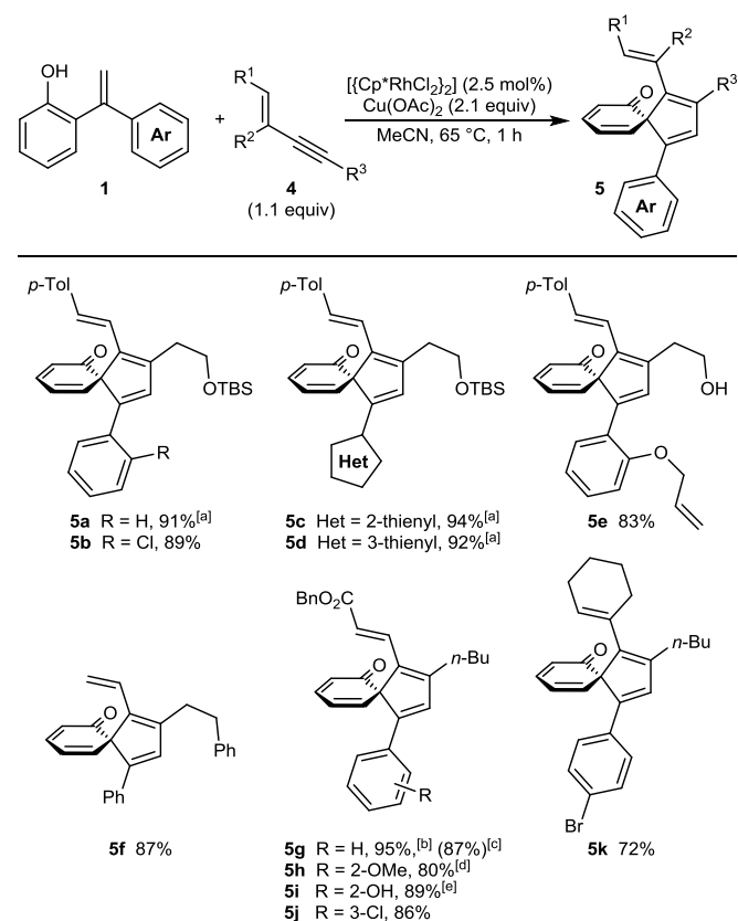
Scheme 2: Reactions of 2-[1-(hetero)arylalkenyl]phenols with conjugated enynes. Reactions proceeded with >19:1 regioselectivity in all cases. Yields are of isolated single regioisomers. [a] Reaction time was 15 min. [b] Reaction time was 30 min. [c] Reaction conducted with \text{Cu}(\text{OAc})_2 (5 mol%) under air at 85 °C for 5 h. [d] Using 1.2 equiv of enyne. [e] Reaction conducted at 40 °C for 2 h.
