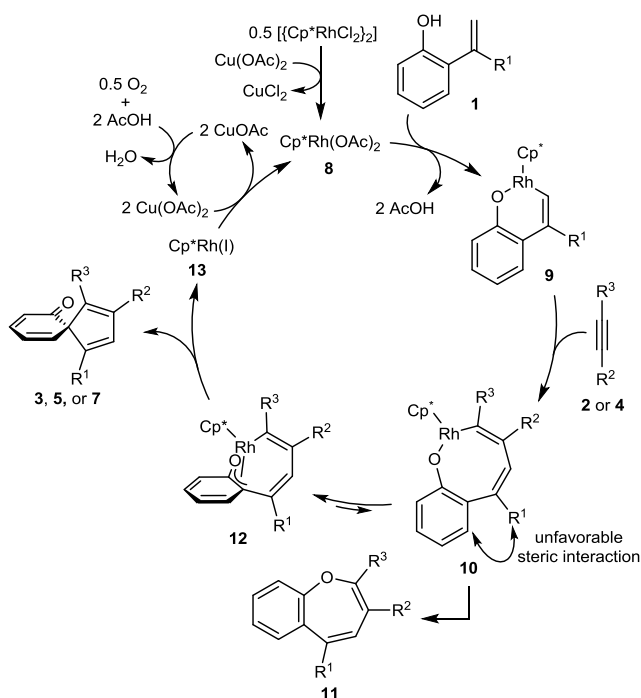
Scheme 3: Possible catalytic cycle.
