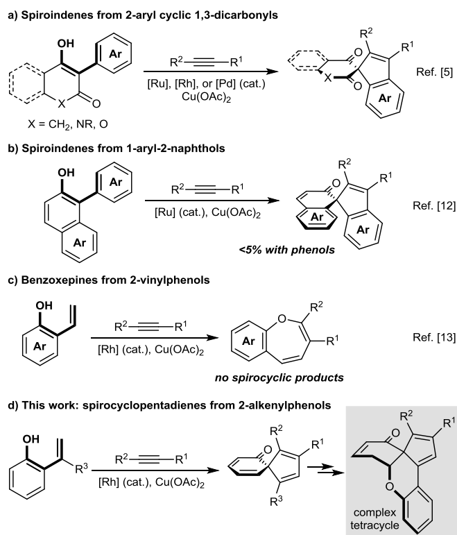
Scheme 1. Oxidative annulations of related substrates with alkynes.
