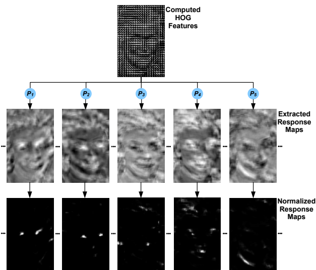
(d) Overview of Response Map Based Texture Model. After computing HOG features for test image in (a), we convolve them with the discriminatively pre-trained filters ( P_1, \dots, P_5 ) for each landmark. The responses are then normalized using a simple logistic function so that the values lie between 0 and 1. These normalized responses form the bases for the proposed response map based texture model.
