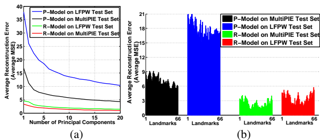
Fig. 3: Pixel Value based (P-Model) vs. Response Map based texture model (R-Model). (a) For the patch around Left Eye Corner , using upto top 20 PCA components. (b) For all landmark points, using top 5 PCA components.
