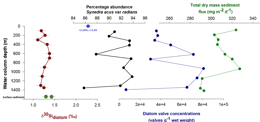
Figure 4. Open sediment trap (2012–2013) data from site BAIK13-1, south basin Lake Baikal (brown symbols). Samples are displayed along a y axis of water column depth. \delta^{30}\text{Si}_{\text{diatom}} data (‰) are expressed with respective analytical errors ( 2\sigma ) and surface sediment samples from cores BAIK13-1C and BAIK13-4F are also displayed (green symbols) along with the mean March surface (2013) water composition (blue symbol). Percentage abundance of the dominant diatom Synedra acus var radians , diatom concentrations (valves \text{g}^{-1} wet weight) and total dry mass sediment fluxes ( \text{mg m}^{-2} \text{d}^{-1} ) are also provided. All data apart from diatom concentrations are presented in Table 2.
