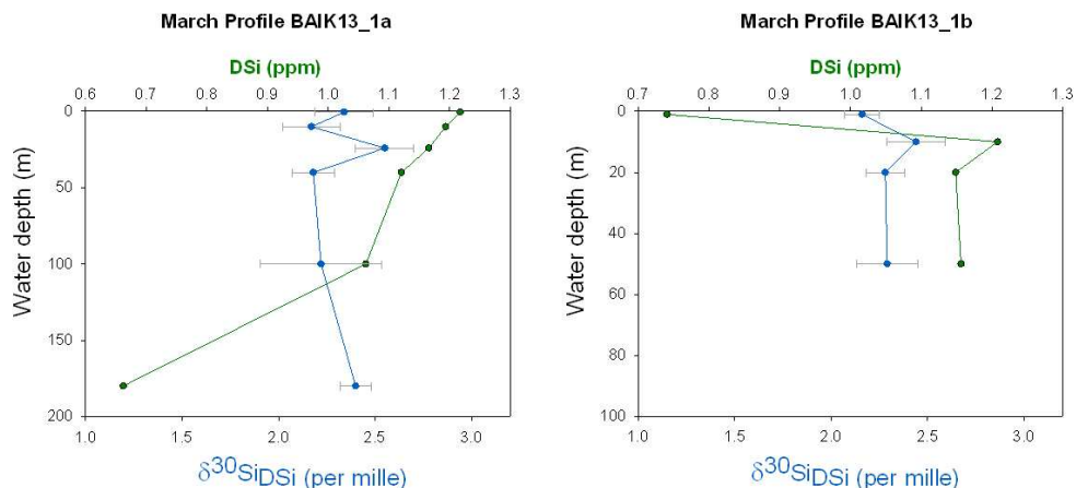
Figure 3. Depicting water column sampling from Lake Baikal (180 m below surface) of DSi concentrations (ppm) shown in green and \delta^{30}\text{Si}_{\text{DSi}} (‰) signatures in blue. The two sampling intervals (BAIK13-1a and 1b) from March 2013 are both displayed. Note the different sampling depths for these two data sets. All analytical errors of uncertainty are shown in grey ( 2\sigma ). All data correspond to Table 1.
