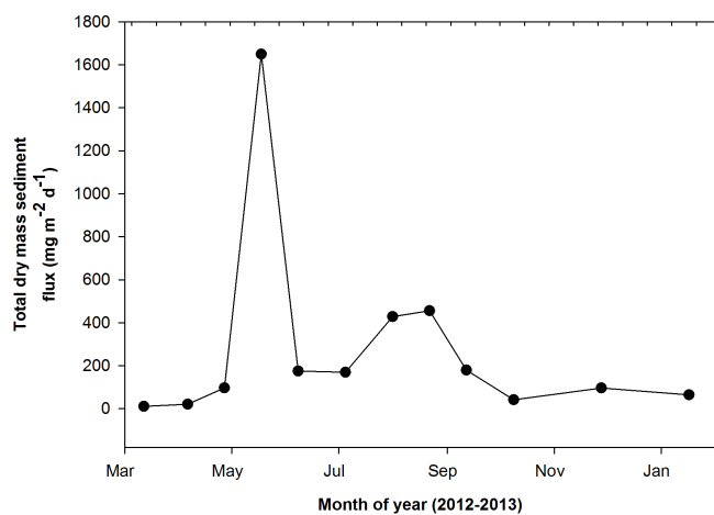
Figure 5. Total dry mass sediment fluxes ( \text{mg m}^{-2} \text{d}^{-1} ) for monthly sequencing traps, positioned at 100 m water depth in the South Basin of Lake Baikal (2012–2013).
