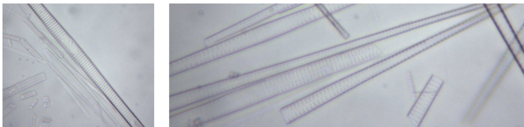
Figure 2. Light microscopy images of open trap diatom species from Lake Baikal ( \times 1000 ). Images show the purity of samples used for \delta^{30}\text{Si}_{\text{diatom}} analyses.
