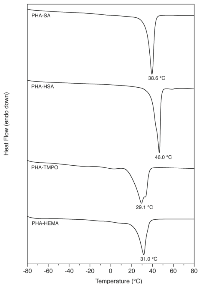
Figure 4 – DSC traces of PHA with different end-functionalisation. PHA-HSA displays the highest T_m (46.0 °C), whilst PHA-TMPO shows the lowest one (29.1 °C)
