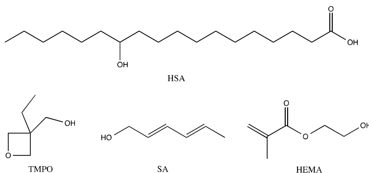
Figure 2 - The functional end-cappers used in this study.
