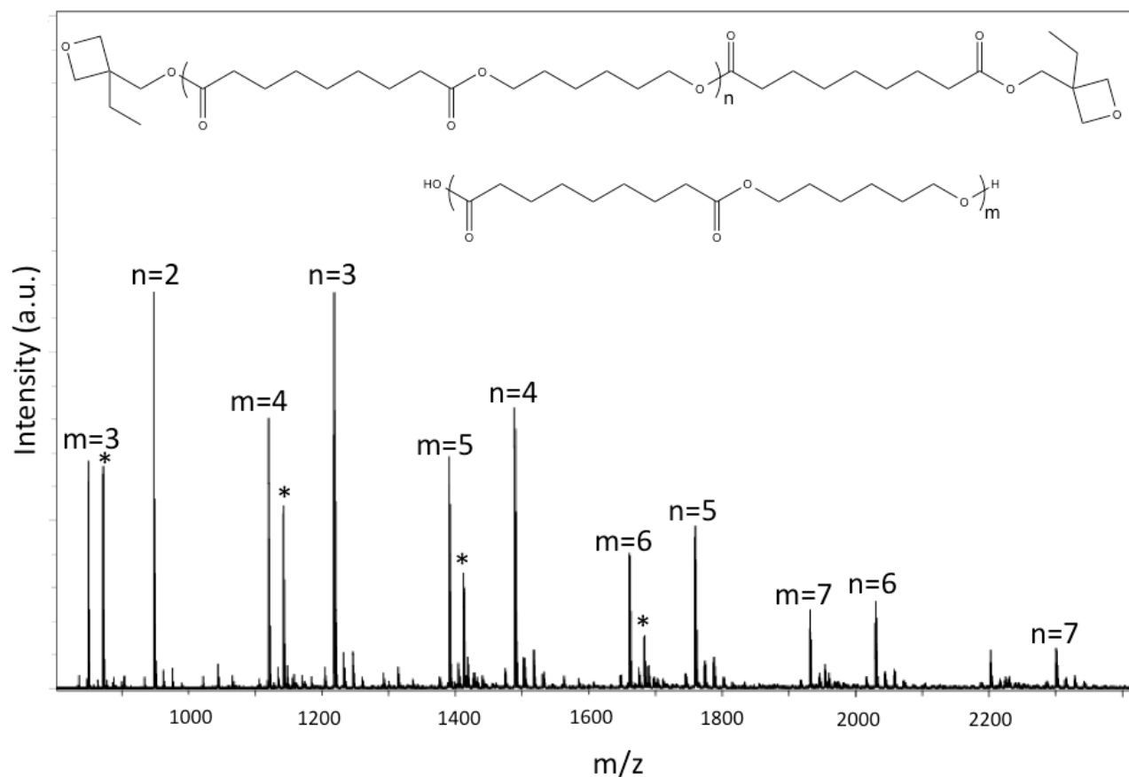
Figure 9 – MALDI-TOF spectrum of PHA-TMPO. (n) di-functional product; (m) AB-type chains with acid and alcohol end-group; (*) AB-type chains with a sodium carboxylate and an alcohol end.
