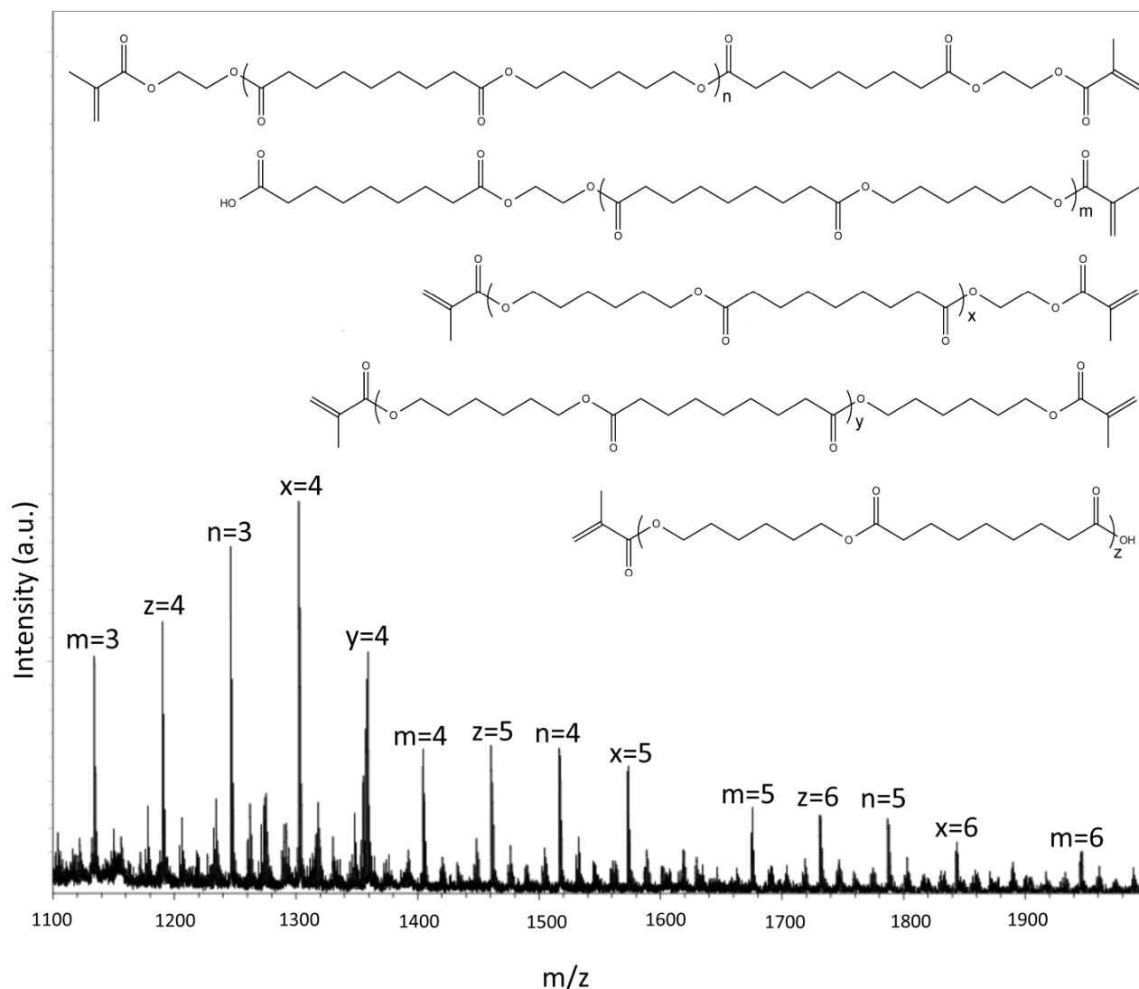
Figure 10 - MALDI-TOF spectrum of PHA-HEMA. Different species can be identified. (n), (x) and (y) are telechelic chains; (m) and (z) are mono-functional chains.
