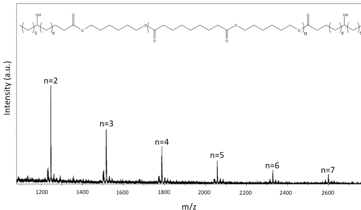
Figure 8 - MALDI-TOF spectrum of PHA-HSA. The main series (n) is given by the telechelic chains. No other species are detected.
