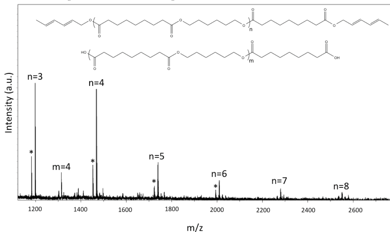
Figure 7 – MALDI-TOF spectrum of PHA-SA. The main series ( n ) is assigned to the telechelic chains ionised with \text{K}^+ . Satellite signals at lower m/z (*) are given by chains with \text{Na}^+ ions. The peak m can be assigned to a non-functional (AB) n A-type chain with DP4.
