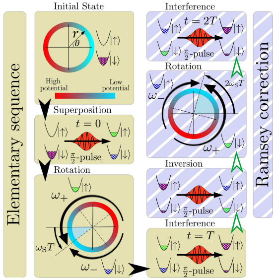
Figure 1. Experimental sequence. The situation is depicted in an inertial frame. Starting with atoms prepared in |\downarrow\rangle located at \theta = 0 , a \pi/2 -pulse generates a superposition of two non-degenerate internal states. Atoms in |\uparrow\rangle are then transported along a circular path in (anti-)clockwise direction. After a half-revolution, a second pulse converts any phase shift into population difference, which is measured in the elementary sequence (black arrows). An extended Ramsey sequence (green arrows) can be used to achieve full common path operation. Here, the \pi/2 -pulse at time T is extended to a \pi -pulse, fully inverting the atomic states. Transport is continued such that all atoms complete a full revolution before converting and measuring the phase difference at time 2T .
