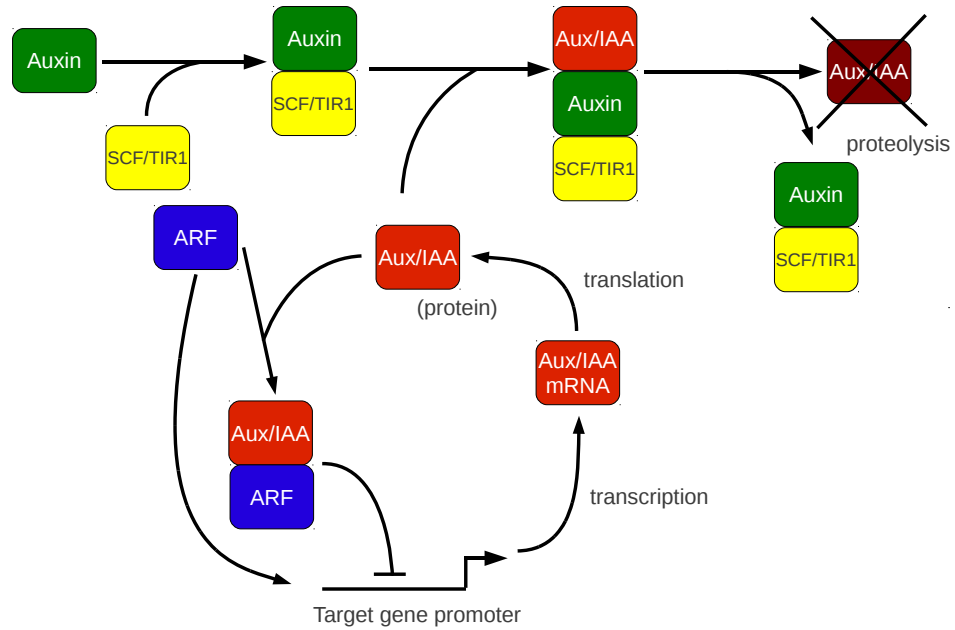
Figure 1.4: Auxin binds with the SCF TIR1 complex, which is then able to bind Aux/IAA. The Aux/IAs are then be ubiquitinated and targeted for degradation by the 26S proteasome. The ARFs, free from dimerisation with Aux/IAs, are then able to activate auxin responsive genes. When Aux/IAA is bound to on the target gene promoter ARF transcription is repressed. Unless stated the arrows represent binding of the different biomolecular complexes. (Figure adapted from Middleton et al. (2010))
