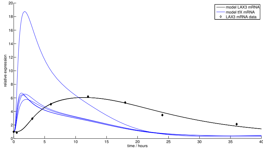
Figure 2.17: Best fits of the LAX3 mRNA in the model given by (2.21a)-(2.21g) (black lines) with the qRT-PCR data from figure 1.9 (black diamonds). Also shown are the predictions for tfX for each parameter set fitted. Five separate parameter sets are shown in total. While as may be expected there is consistency in the model prediction for LAX3, and good agreement with the data, there are variations in timing and magnitude of response for the predictions for tfX.
