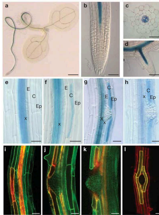
Figure 1.7: Spatial expression of LAX3, detected using the LAX3:GUS marker line in (a) seedling root stele, (b) expanding root stele cells, (c) stele in radial cross section of root, (d) stele of root with emerged lateral root, (e) root section with stage I primordium, (f) stage II primordium (g) stage V primordium and (h) stage VII primordium. From stage II onwards LAX3:GUS is visible in the cortical cells over the developing LRP. LAX3pro:LAX3-YFP expression in cortical cells above (i) stage III, (j) stage V and (k) stage VII primordia. (l) LAX3pro:LAX3-YFP expression in epidermal cells separating to allow for emergence of LRP. (Reproduced from Swarup et al. (2008).)
