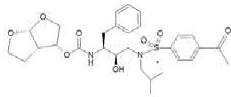
FIGURE 1 Structural formula of the API, a poorly soluble HIV protease inhibitor.
