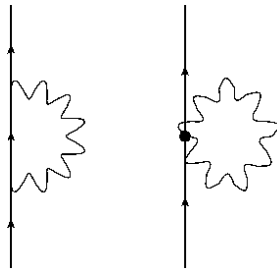
Figure 7.2: Fermion self-energy diagrams at one loop
