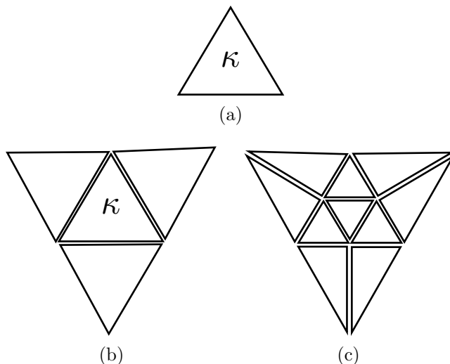
FIGURE 1. Local element patches in two–dimensions, when triangular elements are employed. (a) Original element \kappa (assumed to be an interior element); (b) Mesh patch \mathcal{T}_\kappa^{\mathcal{N}} , which consists of the element \kappa and its neighbours; (c) Mesh patch \mathcal{T}_{\kappa,\text{ref}}^{\mathcal{N}} which is constructed based on isotropically refining \kappa (red refinement) and on a green refinement of its neighbours.
