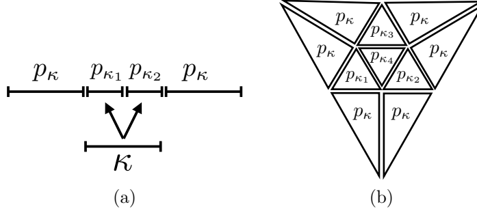
FIGURE 2. Polynomial degree distribution employed for the competitive hp -refinements: (a) One–dimension; (b) Two–dimensional triangular element.
