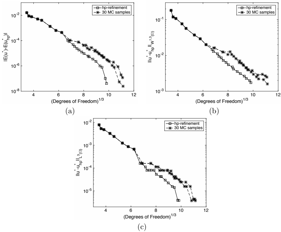
FIGURE 7. Example 3. Comparison of the error with respect to the third root of the number of degrees of freedom: (a) |\mathbb{E}(u^*) - \mathbb{E}(u_{hp}^*)| ; (b) \|u^* - u_{hp}^*\|_{W^{1,3}(\Omega)} ; (c) \|u^* - u_{hp}^*\|_{L^3(\Omega)} .
