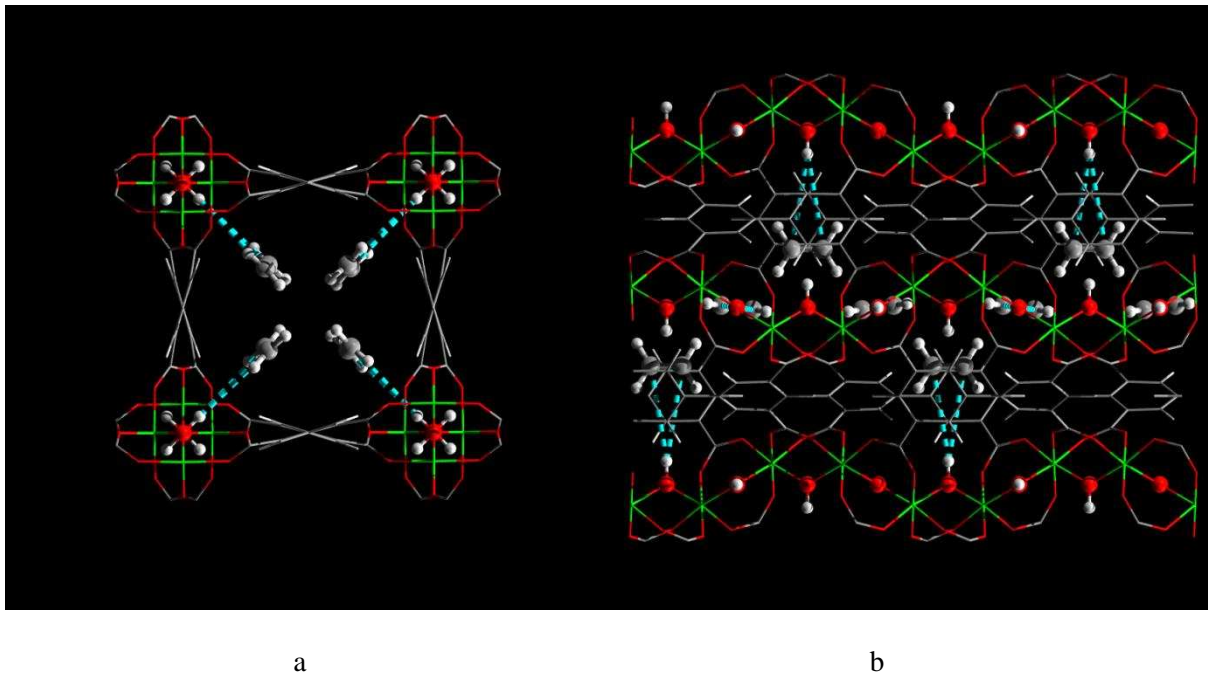
Figure 19. View of the structure of NOTT-300-C 2 H 4 E (a) along the c-axis and (b) along the a-axis. The structure was obtained by DFT simulation. The adsorbed C 2 H 4 molecules in the pore channel are highlighted by the use of ball-and-stick style.
