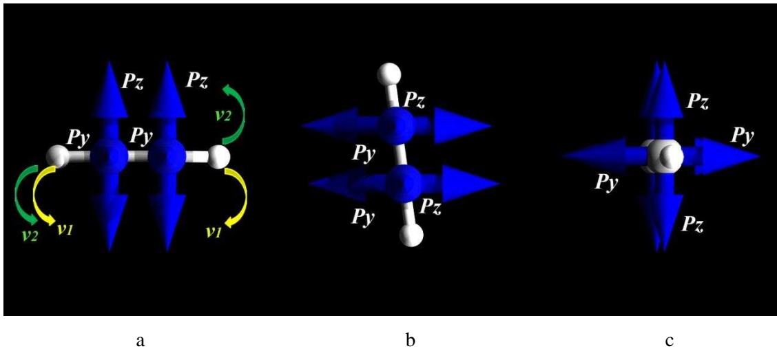
Figure 38. Views of the \pi -orbitals of P_y , P_z for free C_2H_2 molecules along (a) the a-axis, (b), the b-axis and (c) the c-axis ( P_y and P_z orbitals are highlighted in blue). P_y and P_z are equivalent to each other in free C_2H_2 molecules.
