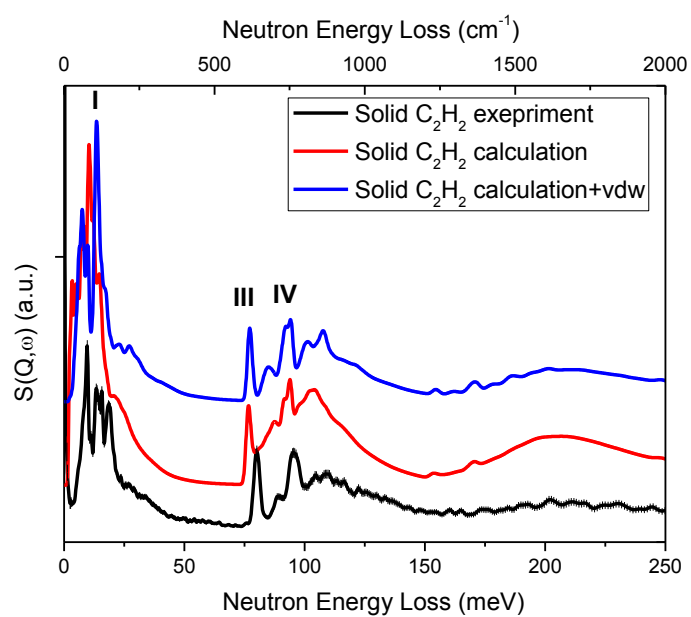
Figure 46. Comparison of the experimental and calculated INS spectra of condensed \text{C}_2\text{H}_2 in the solid state. Comparison of the calculated spectra with and without van der Waals correction is shown. In general, no significant change for calculated INS spectra was observed with van der Waals correction taken into account.
