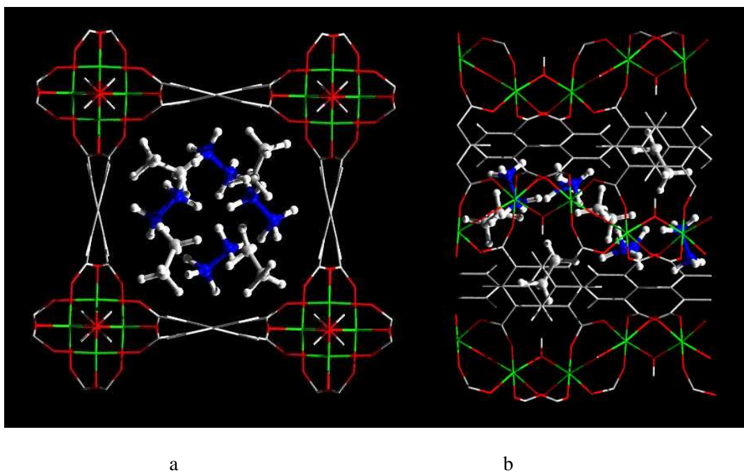
Figure 27. View of the structure of NOTT-300·1.3C 2 D 6 (a) along the c-axis and (b) along the a-axis. The structure was obtained by high resolution neutron powder diffraction, and clear positional disorder for C 2 D 6 molecules at both Site I and II can be seen. The adsorbed C 2 D 6 molecules in the channel are highlighted by the use of ball-and-stick style. The carbon atoms for C 2 D 6 (II) molecules are highlighted in blue.
