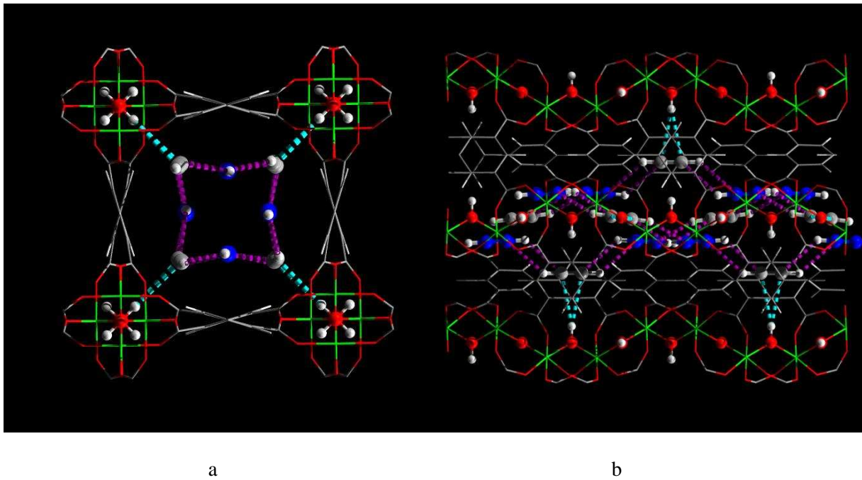
Figure 11. View of the structure of NOTT-300·3C 2 H 2 (a) along the c-axis and (b) along the a-axis. The structure was obtained by DFT simulation. The adsorbed C 2 H 2 molecules in the pore channel are highlighted by the use of ball-and-stick style. The carbon atoms for C 2 H 2 (II) molecules are highlighted in blue.
