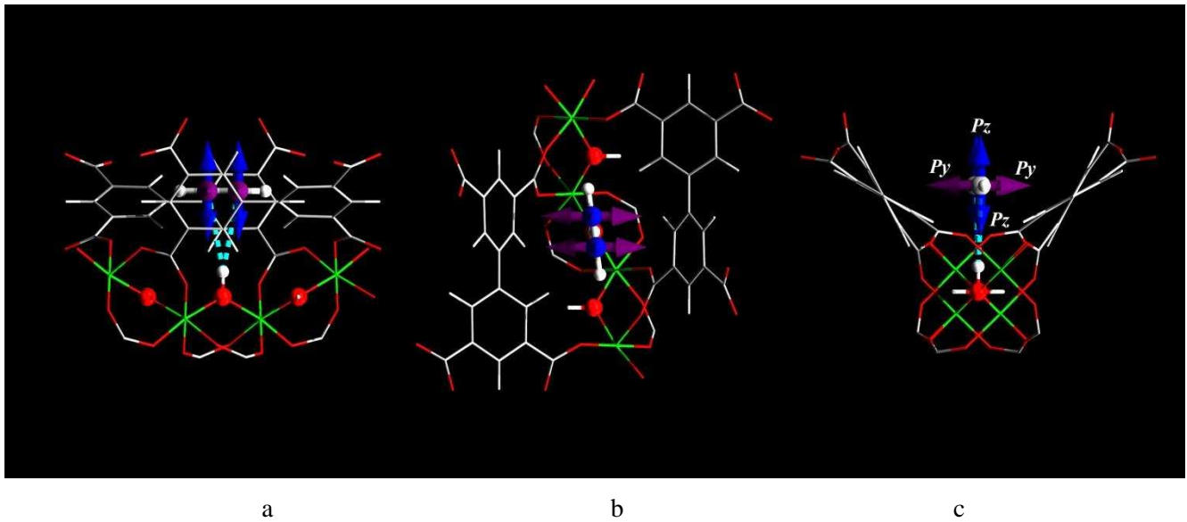
Figure 40. Model II: views of the \pi -orbitals of Py, Pz for adsorbed C 2 H 2 molecules along (a) the a-axis, (b), the b-axis and (c) the c-axis (Py and Pz orbitals are highlighted in purple and blue, respectively). Py and Pz are not equivalent to each other upon adsorption in this mode, leading to removal of degeneracy of the C-H vibrations.
