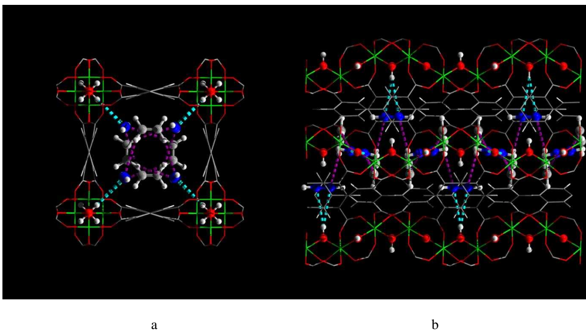
Figure 29. View of the structure of NOTT-300·2.4C 2 H 2 ·0.8C 2 H 4 (a) along the c-axis and (b) along the a-axis. The structure was obtained by DFT simulation. The adsorbed C 2 H 2 and C 2 H 4 molecules in the pore channel are highlighted by the use of ball-and-stick style.
