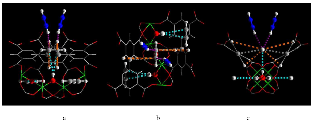
Figure 16. Detailed views of -OH, -CH, and phenyl ring groups binding C_2H_2 molecules in the functionalised cavity of NOTT-300 \cdot 4C_2H_2 . Views along (a) the a-axis, (b), the b-axis and (c) the c-axis. The structure was obtained by synchrotron X-ray powder diffraction experiments. The carbon atom on C_2H_2(II) are highlighted in blue. Clear positional disorder for C_2H_2 molecules at Site II was found. The weak hydrogen-bond between C(\delta^-) of C_2H_2 and H(\delta^+) of -OH is highlighted in cyan, [ C \cdots H = 3.43 \text{ \AA} ]. The weak cooperative supramolecular bond between C(\delta^-) of C_2H_2 and H(\delta^+) from -CH is highlighted in orange, [ C \cdots H = 3.55 , occurring twice]. The weak \pi \cdots \pi stacking interaction between \pi -electrons of C_2H_2 and phenyl rings on the ligand is highlighted in grey [ C \equiv C \cdots C_6 = 3.76 \text{ \AA} , occurring twice]. The weak electrostatic dipole interactions between C_2H_2(I) and C_2H_2(II) molecules are highlighted in purple [ C^{II} \cdots H^I = 2.75 \text{ \AA} ]. Therefore, in total, four types of weak interactions cooperatively interact together to bind C_2H_2 molecules in the functionalised cavity.
