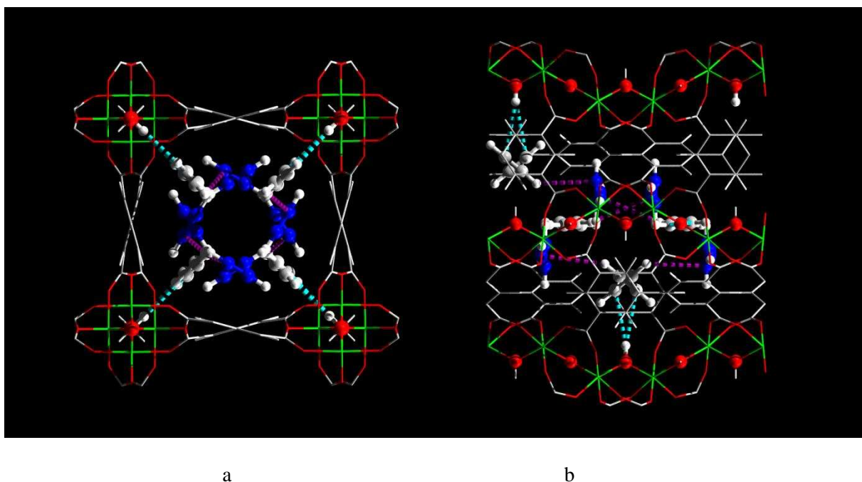
Figure 13. View of the structure of NOTT-300·2.7C 2 D 2 (a) along the c-axis and (b) along the a-axis. The structure was obtained by high resolution neutron powder diffraction. Clear positional disorder for C 2 D 2 molecules at both Site I and II can be found. The adsorbed C 2 D 2 molecules in the pore channel are highlighted by the use of ball-and-stick style. The carbon atoms for C 2 D 2 (II) molecules are highlighted in blue.
