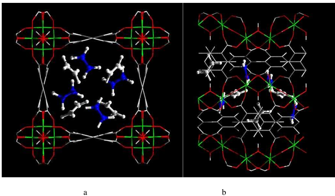
Figure 23. View of the structure of NOTT-300·1.8C 2 D 4 (a) along the c-axis and (b) along the a-axis. The structure was obtained by high resolution neutron powder diffraction, and clear positional disorder for C 2 D 4 molecules at both Site I and II can be seen. The adsorbed C 2 D 4 molecules in the channel are highlighted by the use of ball-and-stick style. The carbon atoms for C 2 D 4 (II) molecules are highlighted in blue.
