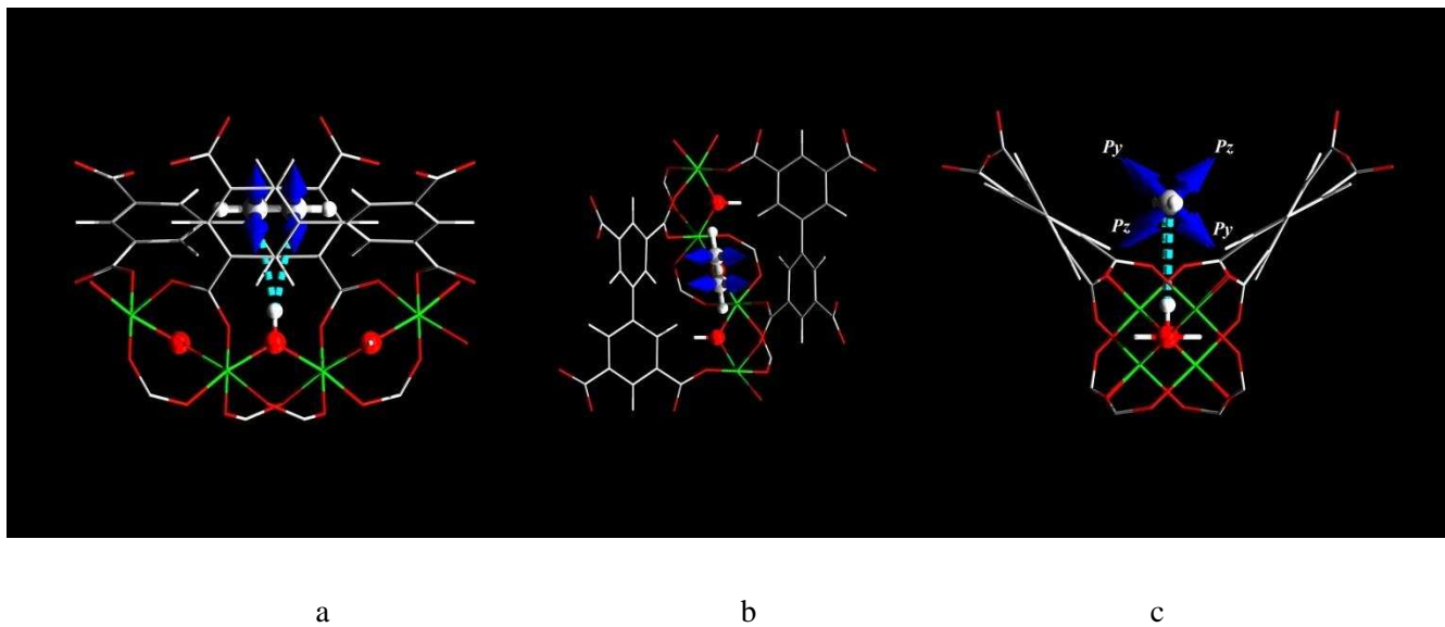
Figure 39. Model I: views of the \pi -orbitals of P_y , P_z for adsorbed C_2H_2 molecules along (a) the a-axis, (b), the b-axis and (c) the c-axis ( P_y and P_z orbitals are highlighted in blue). P_y and P_z are equivalent to each other upon adsorption in this mode, giving no change in degeneracy of the C-H vibrations.
