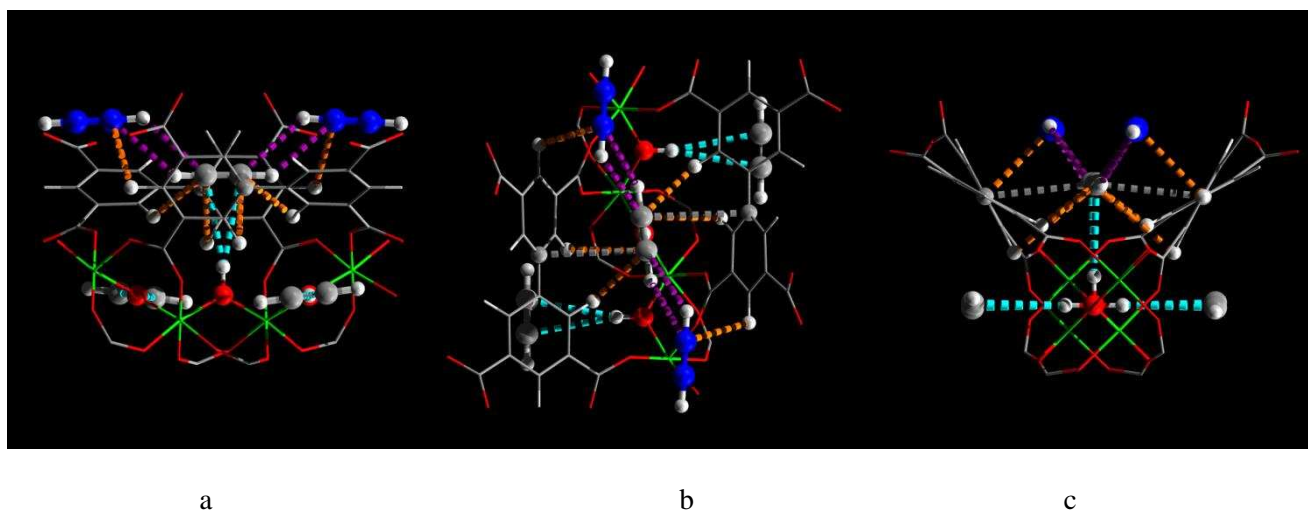
Figure 12. Detailed views of -OH, -CH, and phenyl ring groups binding C_2H_2 molecules in the functionalised cavity of NOTT-300 \cdot 3C_2H_2 . Views along (a) the a-axis, (b) the b-axis and (c) the c-axis. The structure was obtained by DFT simulation. The weak hydrogen-bond between C(\delta^-) of C_2H_2 and H(\delta^+) of -OH is highlighted in cyan, [ O \cdots H = 3.21 \text{ \AA} ]. The weak cooperative supramolecular bond between C(\delta^-) of C_2H_2 and H(\delta^+) from -CH is highlighted in orange, [ O \cdots H = 2.96, 3.64 \text{ \AA} with each occurring twice]. The weak \pi \cdots \pi stacking interaction between \pi -electrons of C_2H_2 and phenyl rings on the ligand is highlighted in grey [ C \equiv C \cdots C_6 = 3.81 \text{ \AA} , occurring twice]. The weak electrostatic dipole interactions between C_2H_2(I) and C_2H_2(II) molecules are highlighted in purple [ C^I \cdots H^{II} = 3.24 \text{ \AA} ; C^{II} \cdots H^I = 3.12 \text{ \AA} , each occurring twice]. Therefore, in total, four types of weak interactions cooperatively interact together to bind C_2H_2 molecules in the functionalised cavity.
