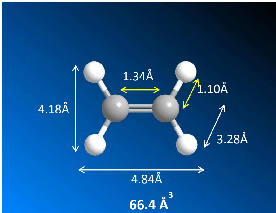
Figure 48. View of the molecular structure for C_2H_4 .
