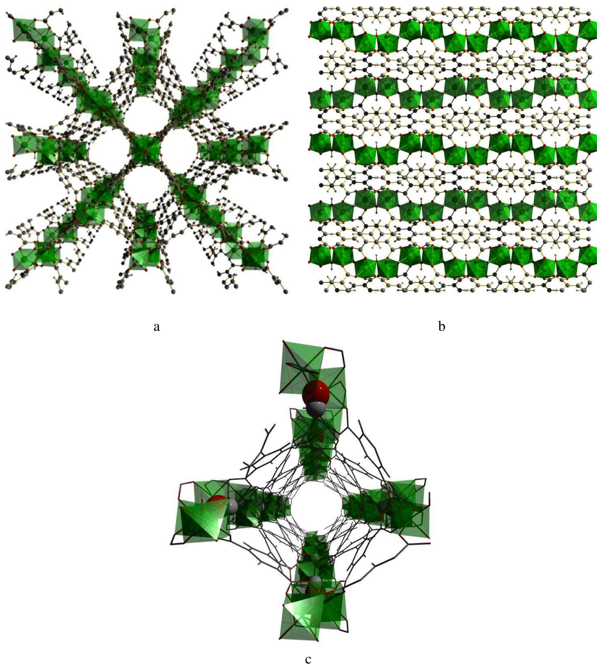
Figure 10. View of the structure for NOTT-300-solvate (a) along the c-axis and (b) along the a-axis. (c) View of the square-shaped channel. The \mu_2 -(OH) groups protrude into the centre of the channel from four directions. (Al: green; carbon: grey; oxygen: red; hydrogen: white; [\text{AlO}_4(\text{OH})_2] : green octahedron). The structure was obtained by high resolution synchrotron powder diffraction. NOTT-300 displays a surface area of 1370 \text{ m}^2 \text{ g}^{-1} , a pore volume of 0.38 \text{ cm}^3 \text{ g}^{-1} and 6.5 \text{ \AA} -wide channels decorated with free metal-hydroxyl (M—OH) groups, each with an open environment to guest molecules. The density of free hydroxyl groups is estimated as 21.2 \text{ -OH per } 1000 \text{ \AA}^2 . The distance between two adjacent —OH groups is approximately 3.22 \text{ \AA} (H \cdots H).
