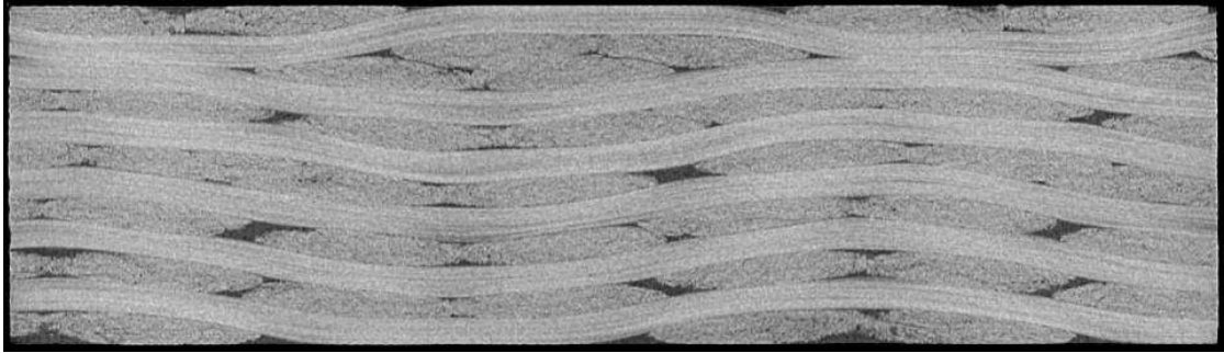
Figure 13. Cross-sectional \mu -CT data for 6 layers of the 2x2 twill weave fabric with S_0 = 660 \text{ g/m}^2 at a specimen thickness of 4 mm (same level of fabric compression as for 3 layers at 2 mm thickness); the fabric was previously unsheared; nesting was random.
