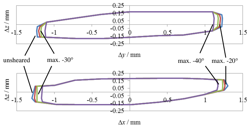
Figure 14. Typical cross-sections of yarns in a 2x2 twill weave fabric with S_0 = 660 \text{ g/m}^2 in geometrical models for resin flow simulations; \Delta x , \Delta y and \Delta z are co-ordinates relative to the centroid of the cross-sections; top: weft-yarn; bottom: warp-yarn.
