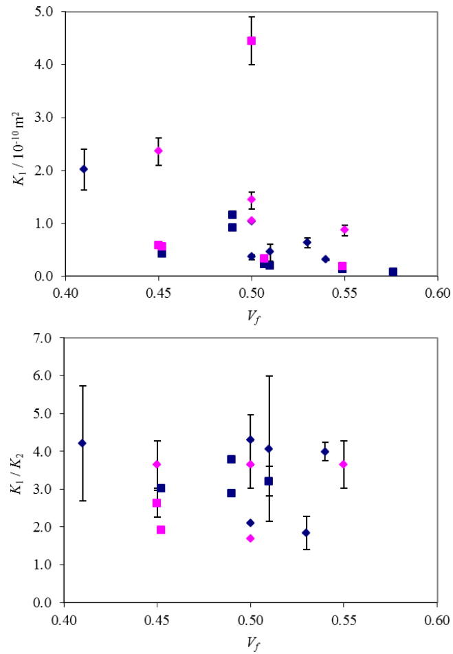
Figure 1. Scatter in permeability values measured by different laboratories for the example of a 2×2 twill weave glass fibre fabric: 1 principal permeability value, K_1 , and ratio, K_1/K_2 , as a function of fibre volume fraction, V_f ; error bars indicate standard deviations.
