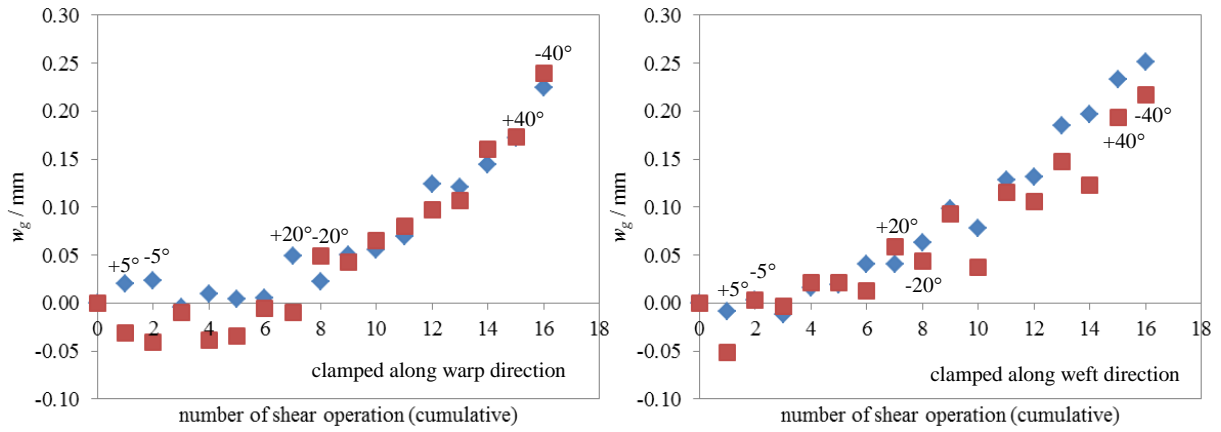
Figure 6. Average width of inter-yarn gaps, w_g , for a specimen of a 2×2 twill weave fabric ( S_0 = 660 \text{ g/m}^2 ) after undergoing different shear operations; diamond symbols: gap width between warp-yarns; square symbols: gap width between weft-yarns.
