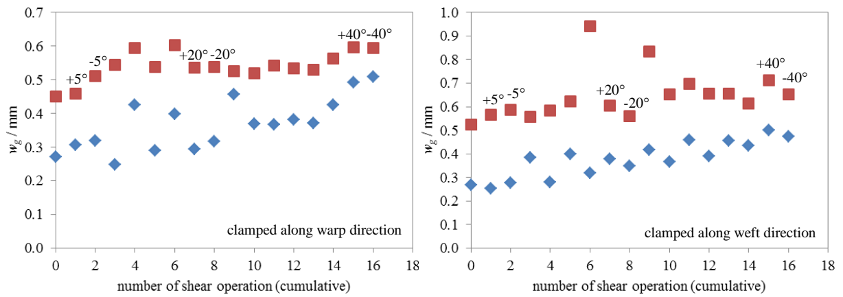
Figure 7. Average width of inter-yarn gaps, w_g , for a specimen of a 2×2 twill weave fabric ( S_0 = 285 \text{ g/m}^2 ) after undergoing different shear operations; diamond symbols: gap width between warp-yarns; square symbols: gap width between weft-yarns.
