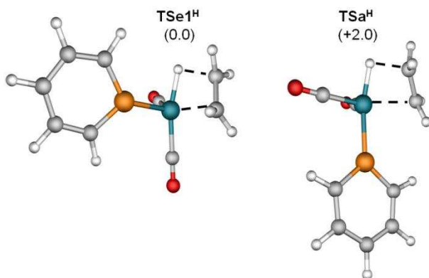
Fig. 2. Molecular structures of alkene insertion on phosphinine-Rh systems: TSe1 H and TSa H . Relative energies in \text{kcal}\cdot\text{mol}^{-1} .
