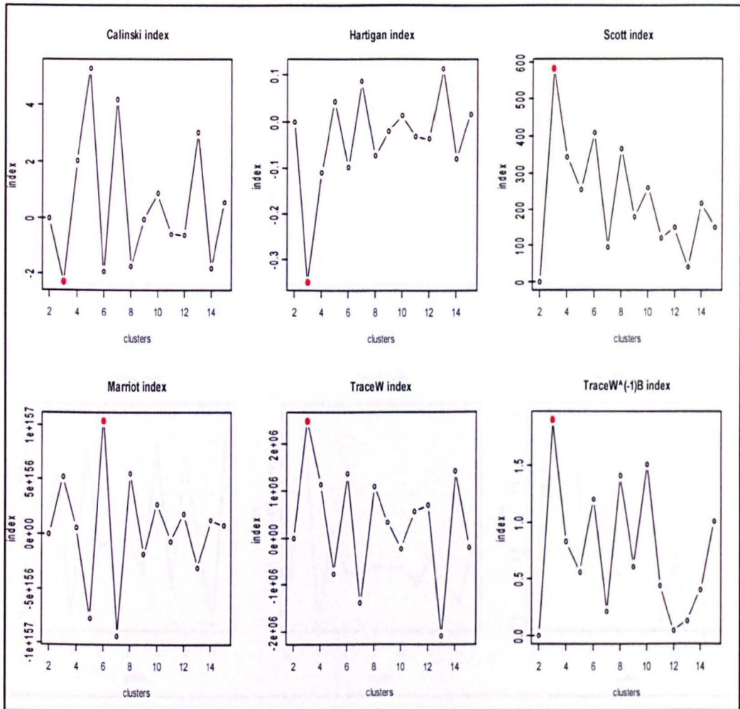
Figure 7.2: Kmeans validity indices
