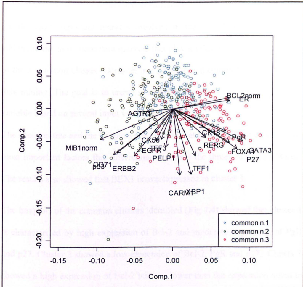
Figure 7.5: Biplots of the 3 common clusters identified using the 25 marker panel.
