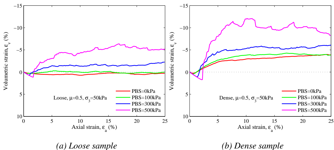
Figure 4.30: Effect of bond strength and axial strain on volumetric strain for both loose and dense samples with particle friction coefficient 0.5 and confining pressure 50kPa
