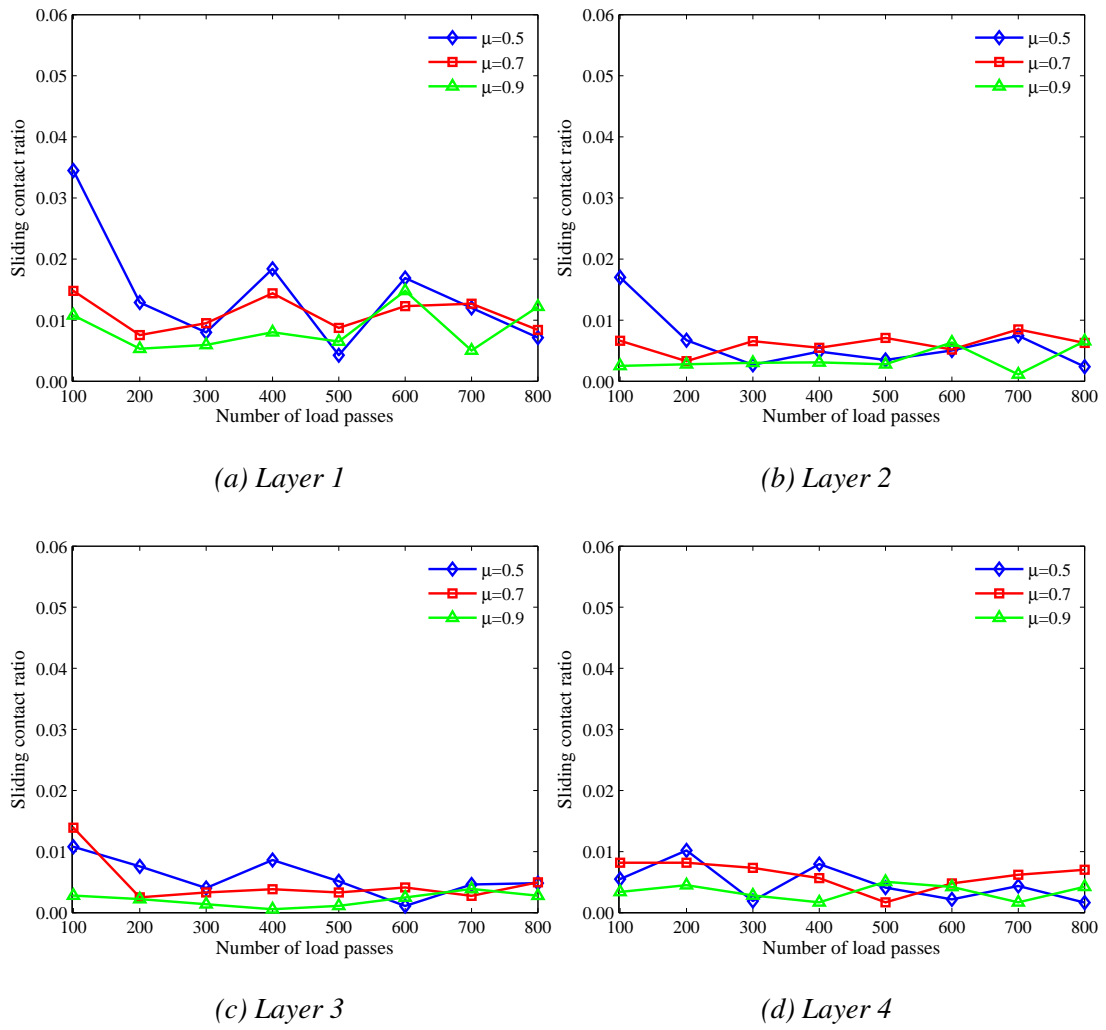
Figure 7.21: Effect of particle friction coefficient on the sliding contact ratio for the unbonded pavement
