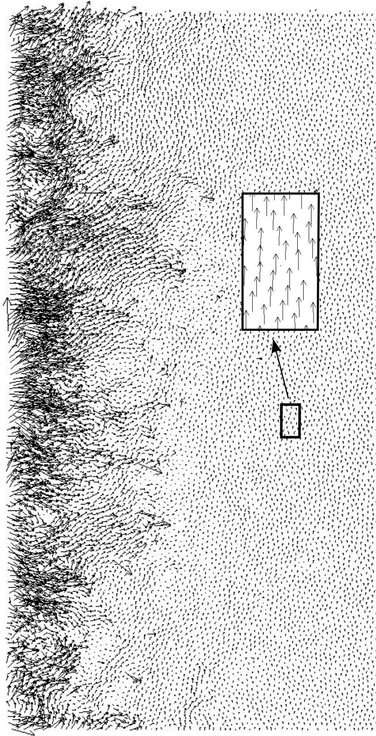
Figure 7.24: Total particle displacement after wheel pass 100 for gravity acceleration of 9.81\text{m/s}^2 and wheel pressure of 7.0\text{kPa} (maximum displacement = 2.41 \times 10^{-2}\text{m} )
