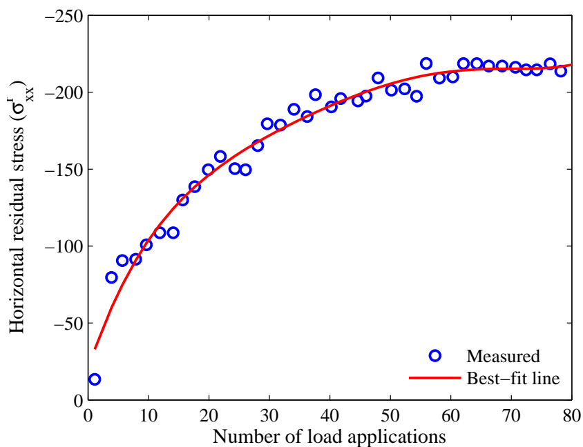
Figure 2.11: Variation of horizontal residual stress ( \sigma_{xx}^r ) with number of load applications (Radovsky and Murashina, 1996)
