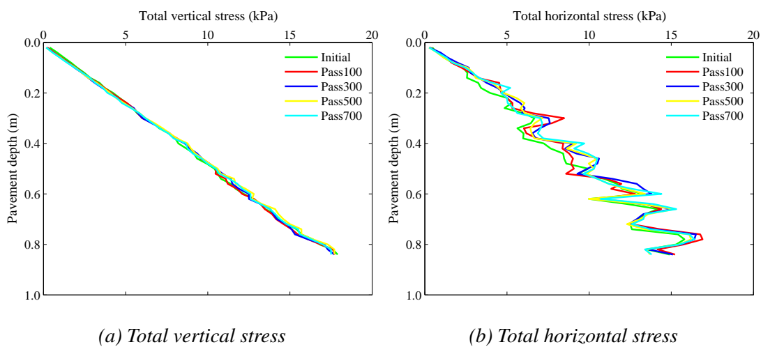
Figure 5.30: The total stress distribution versus pavement depth for gravity acceleration of 9.81m/s^2
