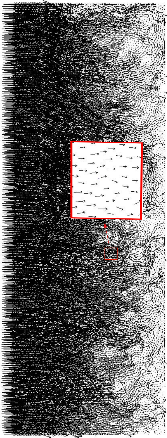
Figure 7.50: Total particle displacement after wheel pass 100 for gravity acceleration of 0.1\text{m/s}^2 and wheel pressure of 10.0\text{kPa} (maximum displacement
