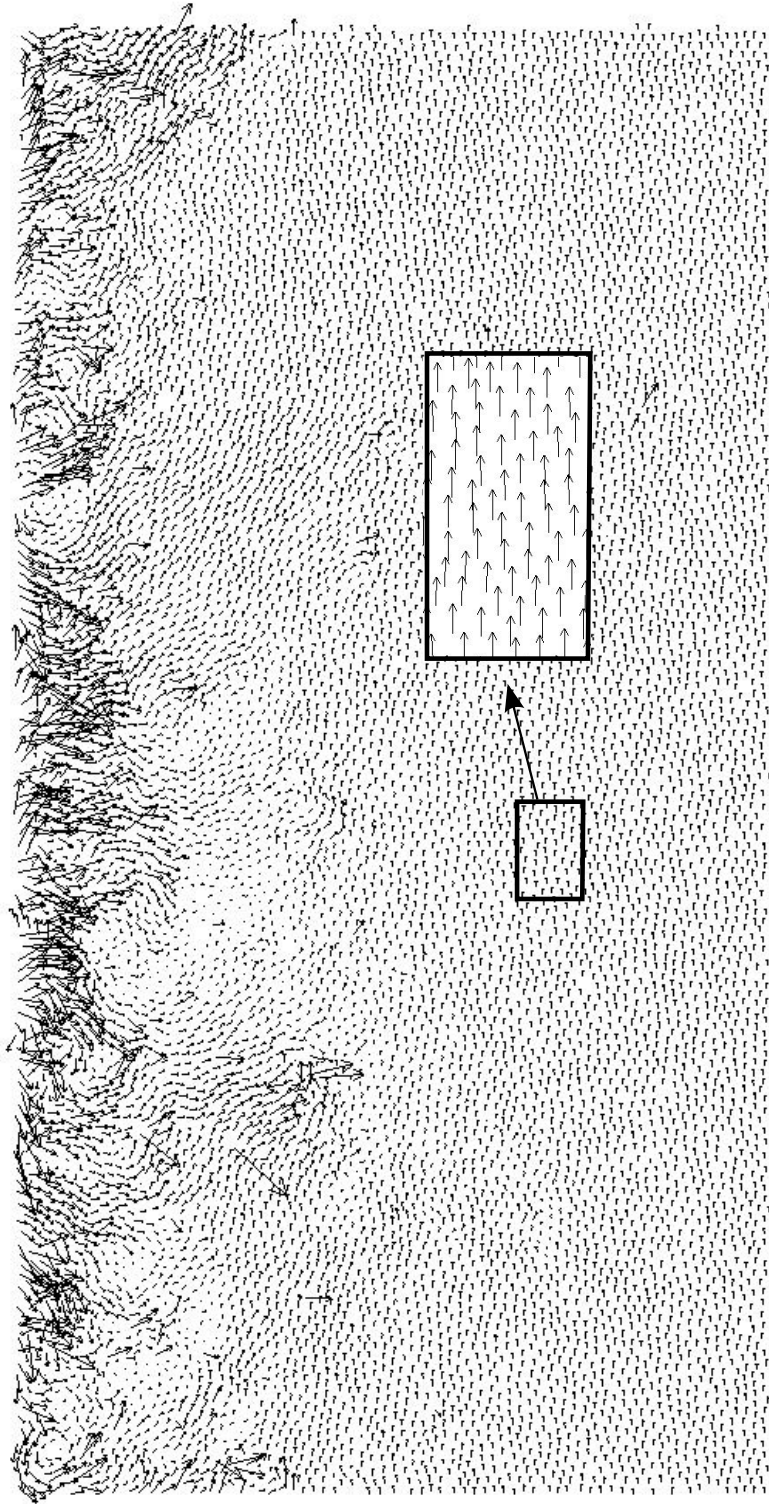
Figure 7.22: Total particle displacement after wheel pass 100 for gravity acceleration of 9.81\text{m/s}^2 and wheel pressure of 2.0\text{kPa} (maximum displacement = 1.43 \times 10^{-2}\text{m} )
