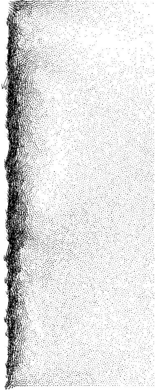
Figure 7.39: Total particle displacement after wheel pass 300 for gravity acceleration of 0.1\text{m/s}^2 and wheel pressure of 169\text{kPa} (maximum displacement = 3.07 \times 10^{-6}\text{m} )
