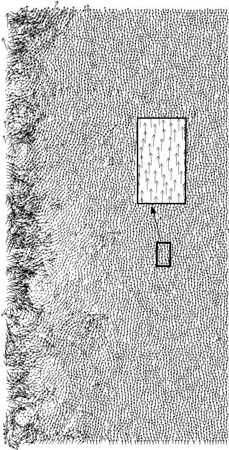
Figure 7.23: Total particle displacement after wheel pass 500 for gravity acceleration of 9.81\text{m/s}^2 and wheel pressure of 2.0\text{kPa} (maximum displacement = 1.39 \times 10^{-2}\text{m} )
