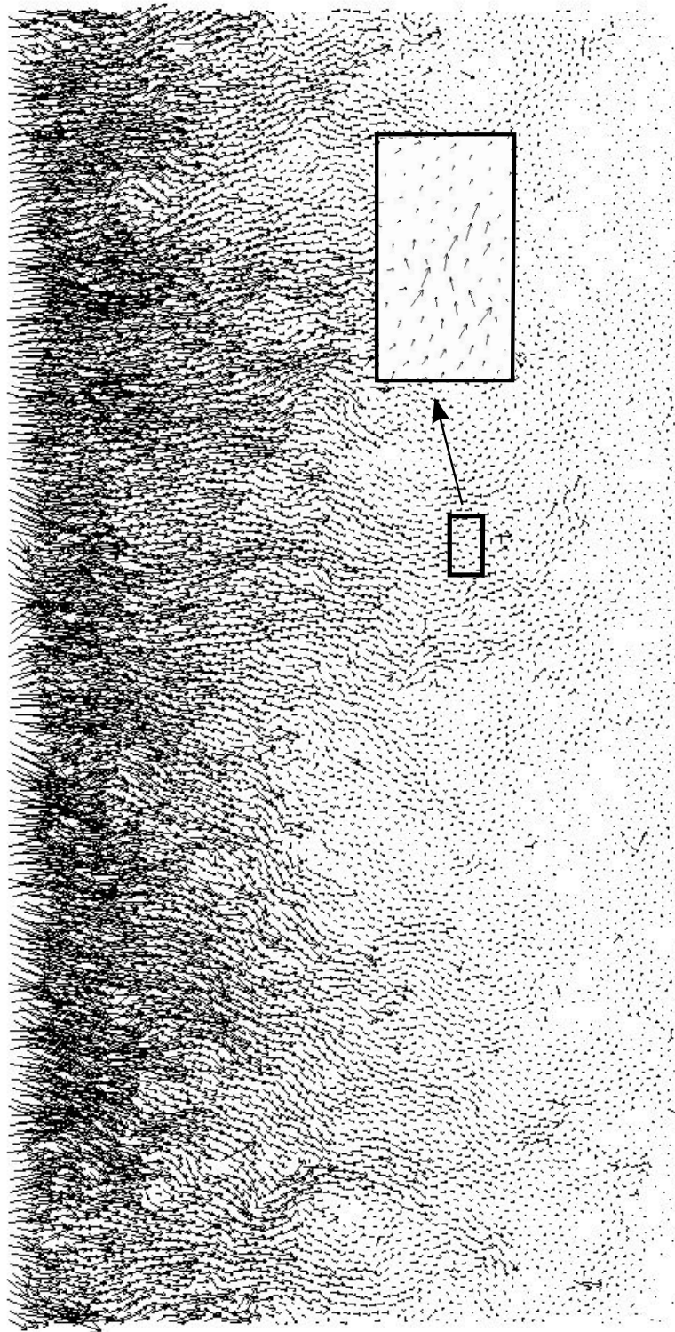
Figure 7.25: Total particle displacement after wheel pass 100 for gravity acceleration of 0.1m/s^2 and wheel pressure of 2.0kPa (maximum displacement = 2.44 \times 10^{-2}m )
