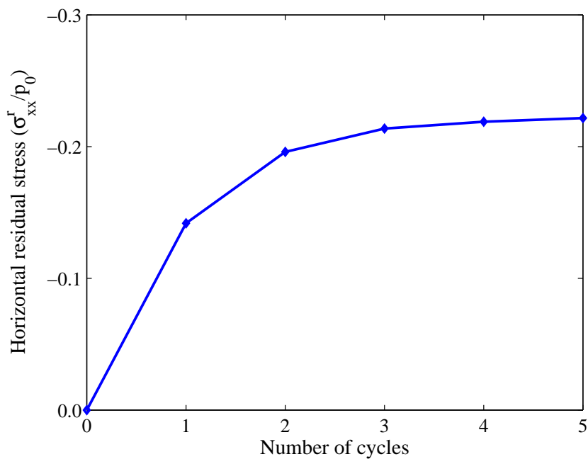
Figure 2.12: Variation of normalised horizontal residual stress ( \sigma_{xx}^r/p_0 ) with number of load applications, where p_0/k = 4.76 , k = 16 \times 10^3 \text{lb/in}^2 (Johnson and Jefferis, 1963)
