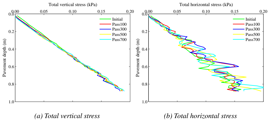
Figure 5.29: The total stress distribution versus pavement depth for gravity acceleration of 0.1m/s^2
