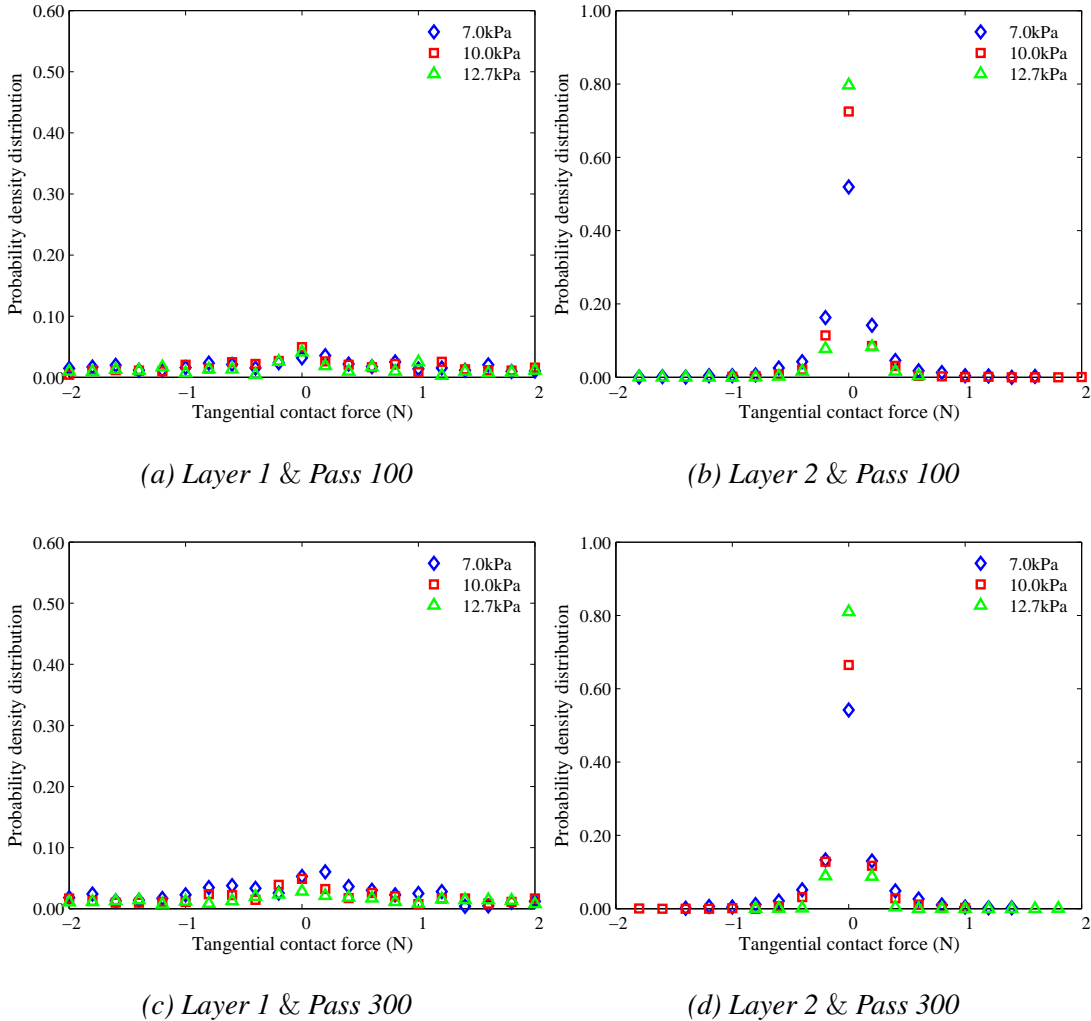
Figure 7.45: Effect of wheel pressure on the probability density distribution of the tangential contact force for the double-layered pavement
