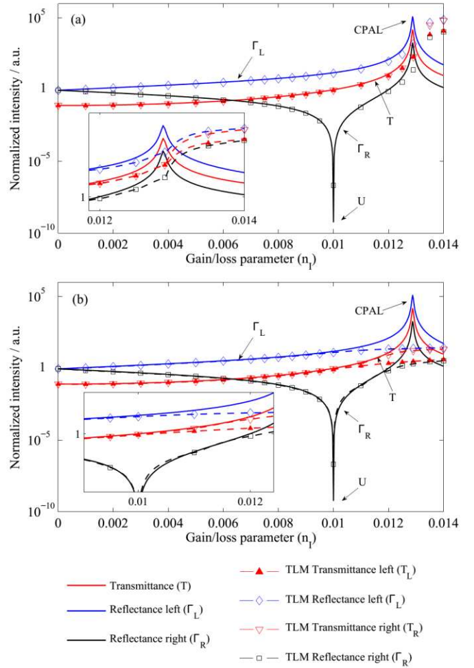
Fig. 3. (Color online) Comparison of the TLM and T-matrix results for the transmitted power from left ( T_L ) and right ( T_R ), power reflected from the left ( \Gamma_L ) and right ( \Gamma_R ) at the Bragg frequency f_B as a function of the gain/loss parameter n_I in structure of 150 number of periods, n_R = 1.55 and \Delta n_R = 0.01 for 2 different amplitudes of the input of CW signal (a) E_m = 0.002 E_{sat} and (b) E_m = 0.2 E_{sat}
