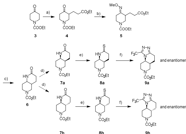
Scheme 1. Synthetic route to compounds 9a and 9b . a
