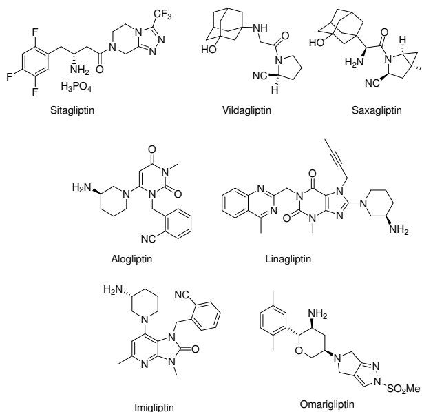
Figure 1. Approved DPP-4 inhibitors: sitagliptin, vildagliptin, saxagliptin, alogliptin, linagliptin and the clinical candidates imigliptin and omarigliptin,
