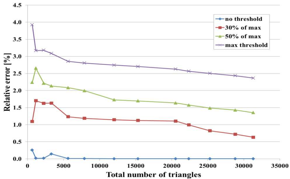
Figure 4.20: Relative error \left| \frac{f_{\text{TLM}} - f_a}{f_a} \right| for the fundamental resonance TM01 of PEC cylindrical resonator of radius 1cm concentrically loaded with a dielectric cylinder of relative permittivity \epsilon_r=2.1 and 0.5cm radius as a function of different mesh sizes.
