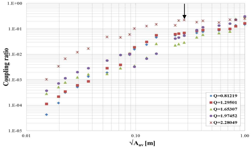
Figure 5.29: Coupling ratio of the excited mode n=0 with mode n=2 as function mesh parameter \sqrt{A_{av}} (m) and for different mesh quality factor Q . Arrow points to mesh with \sqrt{A_{av}} / \lambda_o < 0.1 .
