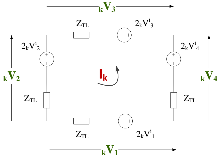
Figure 2.11: Thevenin equivalent circuit of the TLM series node
