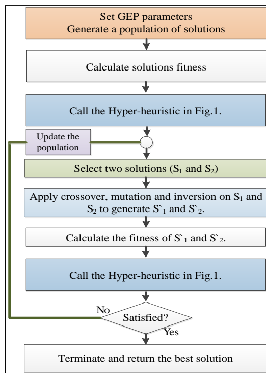
Fig. 6. The proposed hyper-heuristic
