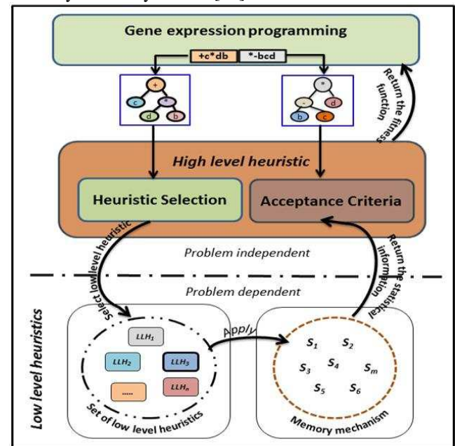
Fig. 1. The proposed gene expression programming based hyper-heuristic (GEP-HH) framework.
