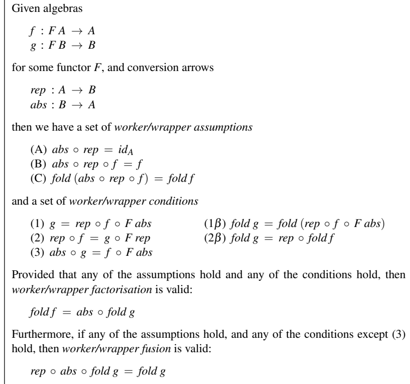
Figure 2: Worker/wrapper transformation for initial algebras.
