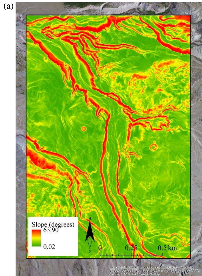
Figure 4.6 Slope maps of the upper analysis reach (see Figure 4.3 for location) derived from the 3 m (a) and 50 m (b) DEMs. Aerial imagery from DigitalGlobe (Microsoft).
