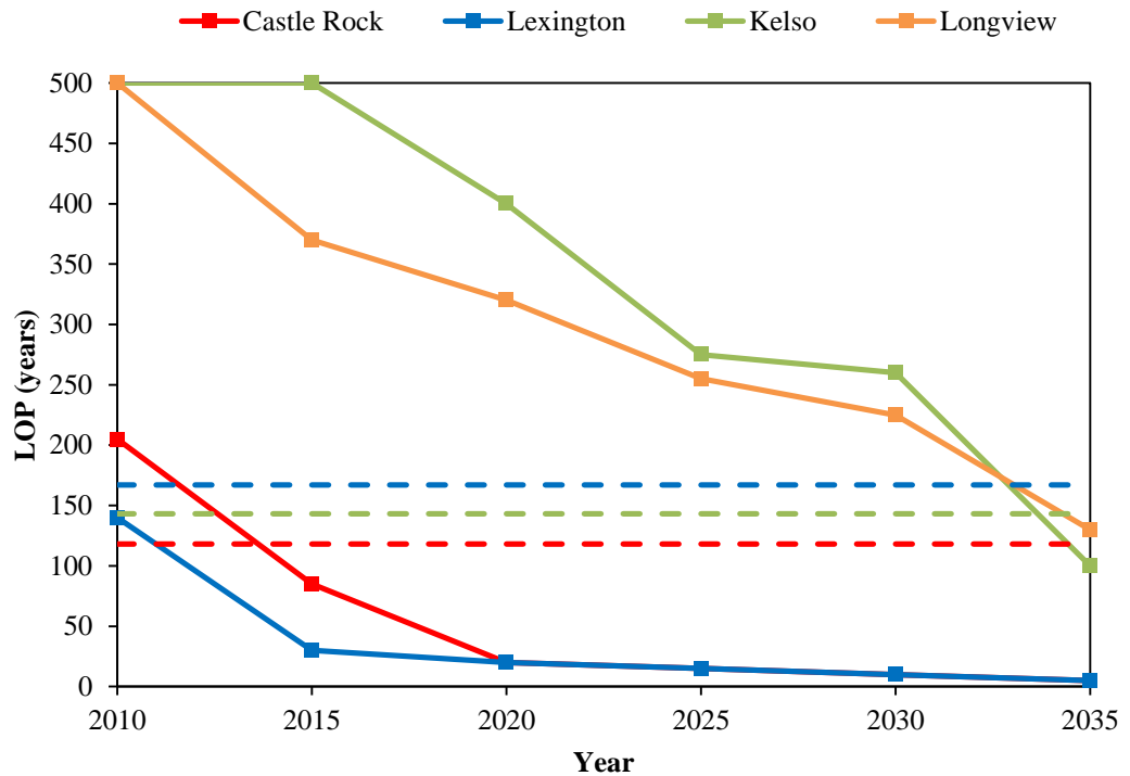
Figure 2.17 Probabilistic forecasts of LoPs at authorized communities on the Cowlitz River. Red, green and blue dashed lines represent the 118, 143 and 167 year authorized LoPs respectively. Adapted from USACE (2012, p. 4).
