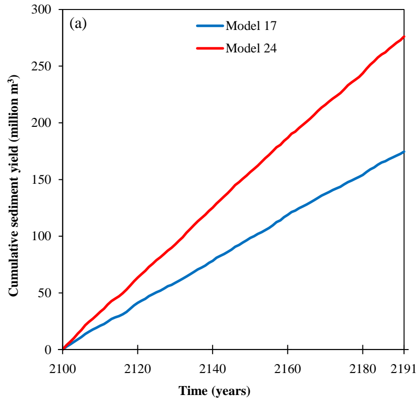
Figure 6.24 (a) cumulative sediment yields for Models 17 and 24; (b) and (c) residuals calculated between the modelled erosion volumes and those predicted by a straight line for Models 17 and 24 respectively; (d) and (e) sediment yield per unit volume of discharge for Models 17 and 24 respectively.
