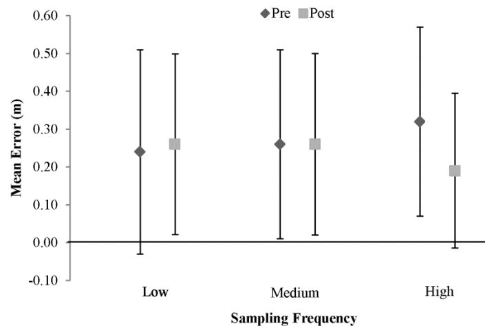
Figure 3: Plot of mean static error for each sampling frequency during pre and post session. Error bars represent standard deviation.
