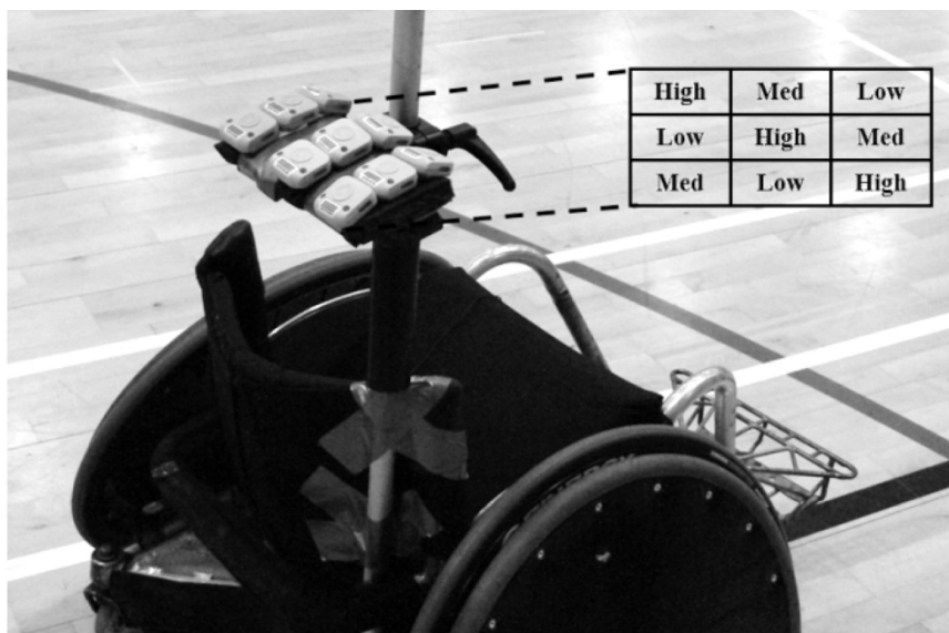
Figure 1: The location of the nine tags fixed to the wheelchair during dynamic tests. Inset is the sampling frequency for each tag with regards to its location
