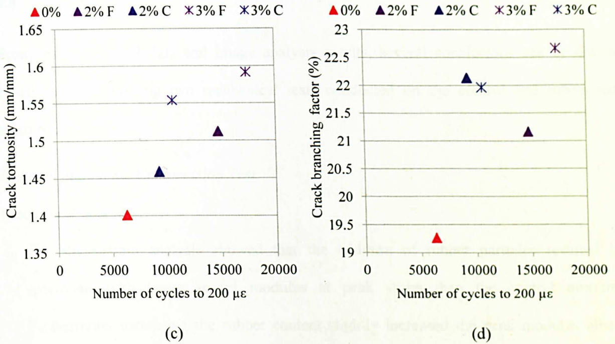
Figure 7.43 Fracture surface parameters vs number of cycles at 100 \mu\epsilon
