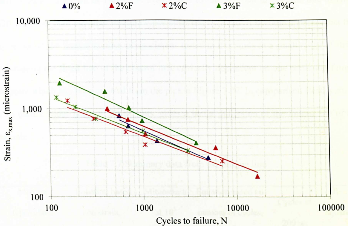
Figure 7.20 Fatigue lines for unmodified and rubberised mixtures tested at 20°C
