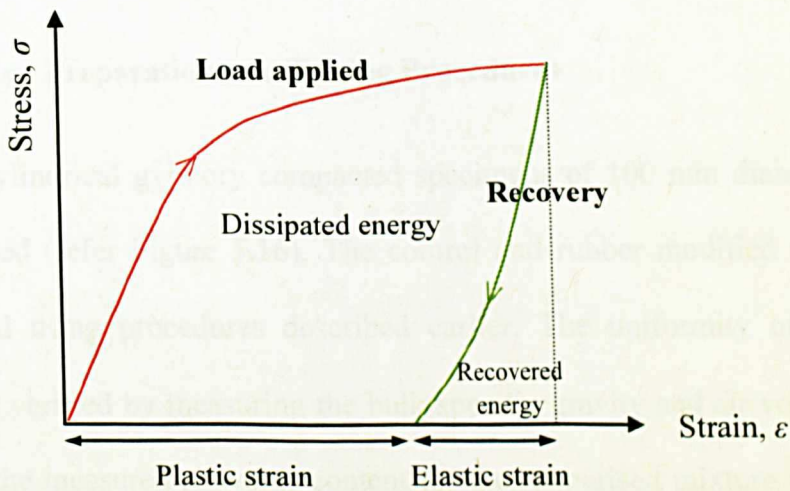
Figure 5.15 Typical of load and unload behaviour in a stress-strain curve
