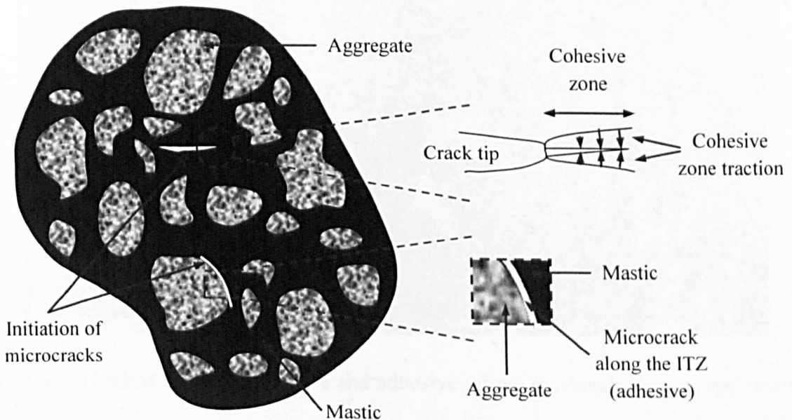
Figure 7.10 Microcracks initiation via cohesive and adhesive failure (inspired from Kim et al., 2007)
