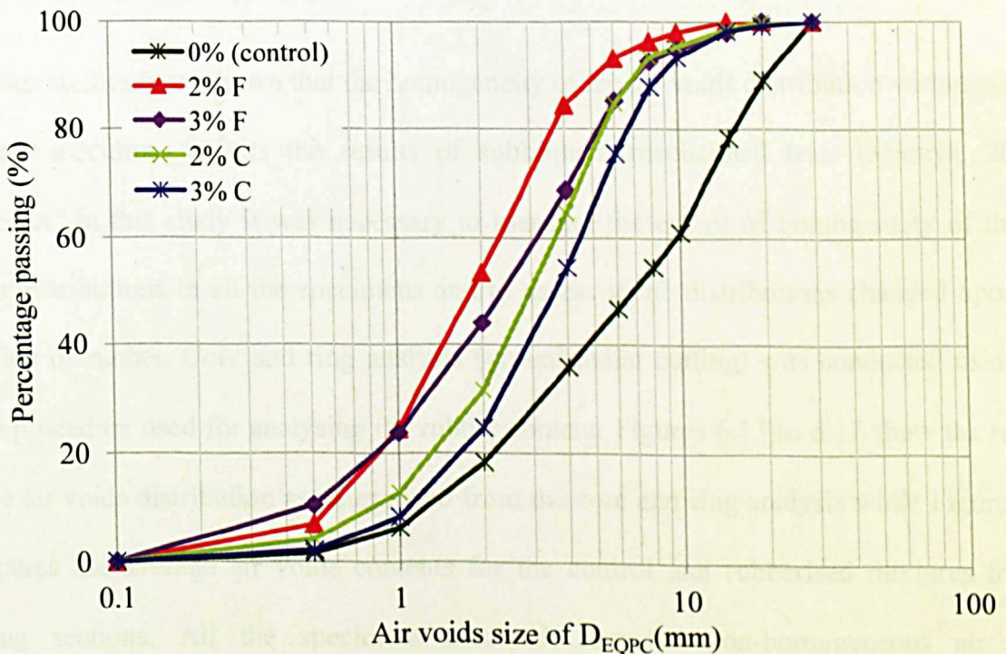
Figure 6.12 Air voids size gradation for different mixtures
