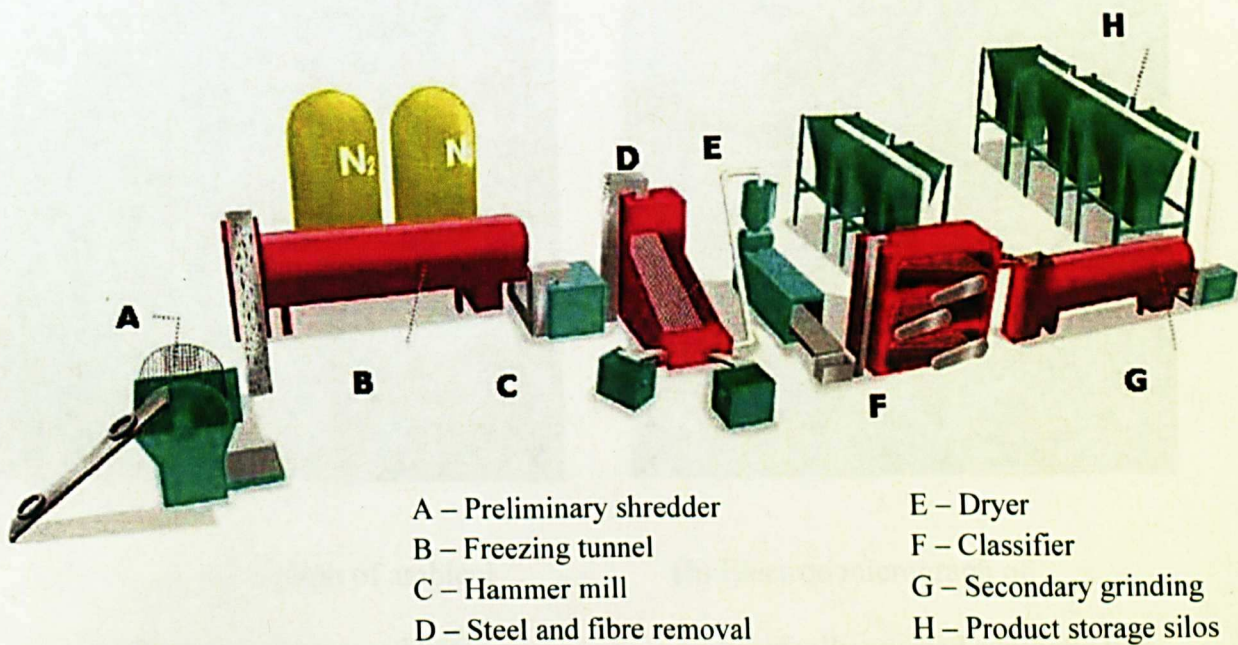
Figure 2.5 Schematic of a cryogenic grinding for scrap tyre recycling system (Reschner 2006)
