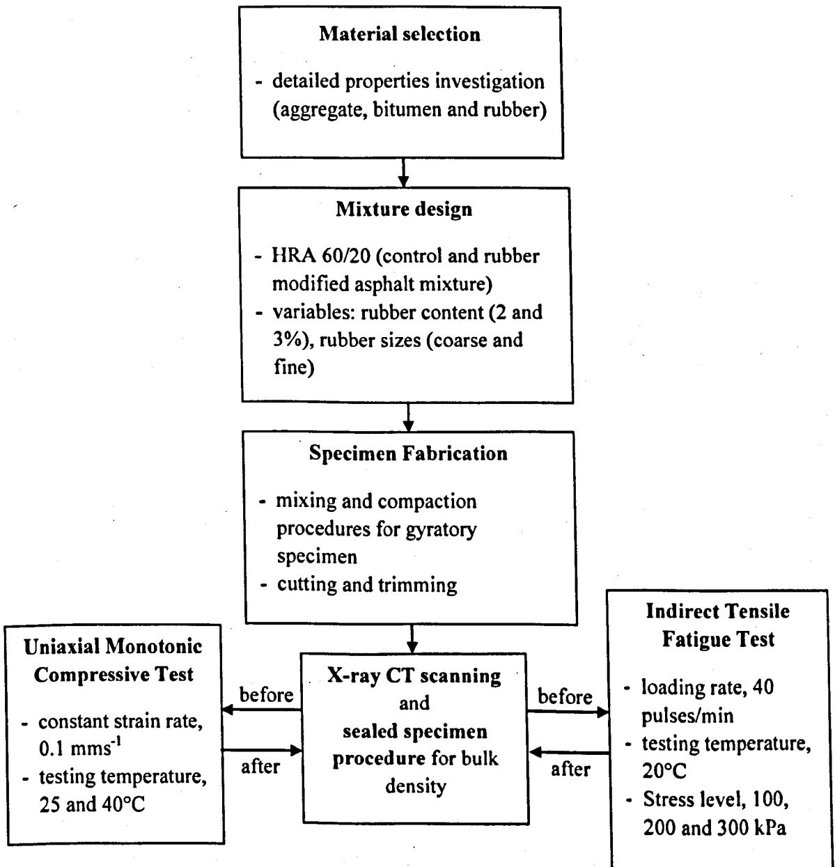
Figure 5.1 Experimental programme
