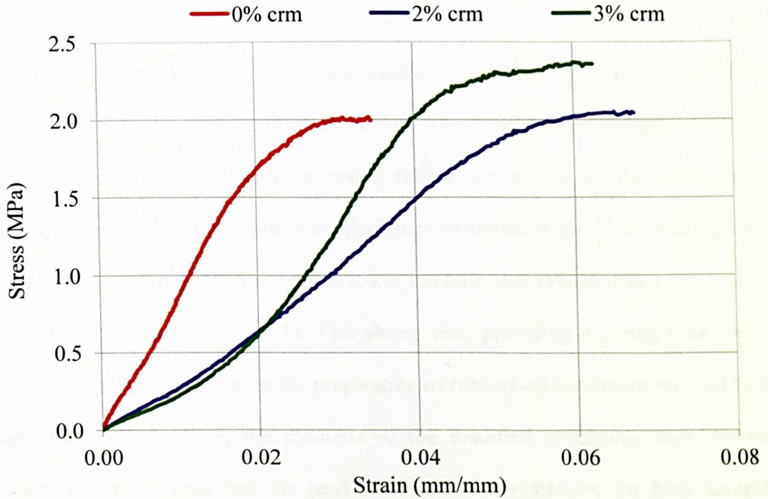
Figure 7.2 Stress-strain plots of specimens subjected to Uniaxial Monotonic Compression at 25°C
