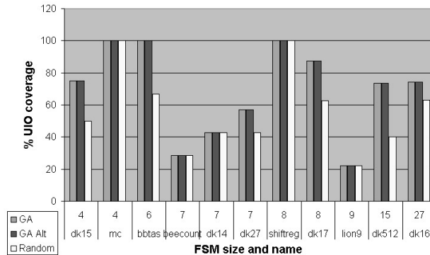
Figure 3.6: Percentage state coverage in UIOs generated by GA compared to random algorithm. Results for real FSMs
