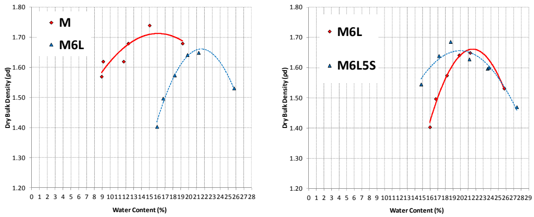
Figure A 13: OWC of soil mixture M, M6L and M6L5S (BS1377-2: 1990)
