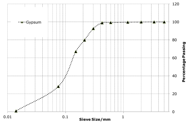
Figure A 7: Particle Size Distribution (PSD) of gypsum (BS1377-2: 1990)
