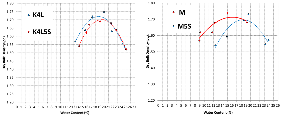
Figure A 12: OWC of soil mixture K4L, K4L5S, M and M5S (BS1377-2: 1990)
