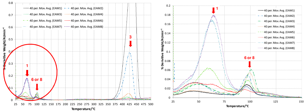
Figure 84: dTGA analysis of M6L5S early age study specimens (EAM1-8). 1 - desorption \text{H}_2\text{O} , 3 – \text{Ca}(\text{OH})_2 , 6 – ettringite (AFt), 8 – \text{CaSO}_4 \cdot 2\text{H}_2\text{O}
