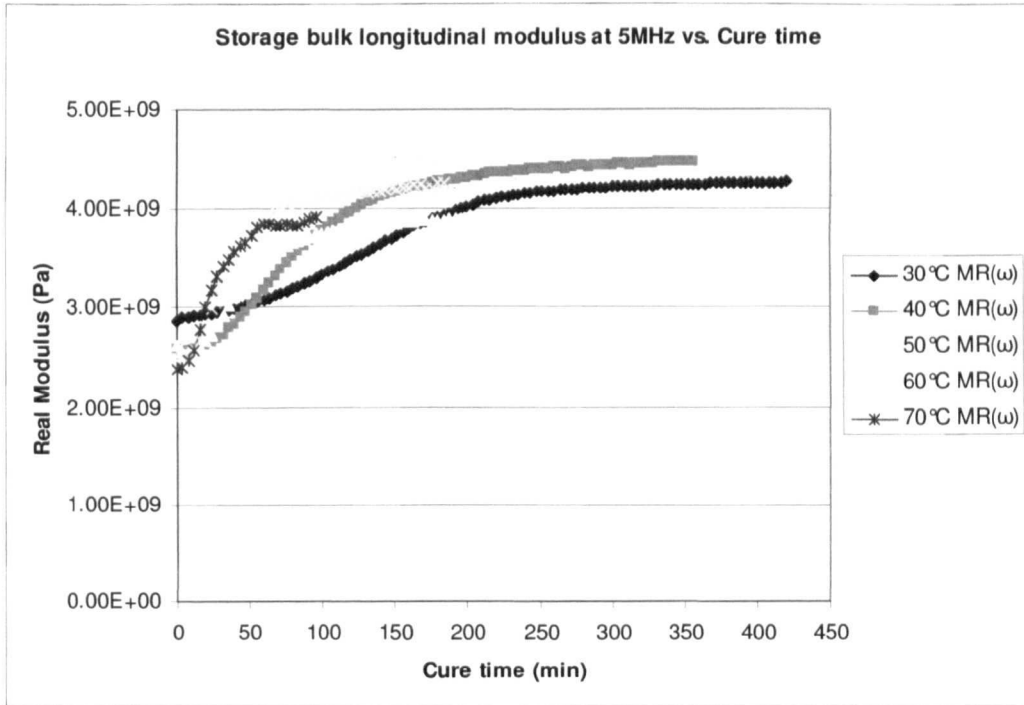
Figure 9.3 Real part of Ultrasonic Compression wave modulus at 5MHz as a function of cure time at cure temperatures of 30°C, 40°C, 50°C, 60°C, and 70°C.
