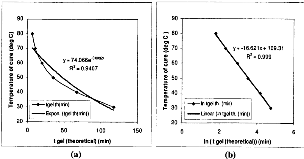
Figure 5.12 (a,b) Theoretical gel time obtained from calorimetric study as a function of isothermal cure temperature for isothermal cure process of Araldite 2015.
