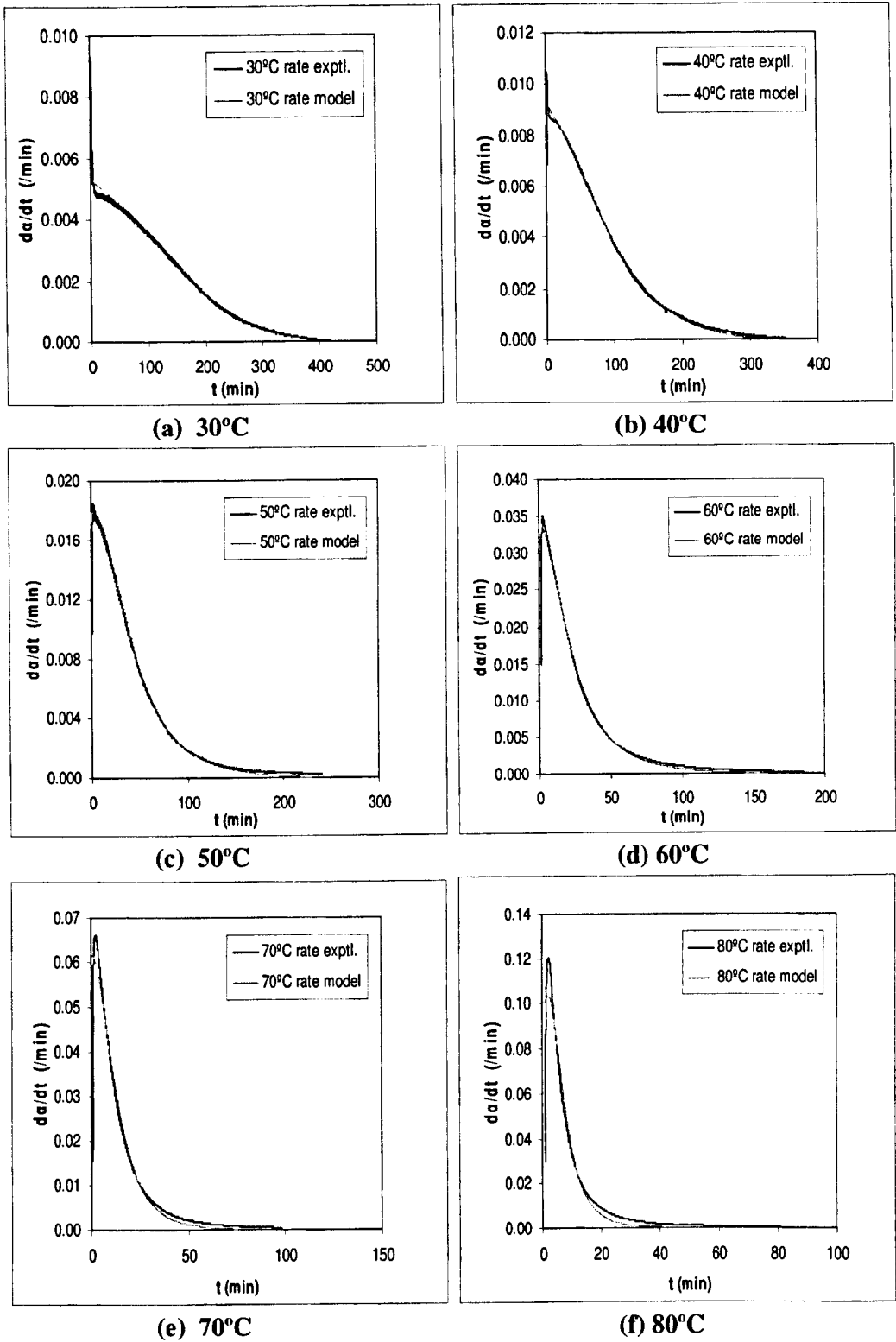
Figure 6.25(a—f) Isothermal reaction rates as a function of cure time — comparisons of experimental data with the predictions of Autocatalytic kinetic model da/dt = k(\alpha_{\max} - \alpha)^n e^{m\alpha} at cure temperatures of : (a) 30°C, (b) 40°C, (c) 50°C, (d) 60°C, (e) 70°C and (f) 80°C.
