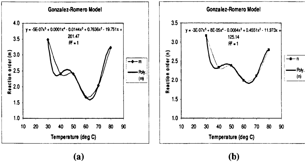
Figure 6.34 The plots showing the effect of the isothermal cure temperature on the reaction orders (a) m and (b) n with associated fits; based on the Autocatalytic kinetic model d\alpha/dt = k(1-\alpha)^n e^{m\alpha} for isothermal cure process of Araldite 2015.
