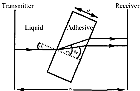
Figure 8.1 Excitation of compression and shear waves in a slab sample immersed in a liquid between an ultrasonic transmitter and receiver.
