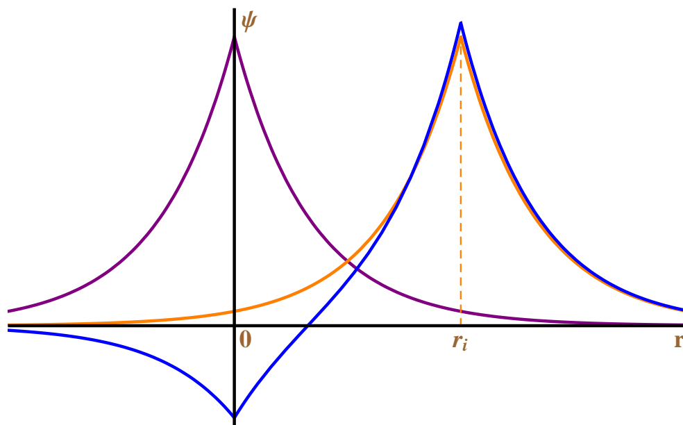
Figure 3.1: Orthogonalised and unorthogonalised states for two interacting s -type Slater orbitals separated by a distance r_i . The wavefunction of the first electron is in purple and remains unchanged, while the unorthogonalised state of the second electron is in orange, and the orthogonalised state is in blue.
