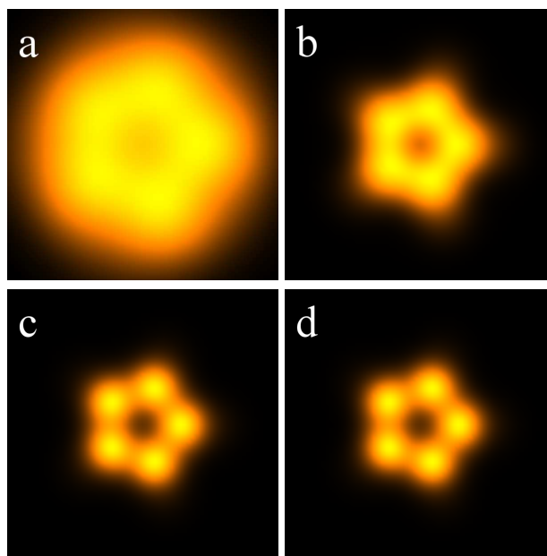
Figure 7.4: Theoretical scans of the repulsive force observed when a C_{60} adsorbed with a pentagonal face prone to the surface interacts with a tip state described by a normalised Gaussian of varying decay rate. The exponents of the Gaussians are (a) -0.1, (b) -1, (c) -10, (d) -100.
