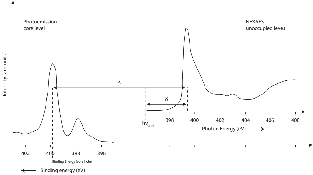
Figure 3.11: Schematic figure to illustrate how a NEXAFS spectrum is converted into a binding energy scale.
