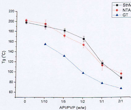
Figure 3.12: Comparisons T_g from SThM, NTA and the Gordon-Taylor's equation for Felodipine-PVP mixtures.
