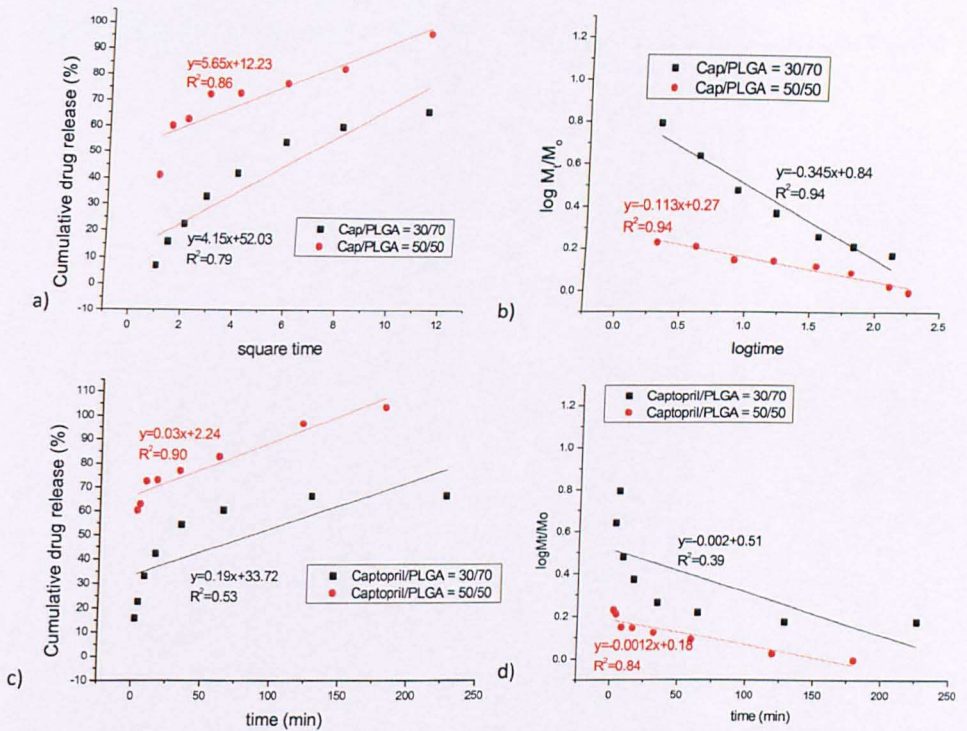
Figure 6.24: a) Higuchi, b) Korsmeyer-Peppas c) zero order, d) first order for mechanism of drug release for the mixtures Captopril/PLGA at ratio of 30/70, and 50/50 prepared by pipetting deposition.
