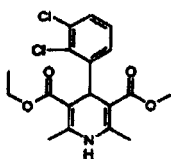
Figure 3.1: Felodipine
