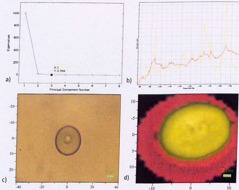
Figure 3.30: a) Eigenvalues plot versus PCs numbers of the Felodipine/PVP = 1/5 mixture b) 2 model spectra used to create the chemical map, where the red, and the yellow correspond to background, and the sample respectively c) optical microscope image of deposited product d) Chemical image of the mixture.
