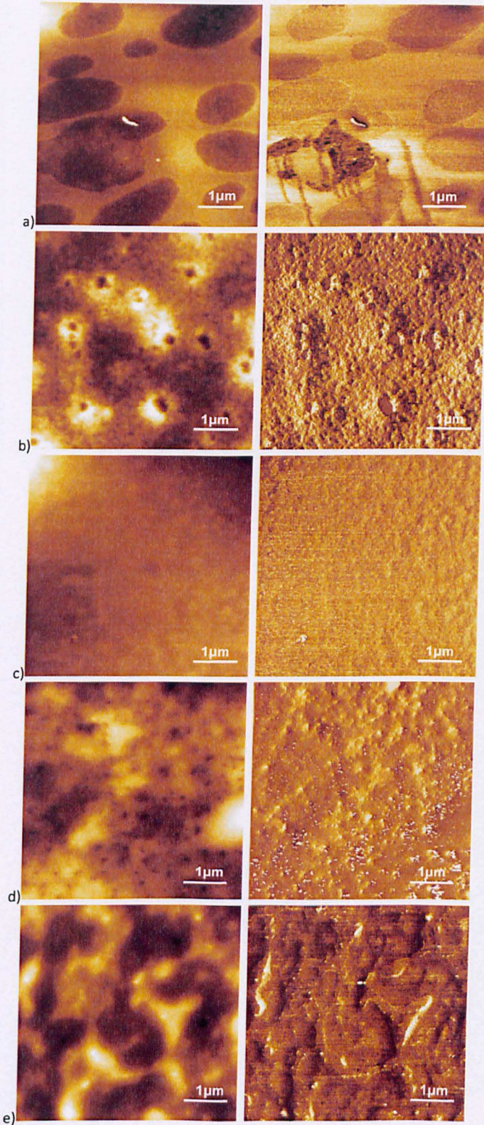
Figure 4.6: Topographic [152] and phase (right) AFM images of 1/5 felodipine/PVP mixture a) before the dissolution in water and after the dissolution for b) 3sec, c) 10sec, d) 15sec, e) 20sec.
