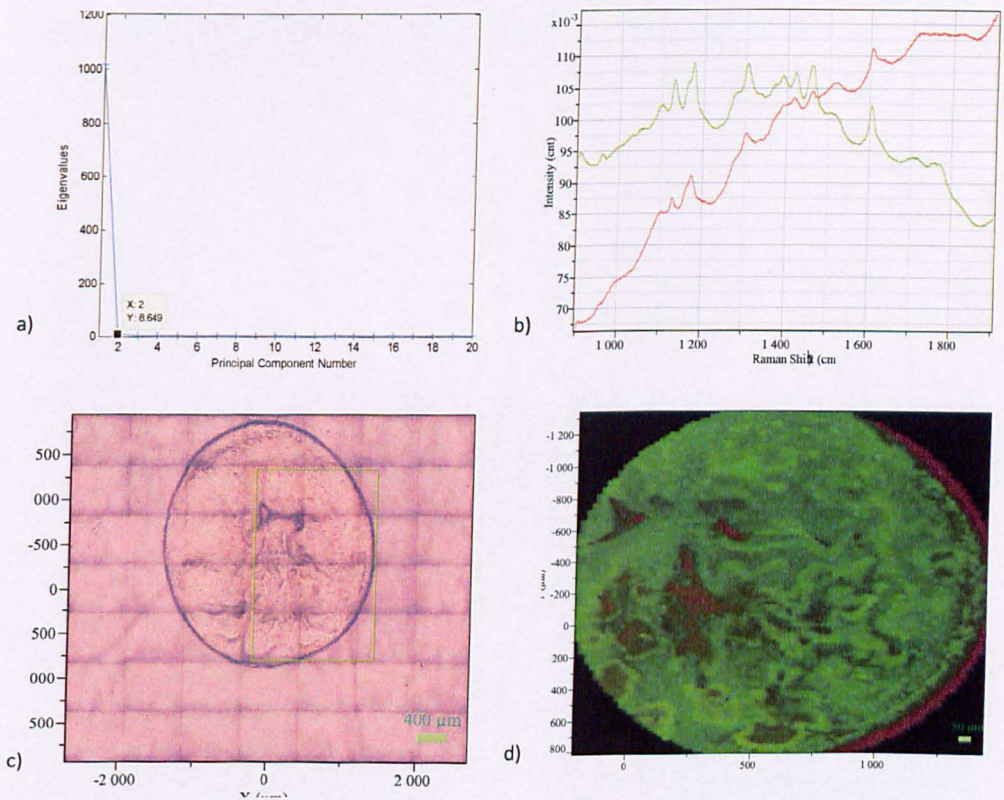
Figure 6.12: Eigenvalues plot versus PCs numbers of the HCT/PLGA/pluronic = 20/75/5 mixture produced by the microarray printer b) 3 model spectra used to create the chemical map, c) optical microscope image of deposited product d) Chemical image of the mixture.
