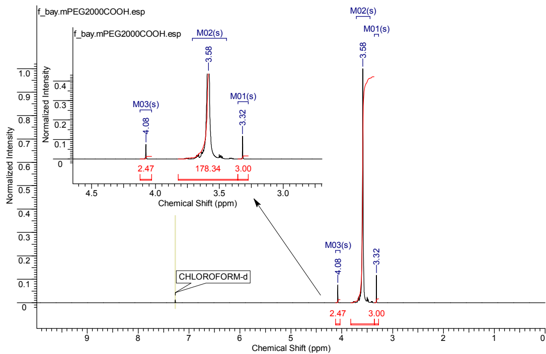
Fig. VI.7. ^1\text{H} NMR for mPEG 2000 COOH Spectrum acquired on a Bruker AV(III)400 spectrometer, 64 scans, in \text{CDCl}_3
