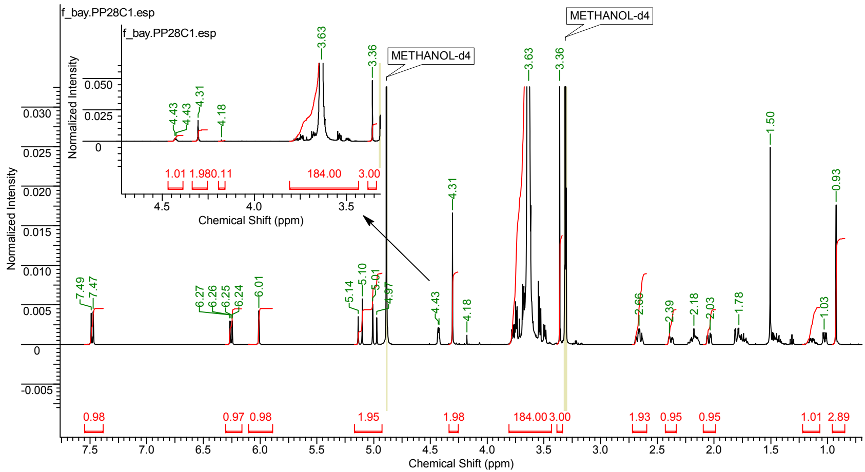
Fig.II.30. 1 H NMR of purified PP28C1 Spectrum acquired on a Bruker AV(III)500, 16 scans, in MeOD
