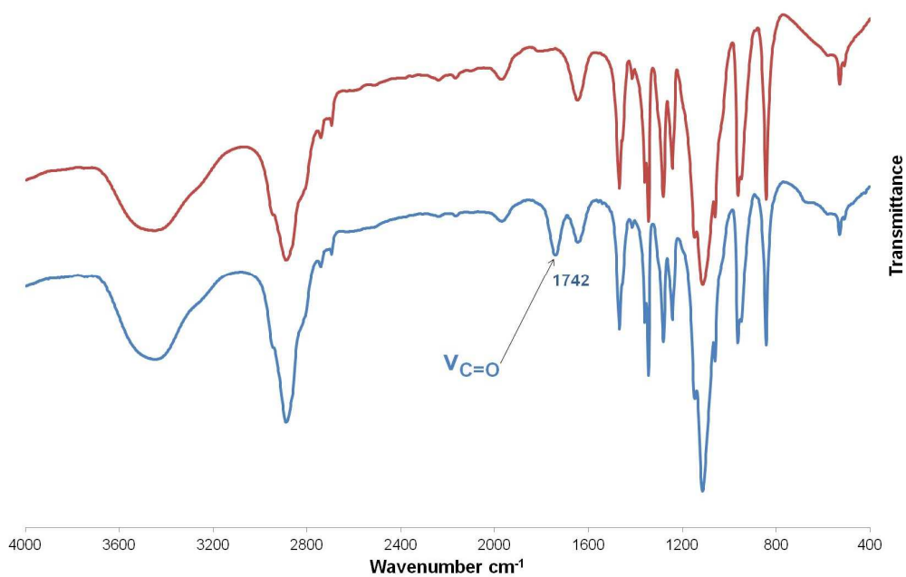
Fig.VI.6. IR spectra for mPEG 2000 and mPEG 2000 COOH
