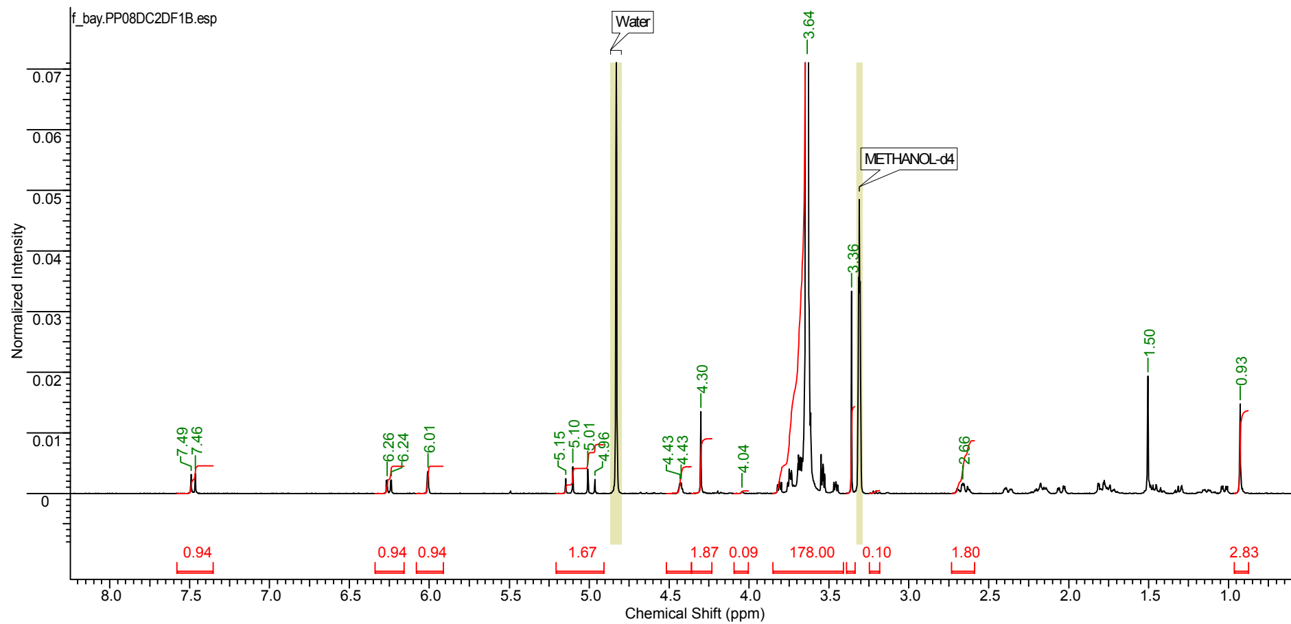
Fig. VI.15. 1 H NMR of PP08DC2DF1B Spectrum acquired on a Bruker AV(III)400 spectrometer, 64 scans, in MeOD
