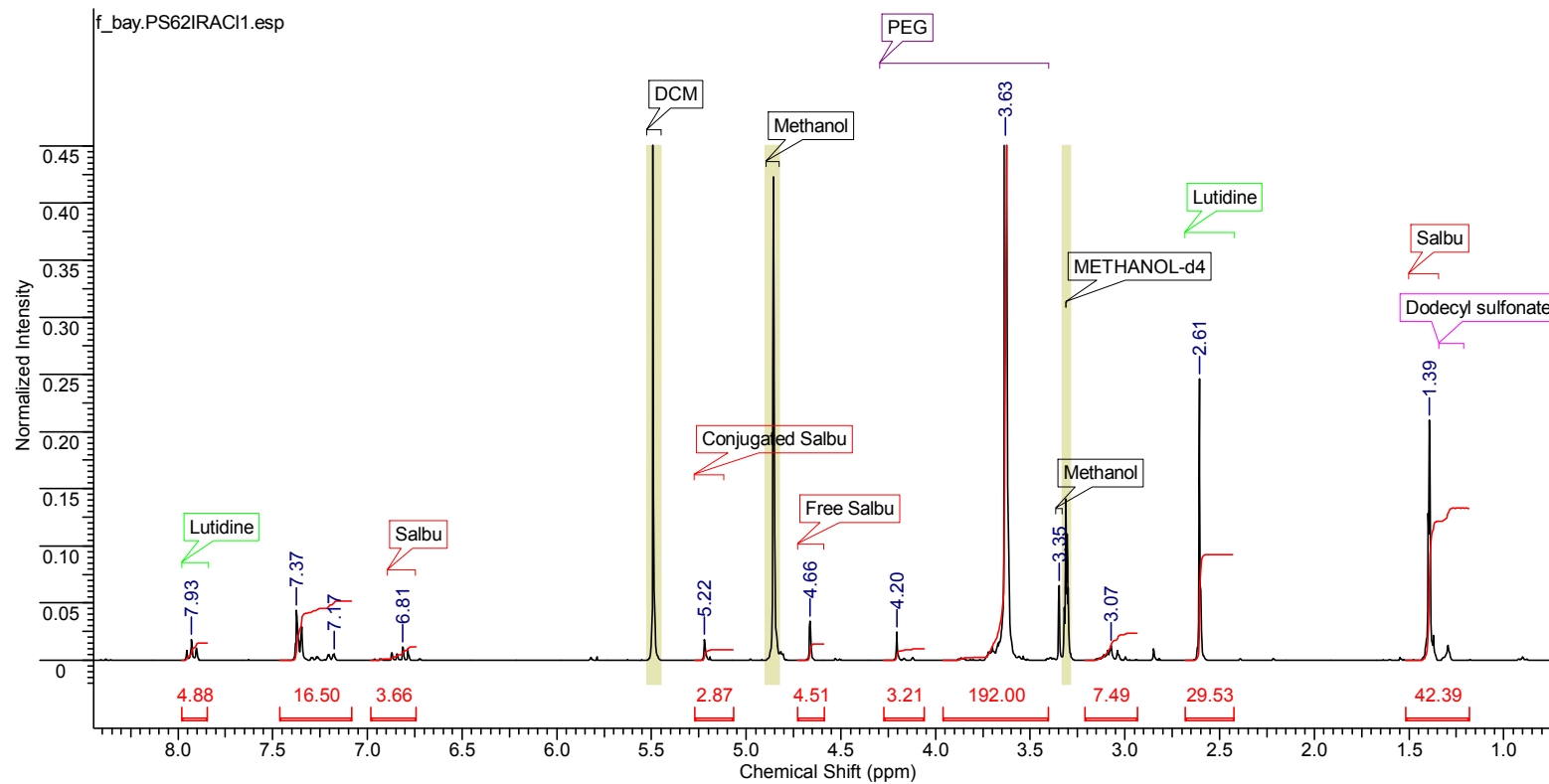
Fig. VI.45. 1 H NMR of PS62IRAC11 Spectrum acquired on a Bruker DPX 300 spectrometer, 16 scans, in MeOD
