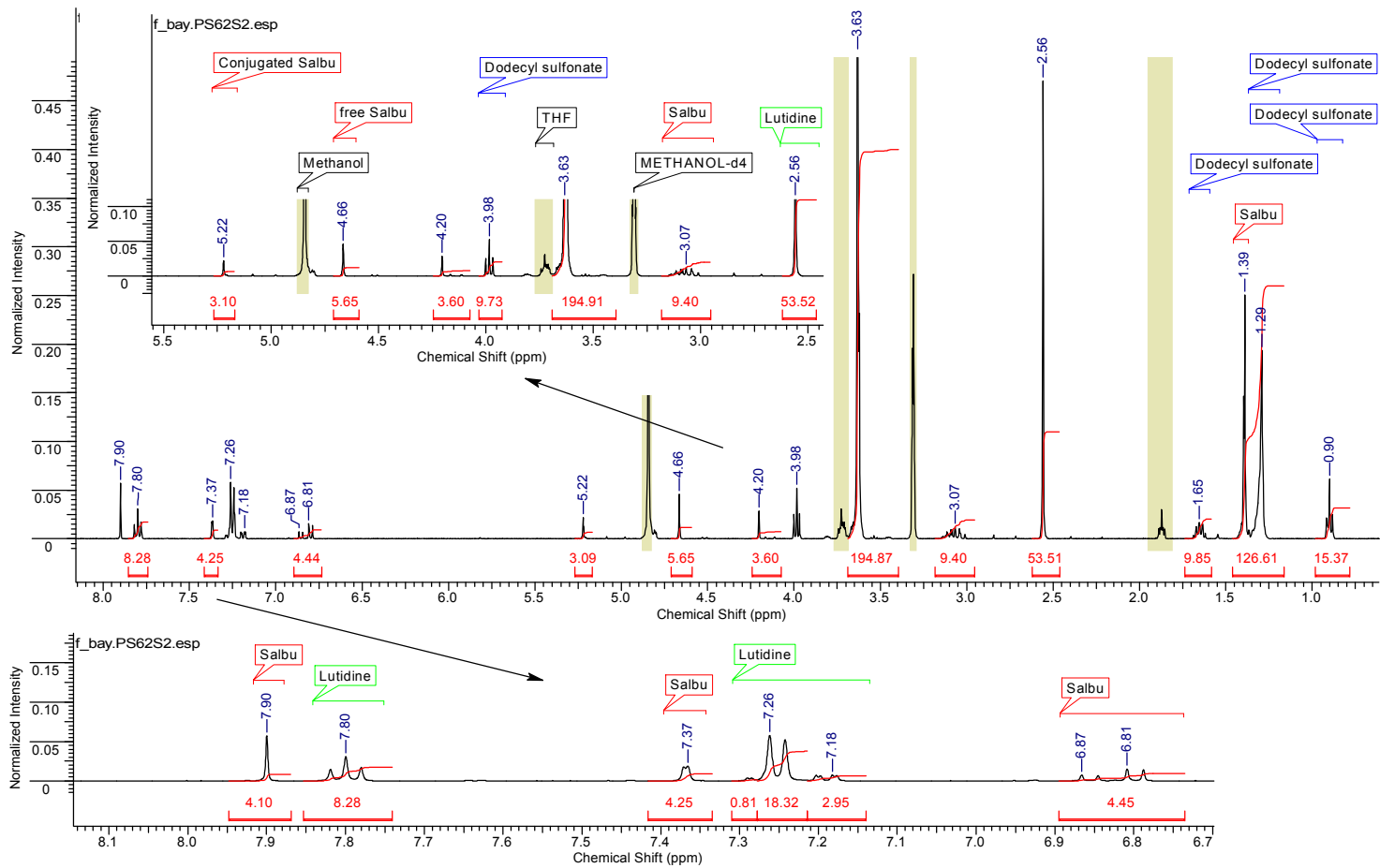
Fig. VI.44. 1 H NMR of PS62S2 Spectrum acquired on a Bruker AV(III)400 spectrometer, 16 scans, in MeOD
