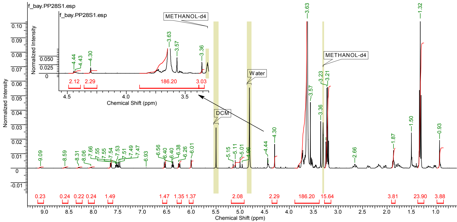
Fig.VI.34. 1 H NMR for the crude PP28S1 Spectrum acquired on a Bruker AV(III)400 spectrometer, 64 scans, in MeOD
