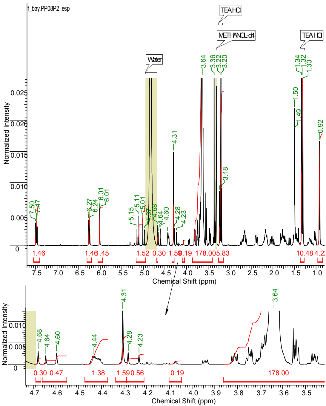
Fig. VI.13. 1 H NMR of crude PP08P2 Spectrum acquired on a Bruker AV(III)400 spectrometer, 64 scans, in MeOD
