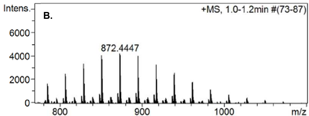
Fig.VI.36. Mass spectrometry analyses of A. PEG 1000 COOH 2 and B. PP33w3 (PEG 1000 -Pred 2 )
