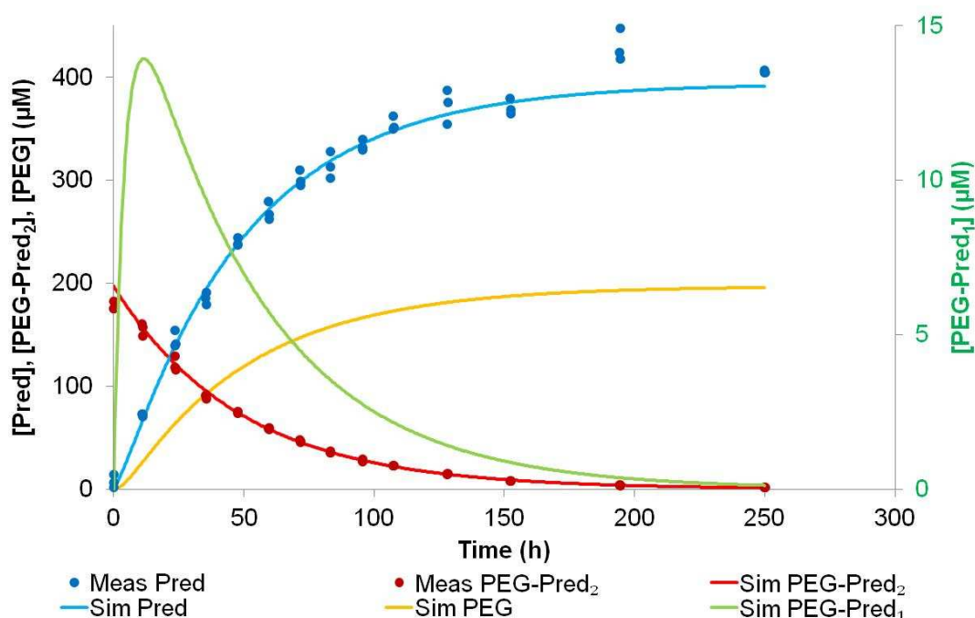
Fig.III.9. Simulation for PP29 hydrolysis at pH 6.2 Meas: Measured values, Sim: Simulated values obtained after solving the system differential equation (III.7) using Berkeley Madonna software. Calculated k_1 = 0.020455 \text{ h}^{-1} , k_2 = 0.228221 \text{ h}^{-1} , initial PEG 2000 -Pred 2 = 197 \mu M.
