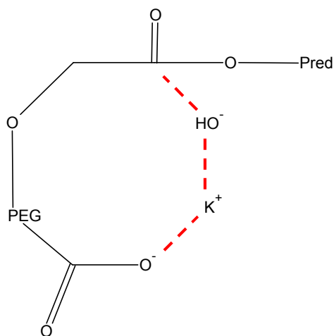
Fig.III.13. Chelate complex for {}^{-}\text{OOC-PEG-Pred}_1 hydrolysis in buffer
