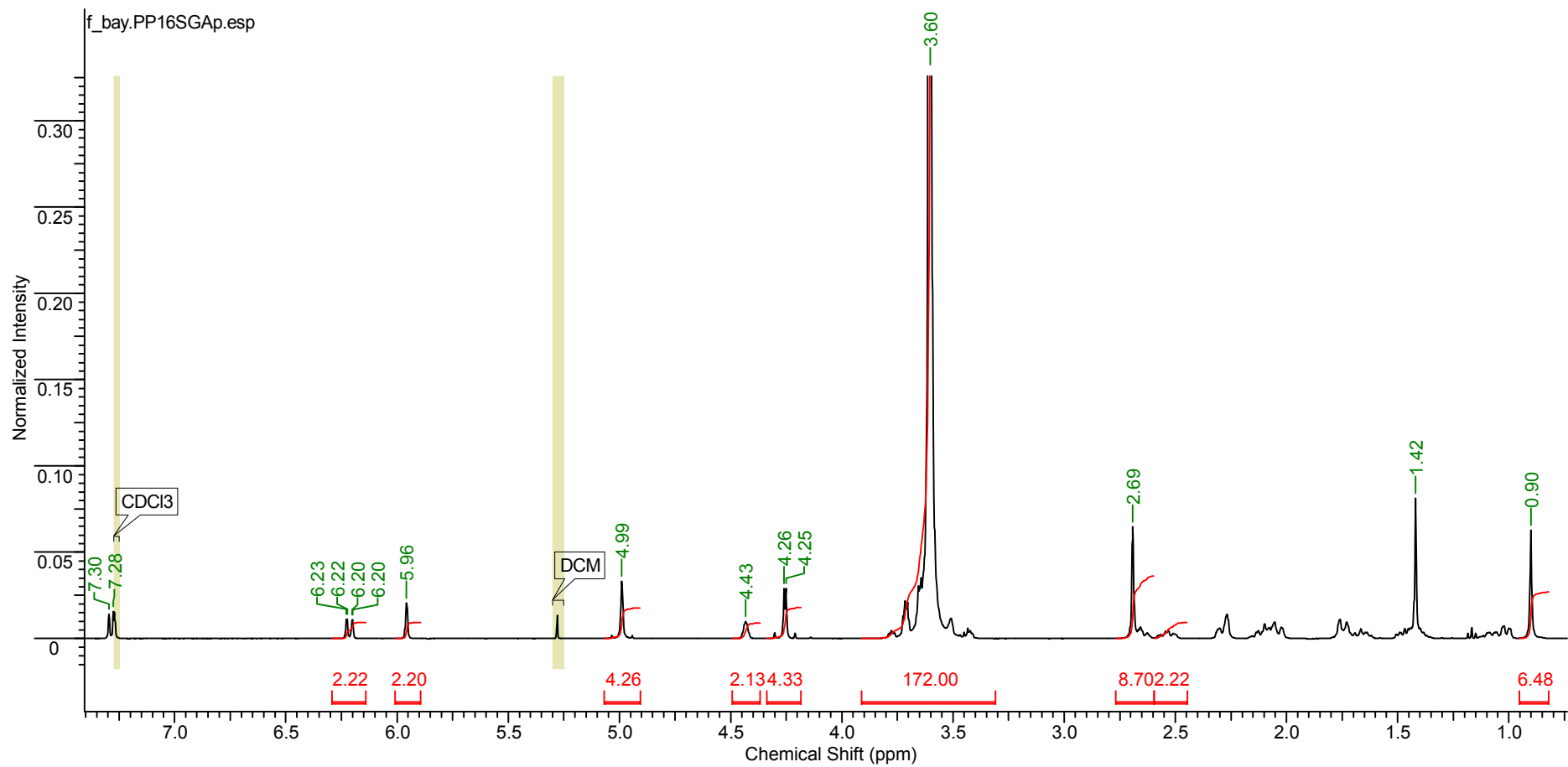
Fig.VI.18. ^1\text{H} NMR of PP16SGAp Spectrum acquired on a Bruker AV(III)400 spectrometer, 64 scans, in \text{CDCl}_3
