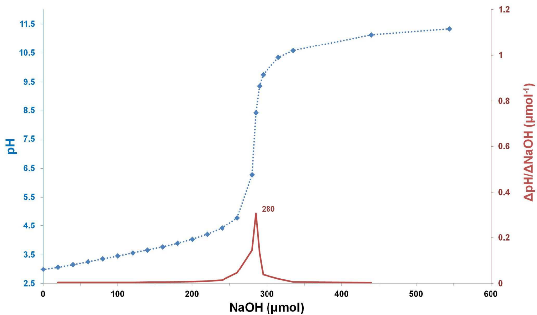
Fig.VI.5. Acid titration for PEG 2000 COOH
