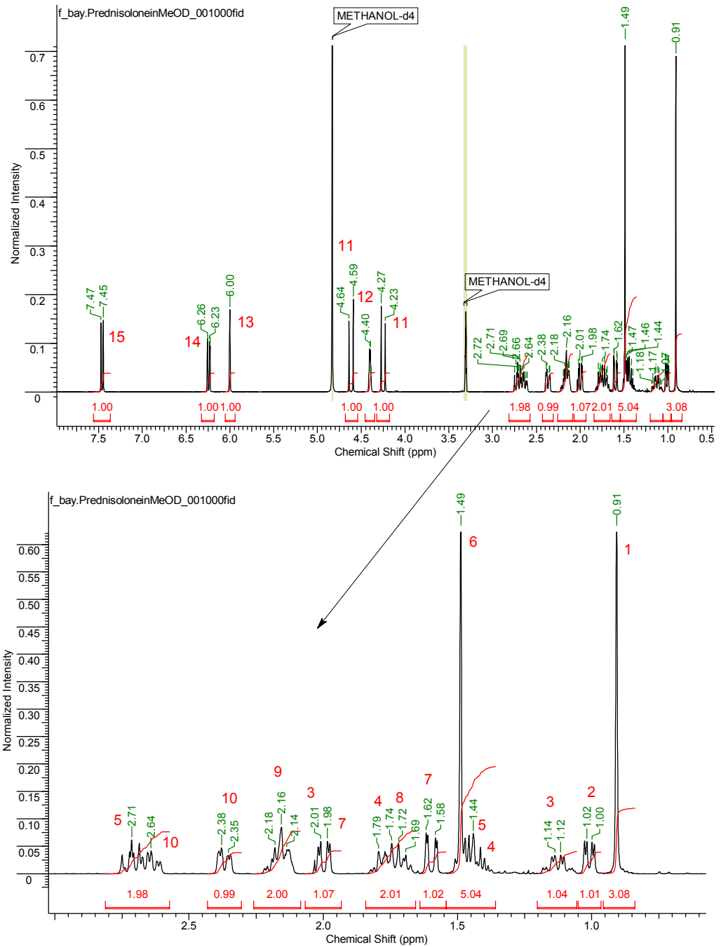
Fig.II.13. ^1\text{H} NMR of prednisolone and signal assignment Spectrum acquired on a Bruker AV(III)400 spectrometer, 16 scans, in MeOD
