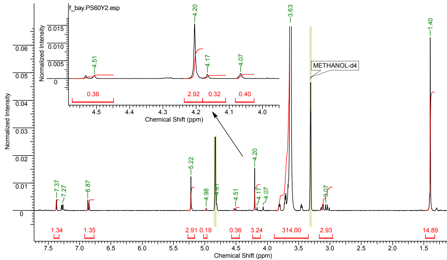
Fig. VI.48. ^1\text{H} NMR of purified PEG 3400 -salbutamol ester Spectrum acquired on a Bruker AV(III)400 spectrometer, 16 scans, in MeOD
