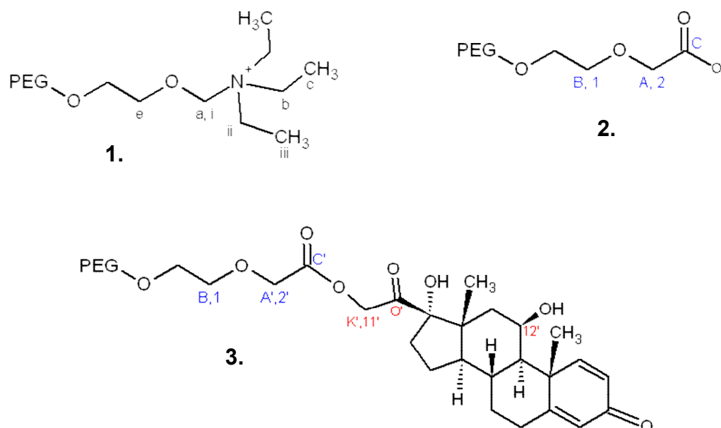
Fig.II.16. Different forms of PEG present in crude PP11 1.PEG-triethylammonium, 2. deprotonated PEG, 3. PEG-prednisolone
