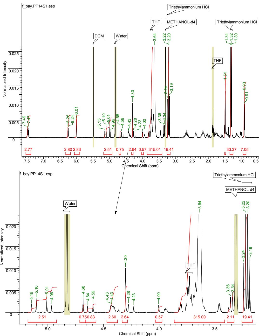
Fig.VI.9. 1 H NMR spectrum for PP14 crude Spectrum acquired on a Bruker AV(III)400 spectrometer, 64 scans, in MeOD
