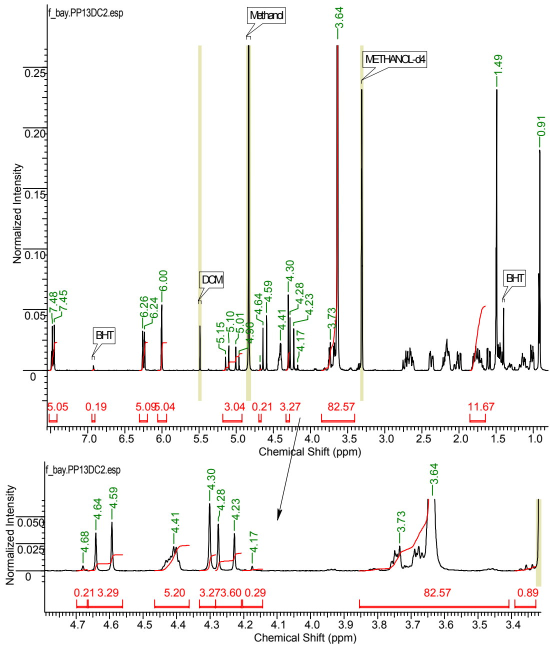
Fig.VI.20. ^1\text{H} NMR of PP13DC2 Spectrum acquired on a Bruker AV(III)400 spectrometer, 64 scans, in MeOD
