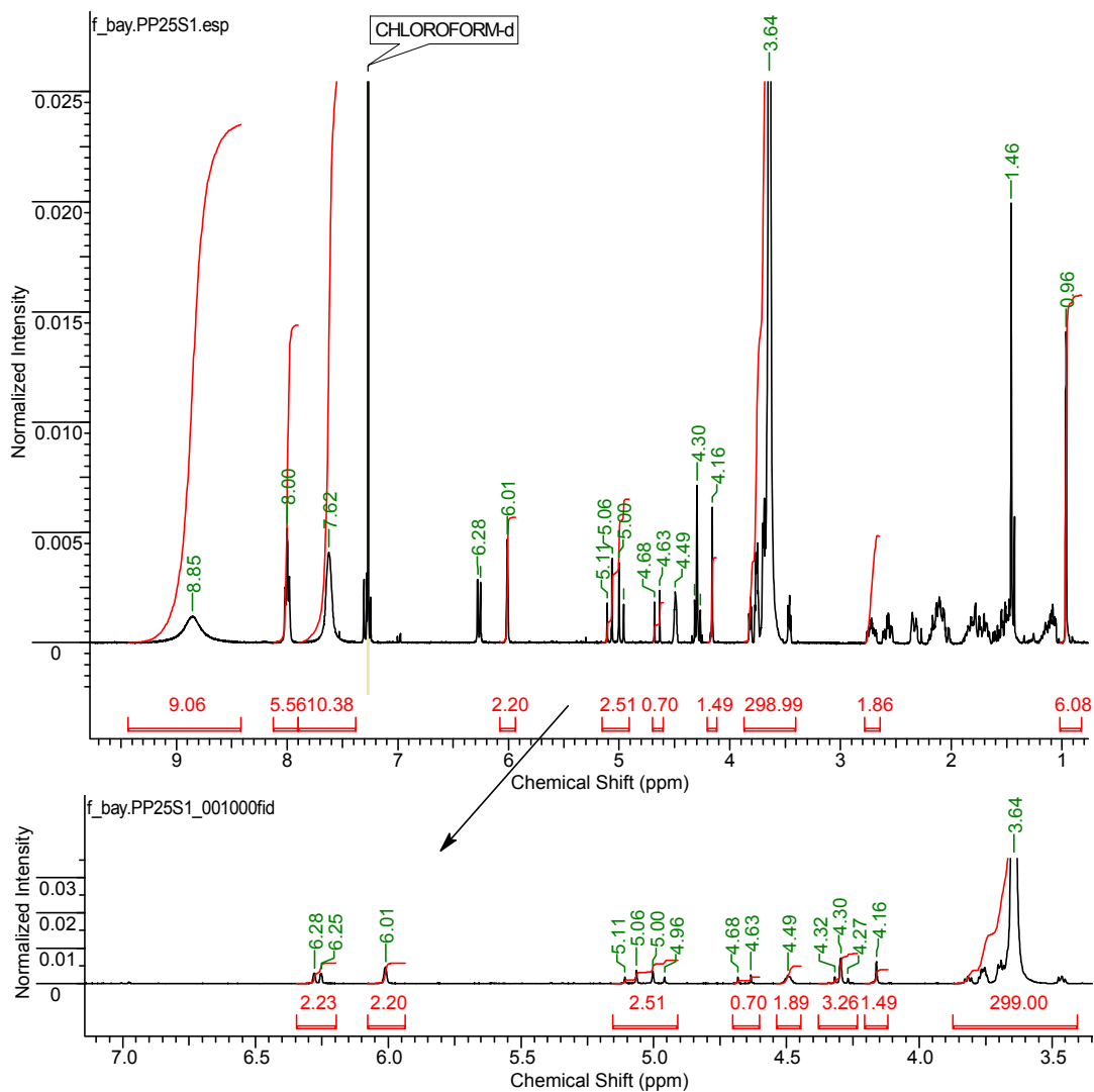
Fig.VI.26. 1 HNMR of PP25S1 Spectrum acquired on a Bruker AV(III)400 spectrometer, 64 scans, in CDCl 3
