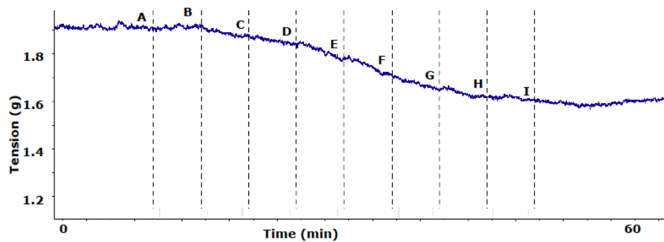
Figure 5.2 Representative trace of the response to anandamide in a mesenteric artery segment from a SHR rat. A=1nM, B=3nM, C=10nM, D=30nM, E=100nM, F=300nM, G=1µM, H=3µM and I=10µM.
