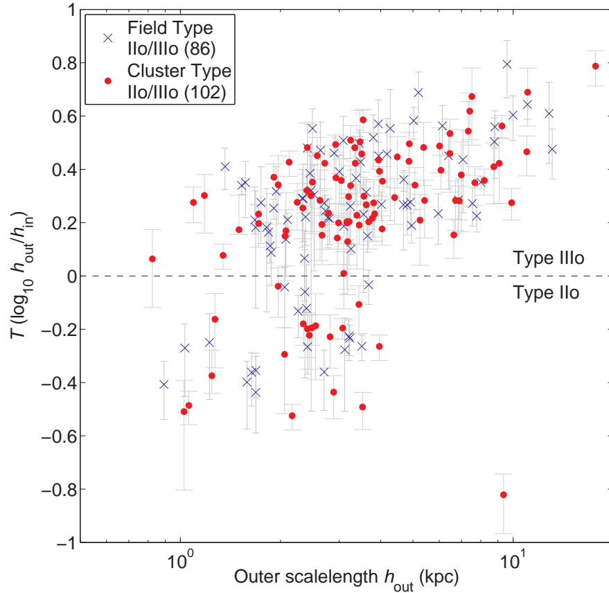
Figure 4.7. A comparison of break strength T and outer scalelength h_{\text{out}} for our Type II o /III o galaxies in the field (blue crosses) and cluster (red points) environment (DTM classification). An outlying cluster galaxy located at h_{\text{out}} = 453.2 kpc, T = 2.382 is not shown for clarity (object #60598; an unusual outer \mu profile make T and h_{\text{out}} potentially uncertain for this galaxy, however this fact has no effect on our results or our conclusions). The T error bars represent the error from the sky subtraction ( \pm 1\sigma ) on a galaxy–galaxy basis. The mean error in T is \pm 0.1 . Respective sample sizes are shown in the legend.
