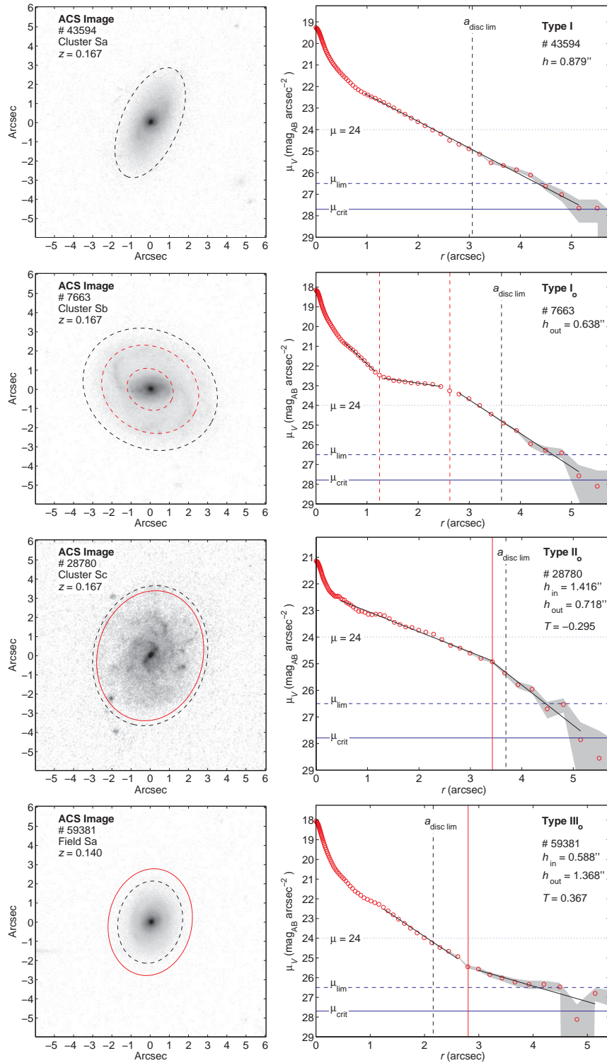
Figure 4.6. Examples of each class of profile (DTM classification). Top to bottom: Type I, Type I o , Type II o and Type III o . Left-hand panels: ACS V-band images. Right-hand panels: azimuthally-averaged V-band radial surface brightness \mu(r) profiles. We overplot the break radii in the outer stellar disc, 24 < \mu < 26.5 mag arcsec -2 (red solid lines). Also shown are break radii with \mu_{\text{brk}} < 24 mag arcsec -2 (red dashed lines), which are not considered in this study, and the stellar disc limit a_{\text{disc lim}} (black dashed line). The inner and outer scalelength, h_{\text{in}} and h_{\text{out}} , respectively, and the break strength T are also shown for reference. The ACS images are in a logarithmic grey-scale.
