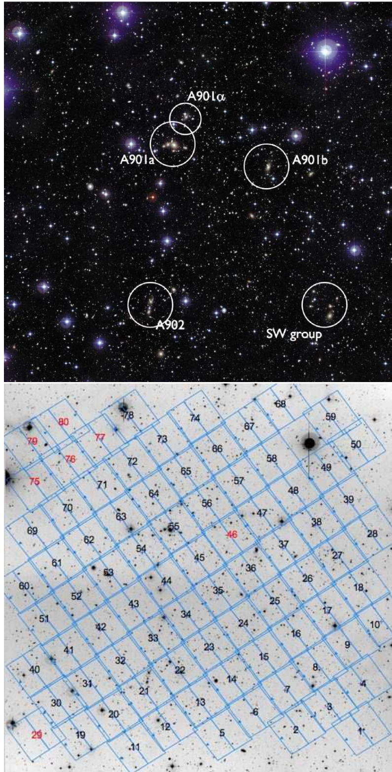
Figure 2.1. The STAGES A901/2 field. Top panel: an image of the complete A901/2 field created using colour information (RGB) from the ground-based COMBO-17 survey (Wolf et al. 2003). The cores of the three Abell clusters (A901a, A901b and A902) and the South-West (SW) group are encircled for reference (note: also encircled is A901 \alpha – some suspected in-falling substructure related to A901a). Bottom panel: a schematic showing the HST /ACS 80-tile mosaic. Image credit – http://www.nottingham.ac.uk/astronomy/stages .
