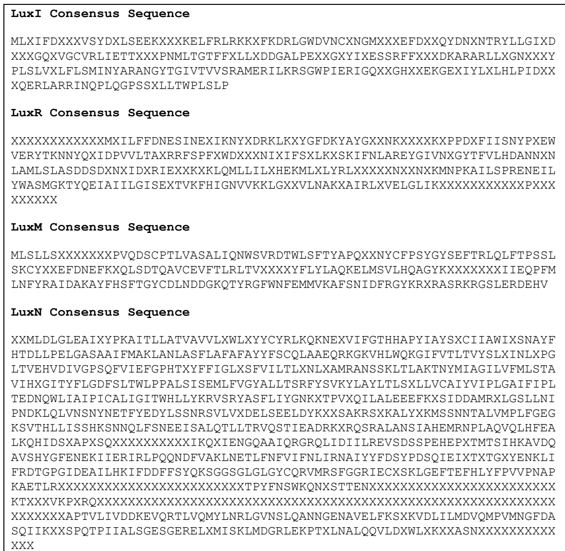
Figure 4.5. AHL synthase and AHL response regulator consensus sequences. The consensus sequences were generated from the majority consensus of ClustalW sequence alignments of multiple LuxI, LuxR, LuxM and LuxN homologues, X represents regions where no majority consensus was present in the alignment (see Appendices 4-7).
