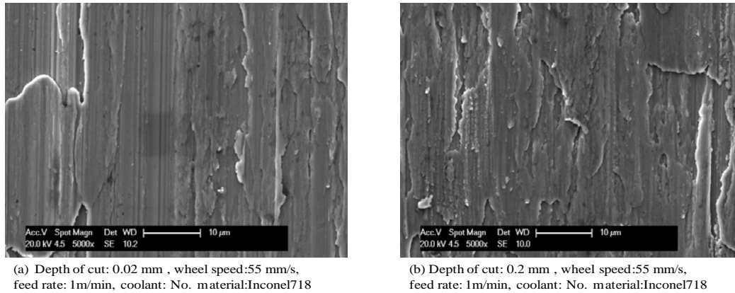
Figure 5-11: SEM images of Inconel718.
