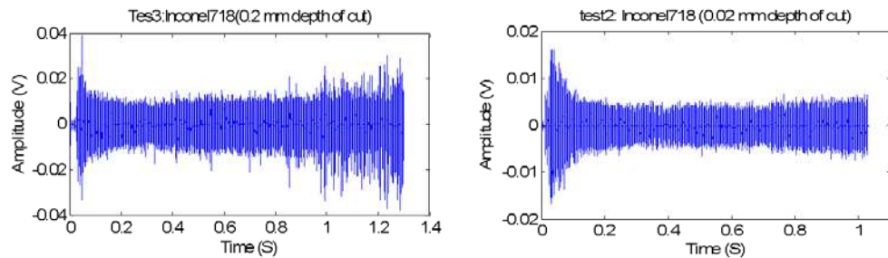
Figure 5-8: The time series plot of burn and no burn phenomena across the total extracted signal (Material: Inconel718).
