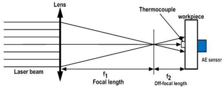
Figure 3-1: Schematic diagram of laser irradiation optical arrangement.
