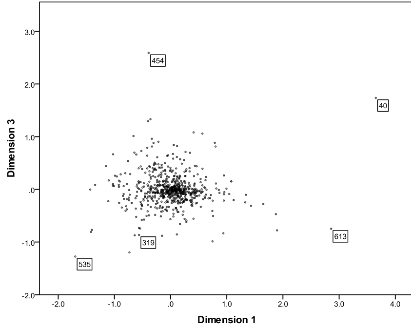
FIGURE 6.12 Dimension 1 against Dimension 3
