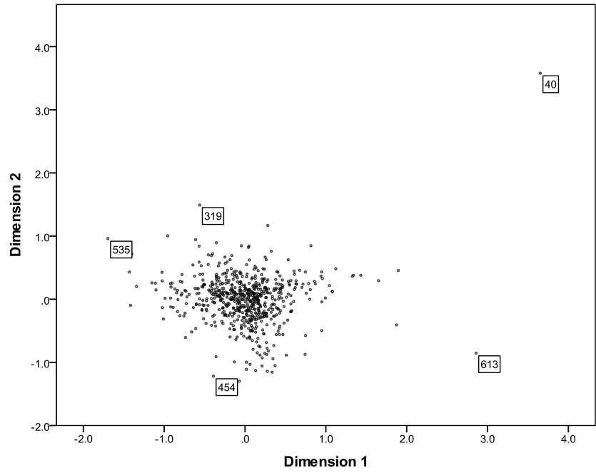
FIGURE 6.11 Dimension 1 against Dimension 2
