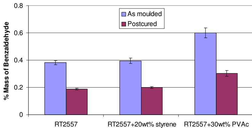
Figure 3.11: The influence of 20wt% additional styrene and 30wt% PVAc on the levels of residual benzaldehyde when compared to the base resin (RT2557), as detected by GC. Additional styrene had minimal affect on the residual benzaldehyde levels. However, the inclusion of PVAc increased benzaldehyde levels significantly. Postcuring reduced each system to half of its original value.
