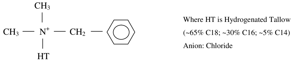
Figure 4.4: Cloisite® 10A chemical structure.
