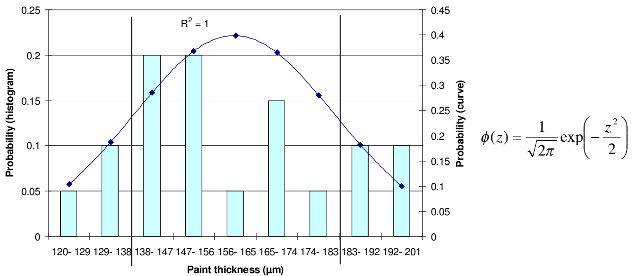
Figure A2.1: Gaussian distribution for total paint thickness.
