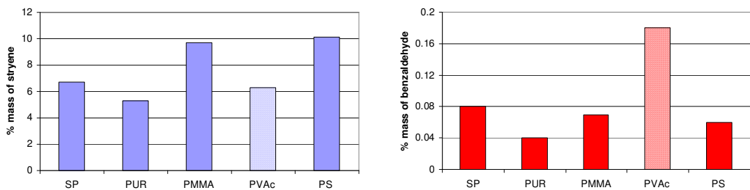
Figure 3.4: Effects of LPA type on residual styrene and benzaldehyde levels immediately after moulding [4]. The higher loading of styrene as solvent in LPA generally has an increased effect on residual styrene, with benzaldehyde production in PVAc increasing dramatically. Constituents are listed in Table 3.5.
