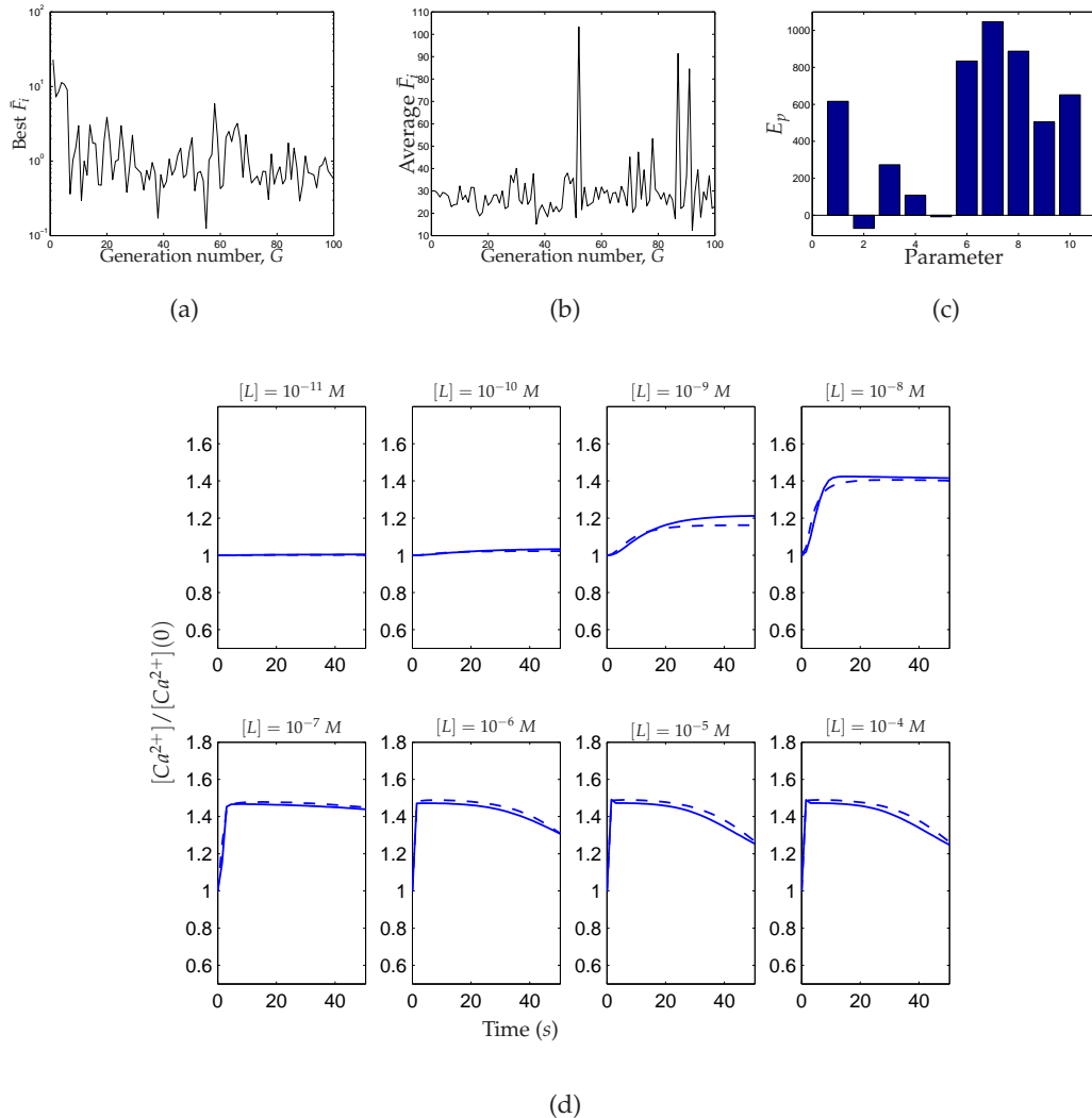
Figure 6.13: Searching in S_C^{10} \subset \mathbb{R}^{10} for the nominal values of the GSA Top 10, using the search parameters \lambda = 50 , G = 100 . (a) The value of F_i for the best individual found in a generation. (b) The average F_i of the whole population. (c) The errors associated with the estimates, calculated using equation (6.15). (d) The fits obtained with the best individual. As previously seen, the fits are very close to the pseudo-data, even though the estimates are considerably different from the nominal parameter values.
