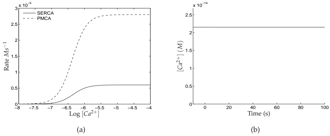
Figure 5.2: (a) A comparison of the rates of the SERCA ( p_1 = 6 \times 10^{-6} M s^{-1} , p_2 = 0.45 \times 10^{-6} M ) and membrane pumps ( V_P = 28 \times 10^{-6} M s^{-1} , K_P = 0.425 \times 10^{-6} M ). (b) There is no Ca^{2+} response to 10^{-7} M of Oxotremorine when V_P = 28 \times 10^{-6} M s^{-1} and K_P = 0.425 \times 10^{-6} M .
