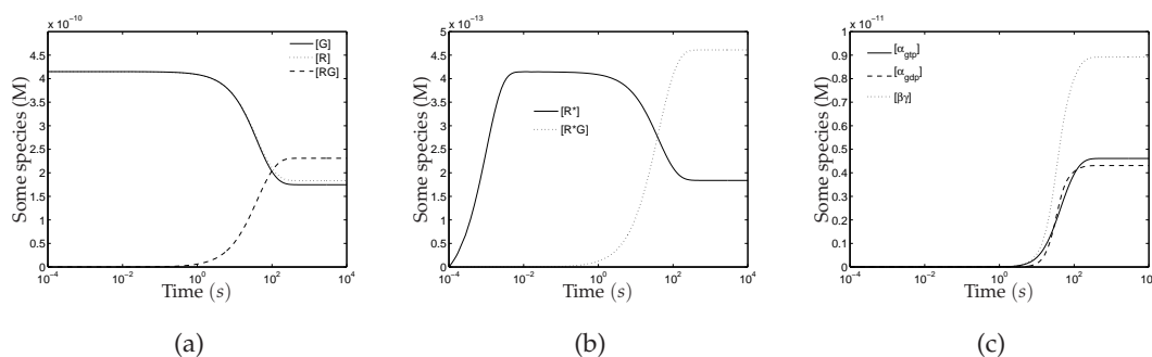
Figure 2.1: The unstimulated phase of signalling. (Note the log scale of the x axes.) Initially, only the unbound receptor ( R ) and G-protein states ( G ) exist. (a) Receptor pre-coupling occurs when the receptor and G-protein bind; (b) spontaneous receptor activation also occurs, allowing the active pre-coupled state ( R^*G ) to form; (c) some G-protein activation also occurs. The steady state levels of these species then serve as initial conditions for ligand stimulation.
