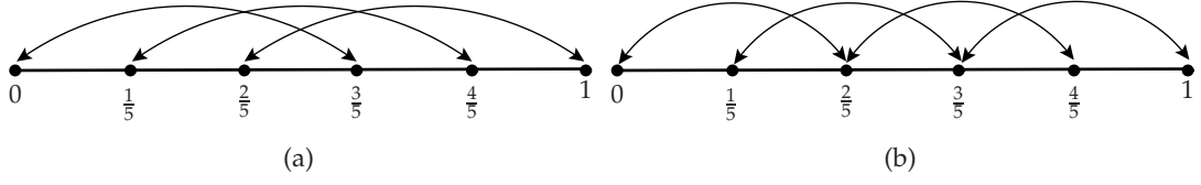
Figure 4.5: (a) A sampling scheme in which p = 6 , and \delta = \frac{p/2}{(p-1)} = \frac{3}{5} allows each point to be sampled with equal likelihood. (b) If, instead, \delta = \frac{p/3}{(p-1)} = \frac{2}{5} is chosen, points \frac{2}{5} and \frac{3}{5} are more likely to be sampled than the others.
