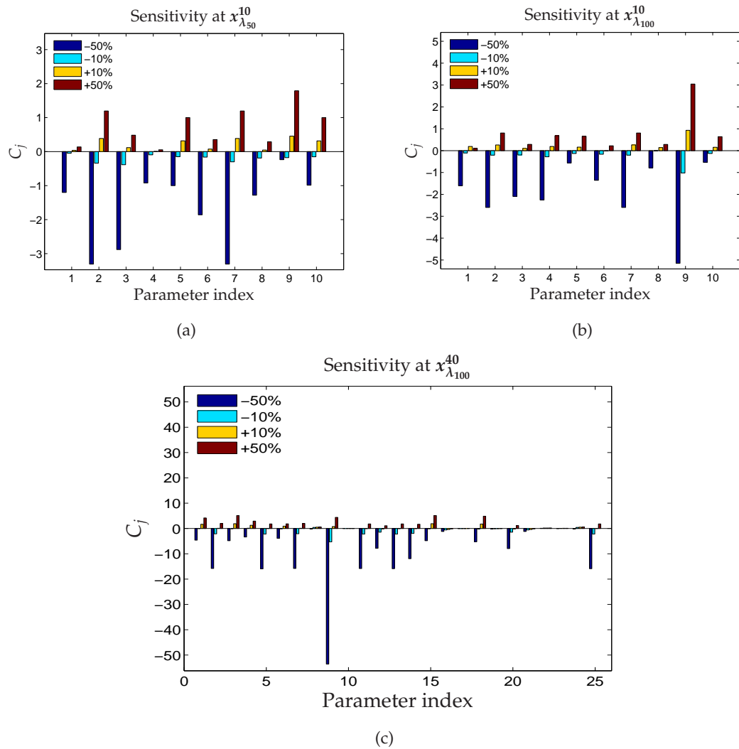
Figure 6.20: Sensitivity coefficients calculated (using equation 6.16) at the best three parameter sets found by SRES when fitting to the experimental data. (a) x_{\lambda_{50}}^{10} , (b) x_{\lambda_{100}}^{10} , (c) x_{\lambda_{100}}^{40} . Several of the same parameters are sensitive at all three points, including 2: k_{PIP_2b+} , 7: [PIP_2] , and 9: p_2 .
