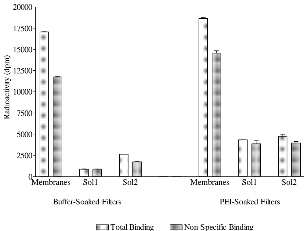
Figure 3.2: The effect of solubilization and filter pre-treatment on the total and non-specific binding of [ 3 H]-SR141716A to rat cerebellum membranes. Data are expressed as the mean \pm SEM of three determinations of [ 3 H]-SR141716A binding at each assay condition.
