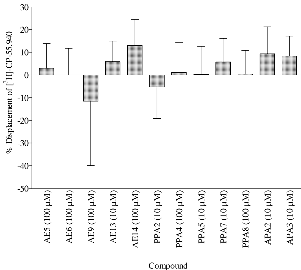
Figure 4.10: The displacement of [ 3 H]-CP-55,940 from porcine spleen membranes by aryl ethanolamide and phosphinic acid test compounds. Data are expressed as the mean \pm SEM of three independent experiments.
