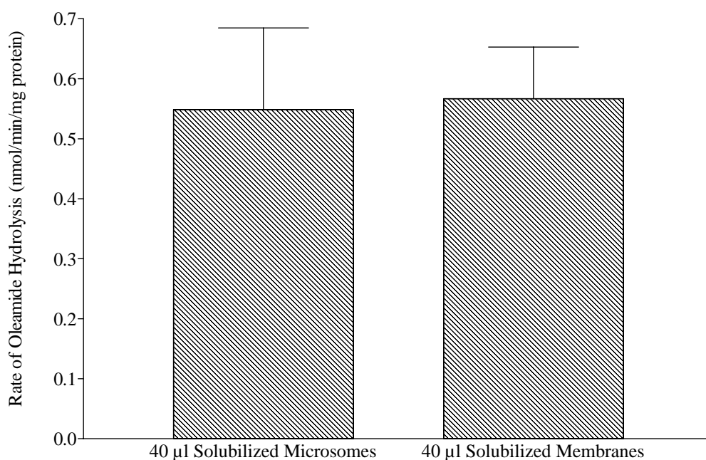
Figure 6.7: Comparison of the rate of FAAH-catalysed hydrolysis of 160 \mu M oleamide in solubilized preparations of rat liver microsomes and membranes. Data represent the mean \pm range of two determinations of rate. Protein concentrations were determined prior to solubilization of the tissue preparations.
