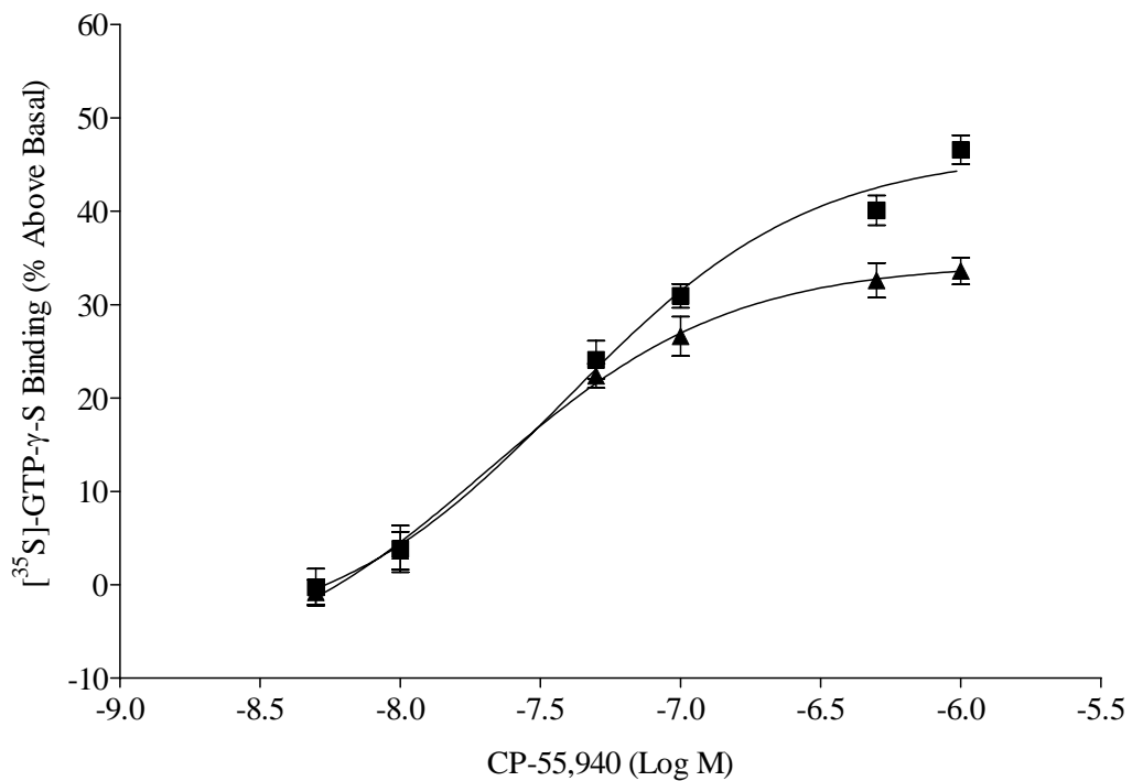
Figure 3.6: CP-55,940-stimulated [ 35 S]-GTP-γ-S binding to rat brain membranes using 50 μM (■) and 100 μM (▲) GDP. Data are expressed as the mean ± SEM of three determinations of [ 35 S]-GTP-γ-S binding and were fitted by non-linear regression using GraphPad Prism.
