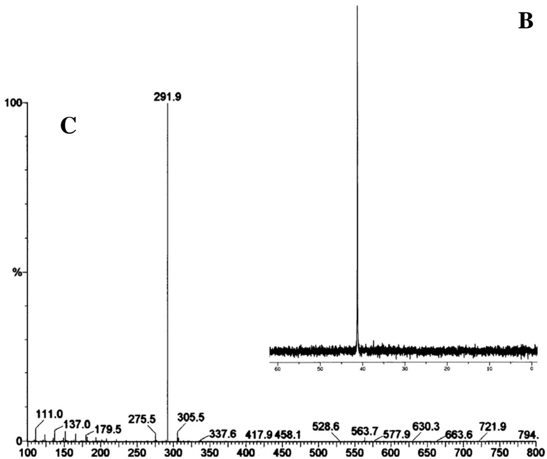
Figure B3: 1 H NMR spectrum (A) 31 P NMR spectrum (B) and mass spectrum (C) of compound APA2.
