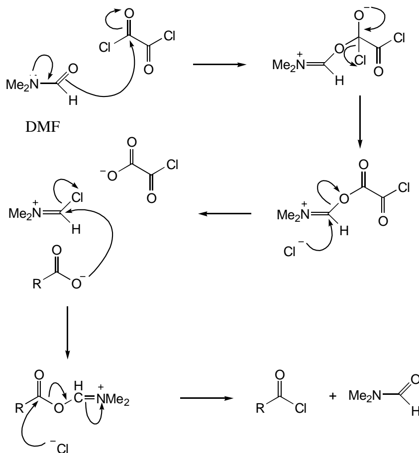
Scheme 2.4: Proposed mechanism of DMF-catalysed acid chloride synthesis using oxalyl chloride.
