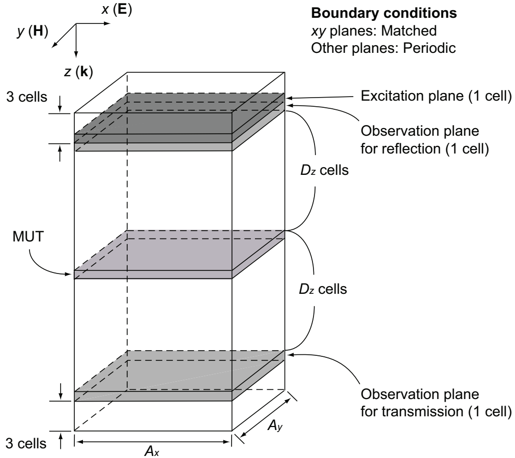
Figure 3.3: Simulation space for scattering parameter calculations.
