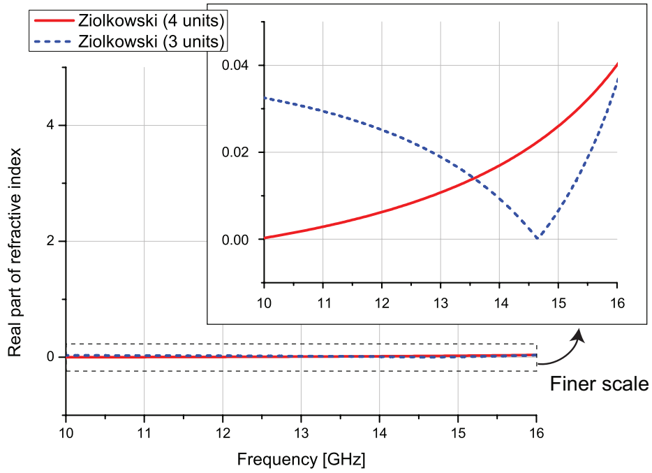
Figure 5.4: n' retrieved by Ziolkowski's method using wire units. The finer scale of the result is described in the inset.
