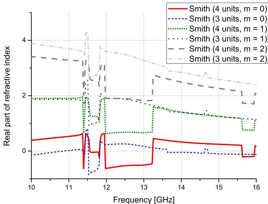
Figure 5.9: n' retrieved by Smith's method using LHM units.
