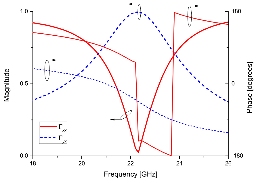
Figure 9.3: L -shaped metamaterial (top) and its reflection coefficients (bottom). A_x , A_y , l , w , t_m and t_s were modelled to be 6.3, 6.3, 5.7, 0.3, 0.0 and 1.2 mm by cubical unit cells of \Delta l = 0.075 mm. The electromagnetic properties of the substrate were \epsilon_r = 1.0 and \mu_r = 1.0 . No loss factor was implemented. The reflection coefficients were calculated along x axis which was the same as the incident electric field direction ( \Gamma_{xx} ) and y axis ( \Gamma_{yx} ). The polarisation of the electric field was changed by 90 degrees at around 22 GHz.
