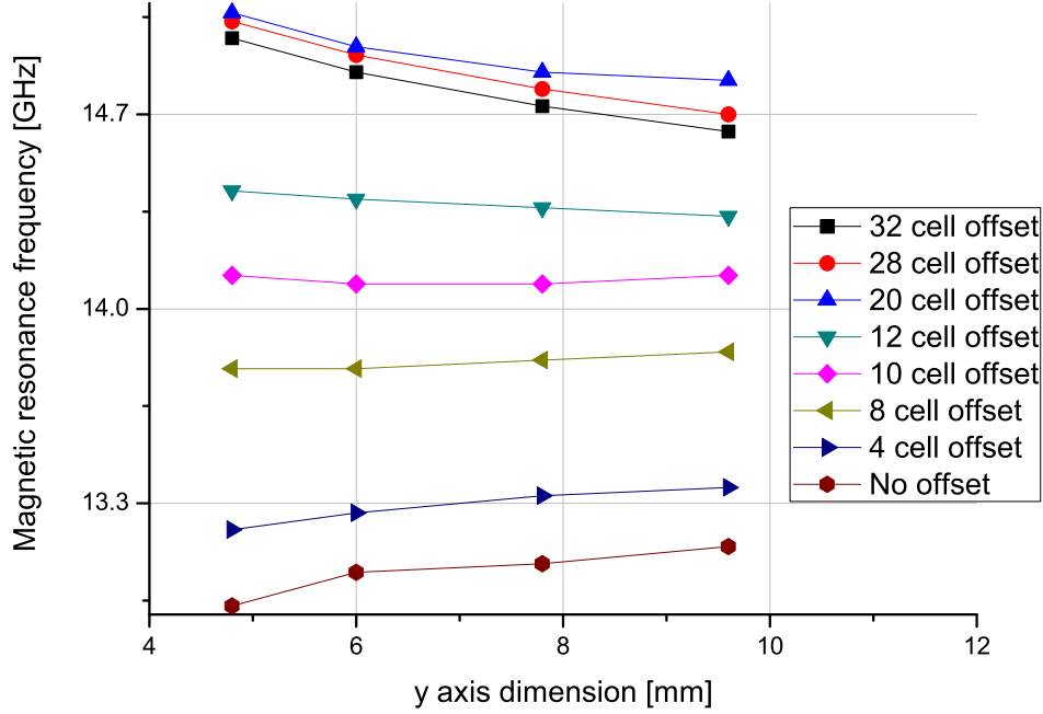
Figure 4.23: Magnetic resonant frequencies for asymmetrically paired CW arrays with various y axis periodicities.
