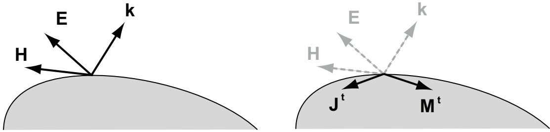
Figure 2.8: Incident wave (left) represented by Huygen's sources (right).
