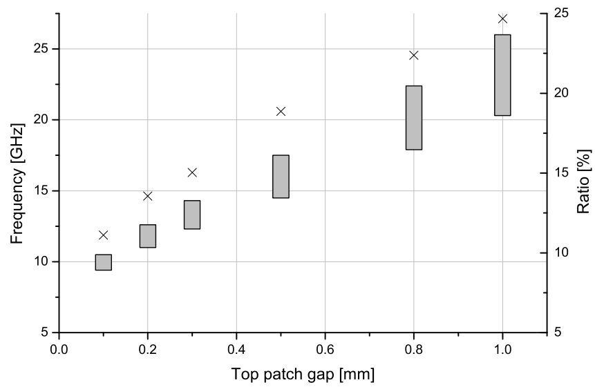
Figure 3.30: Reflection coefficient phase dependence of EBG structure on top patch gap. The top figure shows the reflection coefficient phase as a function of frequency up to 40 GHz. The bottom figure shows the in-phase reflection bandwidth (grey bars) and its ratio to the centre frequency (crosses).
