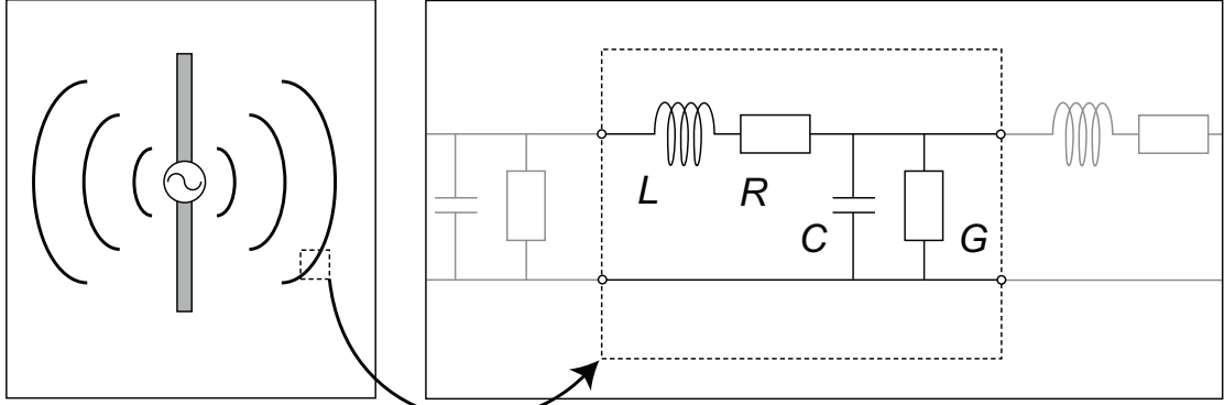
Figure 2.1: Analysis space (left) expressed by TLM method (right).
