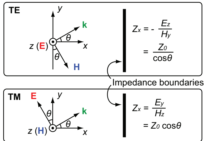
Figure D.3: Use of impedance boundary to reduce reflection of incident wave. The boundary is connected to Z_x of the characteristic impedance so that the reflection of the oblique wave is reduced.
