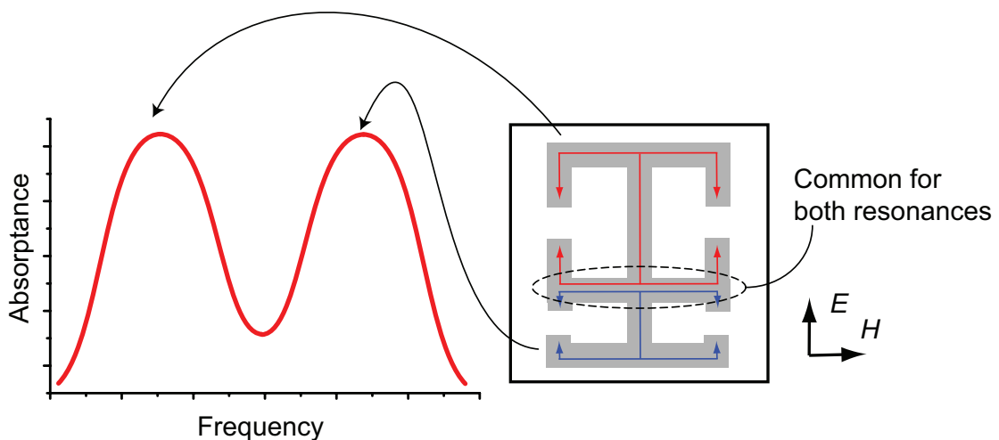
Figure 9.2: Example of metamaterial absorbers sharing metal geometry for double absorptance peak [77]. The metal geometry is placed close to a PEC wall. The middle part of the metal geometry is used for both first and second absorptance peaks (resonances).
