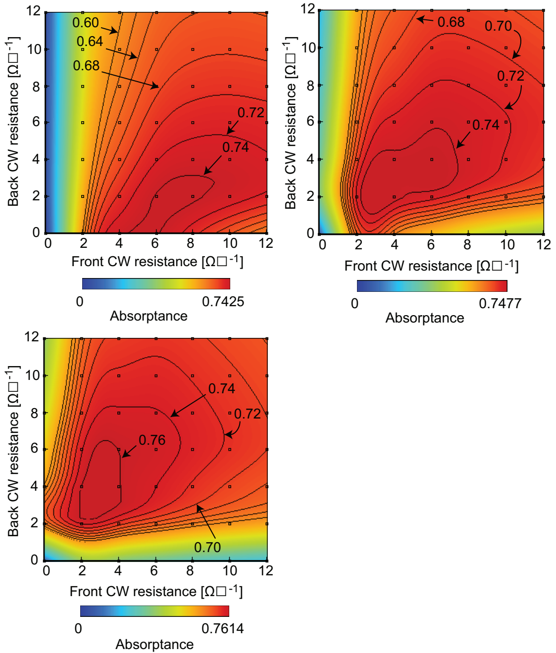
Figure 7.13: Various combinations of R applied for paired CW. The top left, top right and bottom left figures show the absorbances of no offset at 26.35 GHz, 1.2 mm offset at 26.23 GHz and 2.4 mm offset at 27.20 GHz, respectively. The dots in the figures represent the calculated sheet resistance patterns and the intermediate values were estimated by using spline interpolation.
