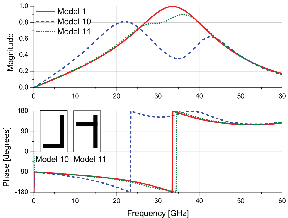
Figure 3.12: Reflection coefficient magnitudes (top) and phases (bottom) of decomposed y -shaped metamaterial models 1, 10 and 11.
