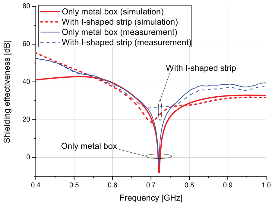
Figure 7.25: Measurement and simulation results of shielding effectiveness of metal box and its improvement by I-shaped strip. The top figure shows the I-shaped strip used. 50 Ω of a lumped resistor was used for this structure. The other part of the structure was composed of copper tape. The measurement and simulation results using the lumped resistor type of the I-shaped strip in the metal box are shown in the bottom figure.
