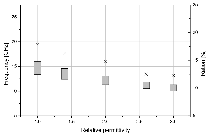
Figure 3.31: Reflection coefficient phase dependence of EBG structure on relative permittivity of substrate. The top figure shows the reflection coefficient phase as a function of frequency up to 40 GHz. The bottom figure shows the in-phase reflection bandwidth (grey bars) and its ratio to the centre frequency (crosses).
