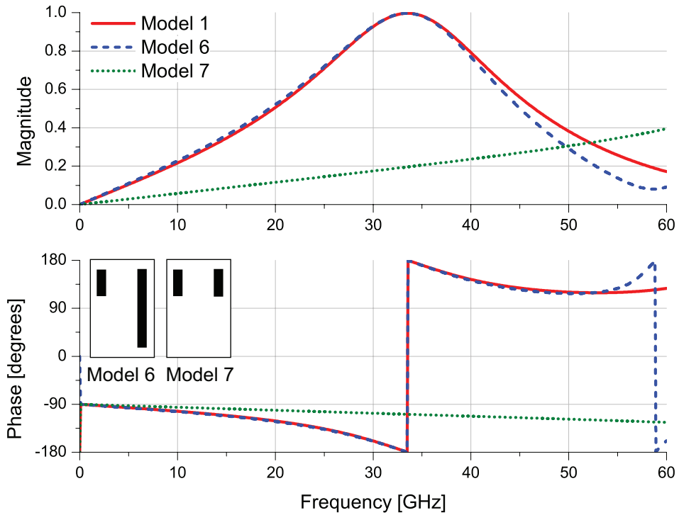
Figure 3.10: Reflection coefficient magnitudes (top) and phases (bottom) of decomposed y -shaped metamaterial models 1, 6 and 7.
