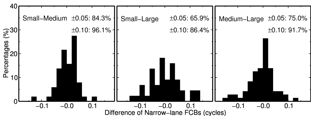
Figure 5.9: Distribution of narrow-lane FCB differences between the three ring networks. Note that satellite clocks based on the large ring-network are used in all three ring-network solutions
