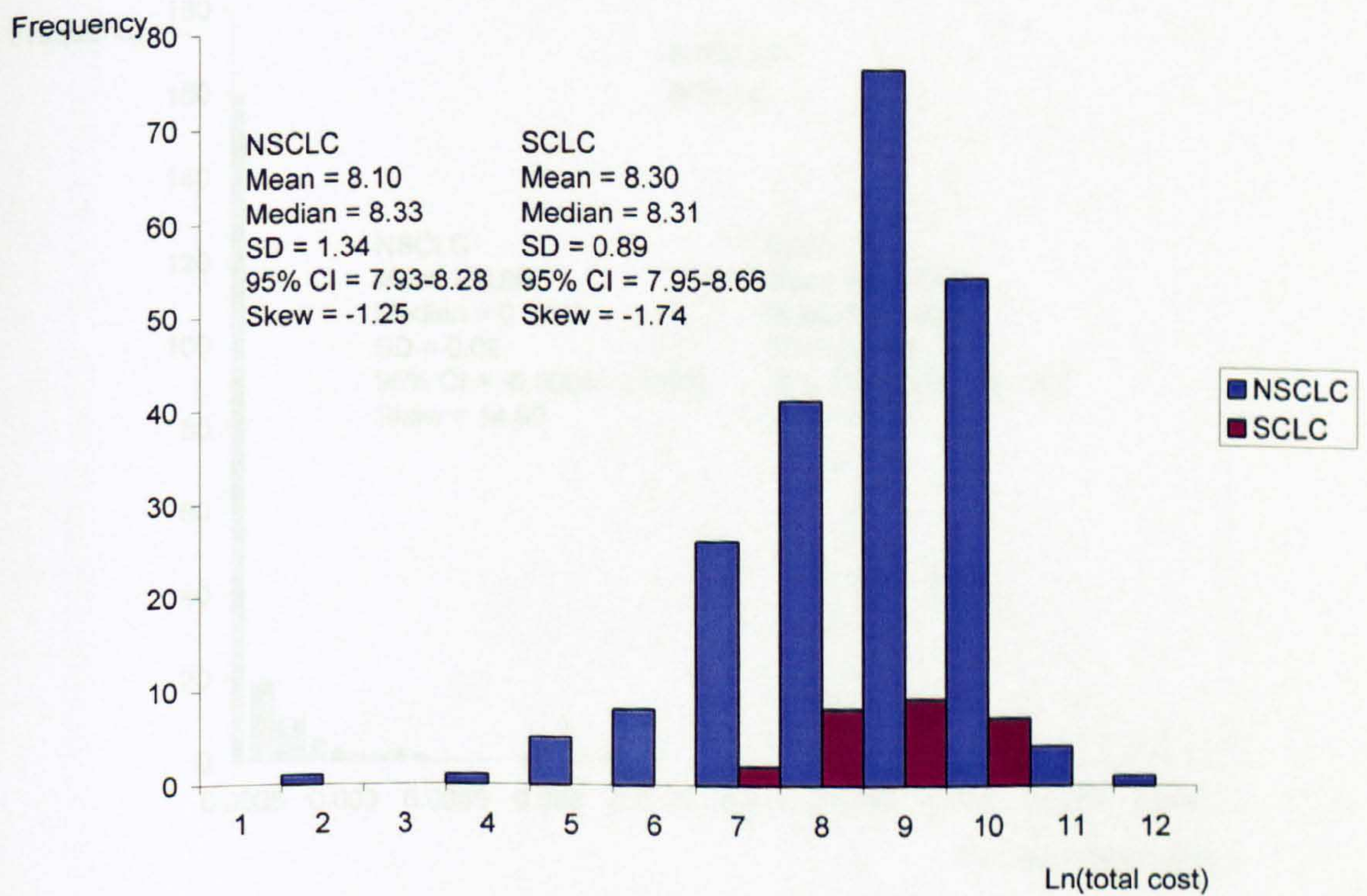
Figure 8.17 Histogram of Ln transformed lung cost data
