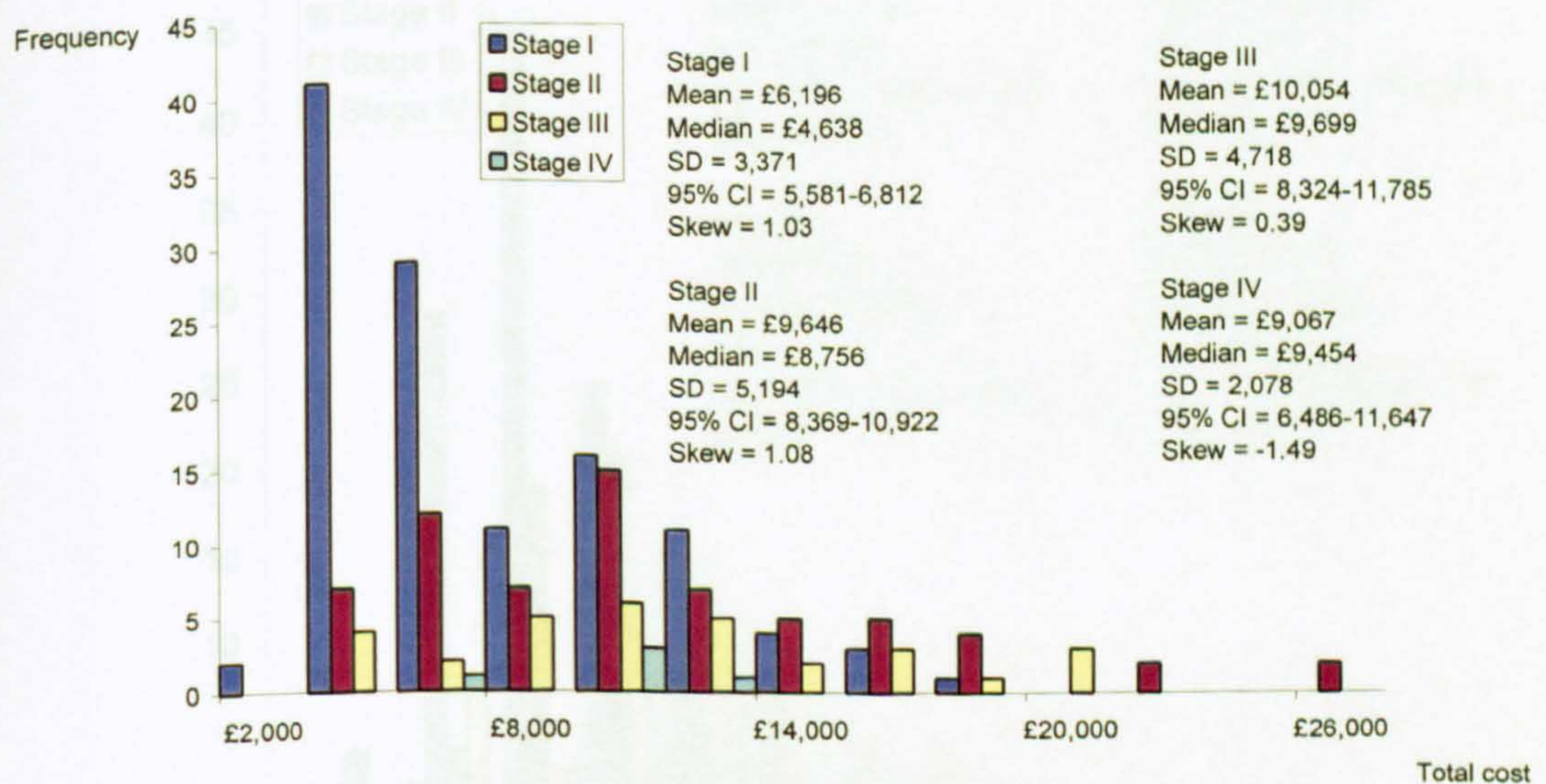
Figure 8.9 Histogram of cervical cost data with outliers removed
