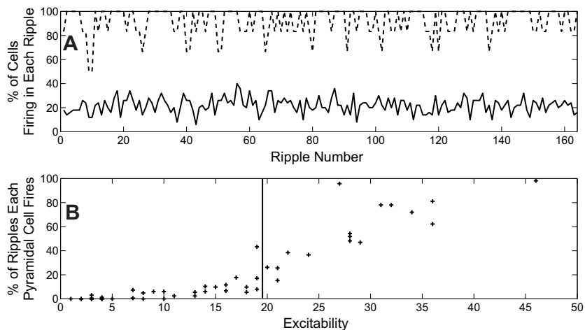
Figure 6.9: A: Percentage of pyramidal cells (solid line) and interneurons (dashed line) that fire on each detected ripple. B: Percentage of ripples during which each pyramidal cell fires, versus the cell's excitability (as number of synapses it receives per CA3 incoming connection). The vertical line represents the threshold (19.5 synapses per CA3 incoming connection) between the two pyramidal cell groups.
