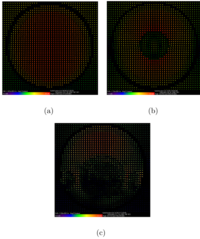
Figure 6.17: TE_{11} mode distribution: (a) in unloaded magnet bore; (b) in a loaded magnet bore with spherical phantom and (c) in the magnet bore loaded with HUGO body model.
