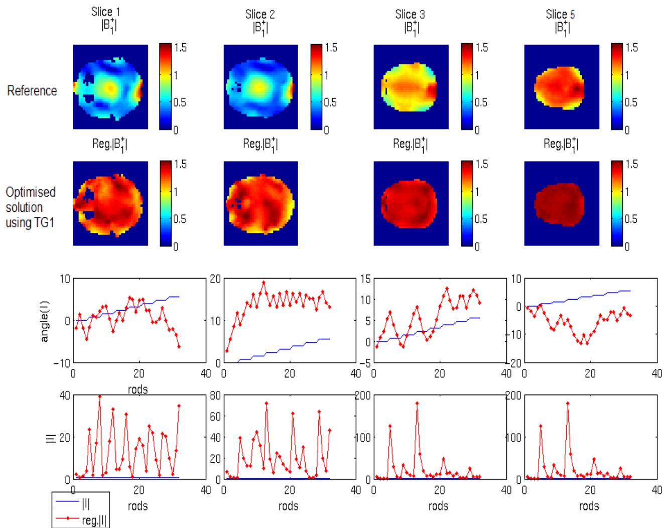
Figure 5.17: Rotational field map ( \mu T ) and currents' phases (radian) and amplitude (Amp) for 32 multi-elements coil for slices 1, 2,3 and 5.
