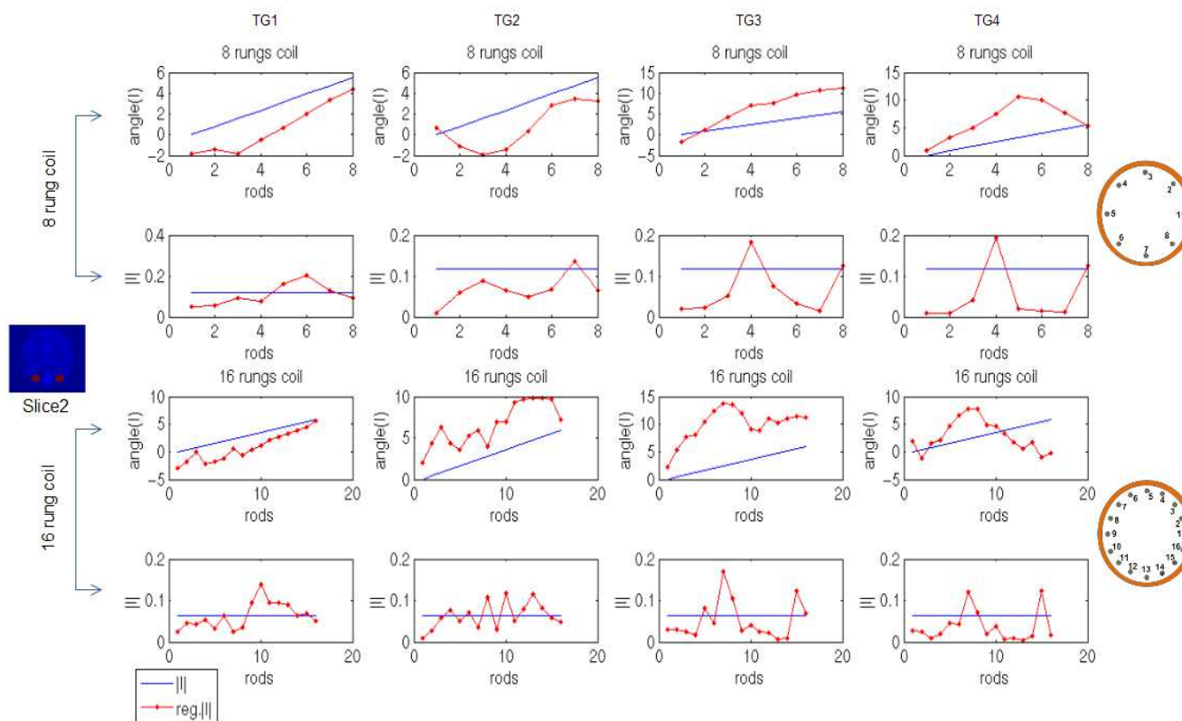
Figure 5.6: Currents and phases of the 8-rung coil, top two rows, and; of the 16-rung coil, bottom two rows, for the second slice using target fields (TG1, TG2, TG3 and, TG4) from left to right. The blue line represents the results of a standard coil and the red line represents the optimisation technique results (RF shimming).
