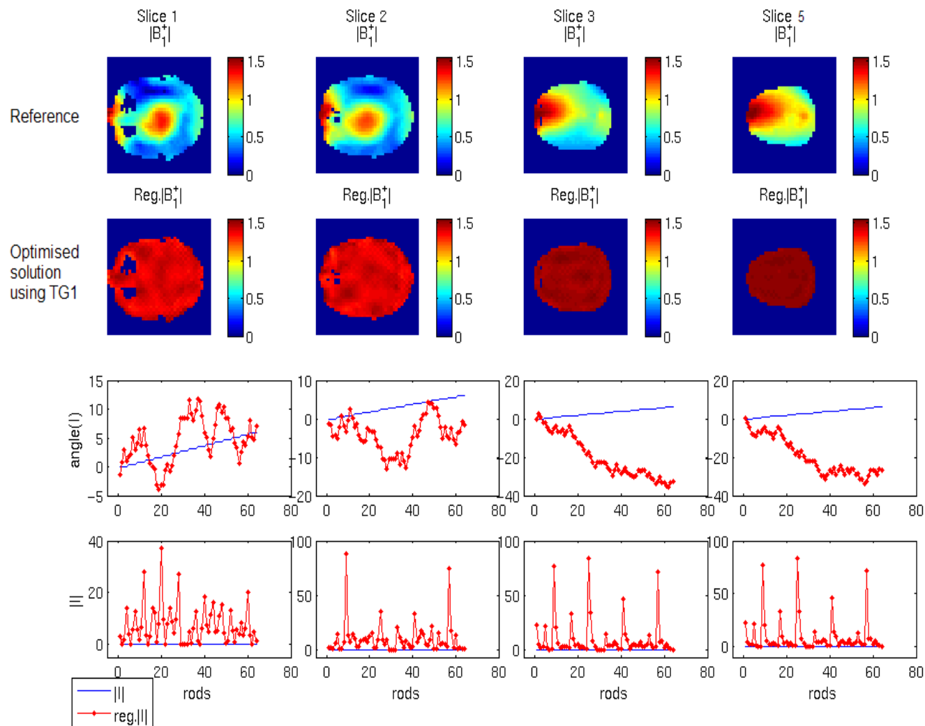
Figure 5.18: Rotational field map ( \mu T ) and currents' phases (radian) and amplitude (Amp) for 64 multi-elements coil for slices 1, 2,3 and 5.
