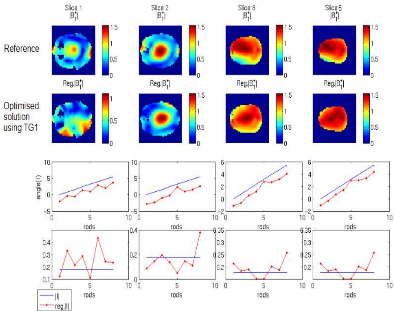
Figure 5.15: Rotational field map ( \mu\text{T} ) and currents' phases (radian) and amplitude (Amp) for 8 rung coil for slices 1, 2,3 and 5.
