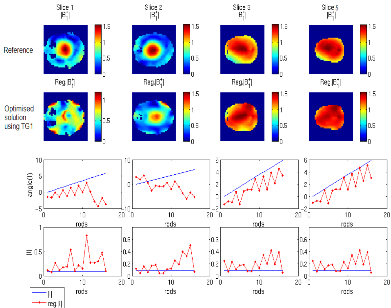
Figure 5.16: Rotational field map ( \mu T ) and currents' phases (radian) and amplitude (Amp) for 16 rungs coil for slices 1, 2,3 and 5.
