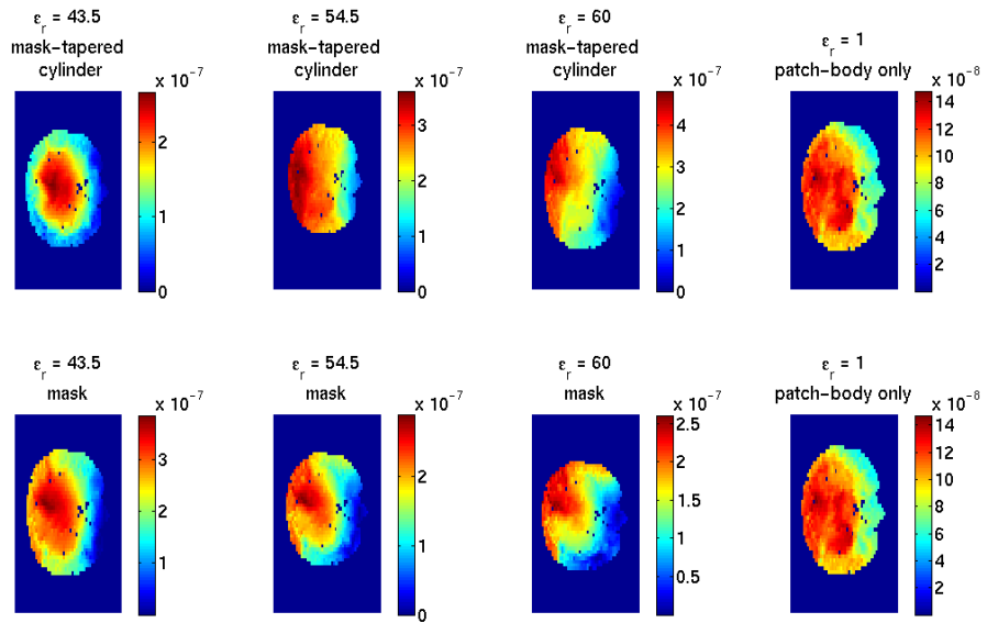
Figure 6.5: Field maps of a slice passing through the eyes; top: for tapered cylinder with match \epsilon_r = 43.5, 54.5, 60 and; bottom: for mask match with the same dielectric values both compared to the field maps of the same slice with no matching load.
