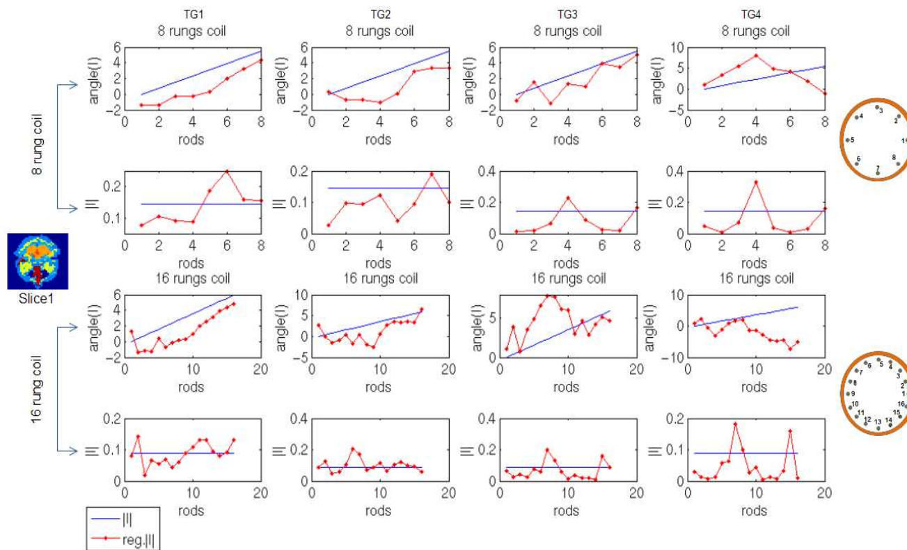
Figure 5.4: Currents and phases of the 8-rung coil, top two rows, and; of the 16-rung coil, bottom two rows, for the first slice using target fields (TG1, TG2, TG3 and, TG4) from left to right. The blue line represents the results of a standard coil and the red line represents the optimisation technique results (RF shimming).
