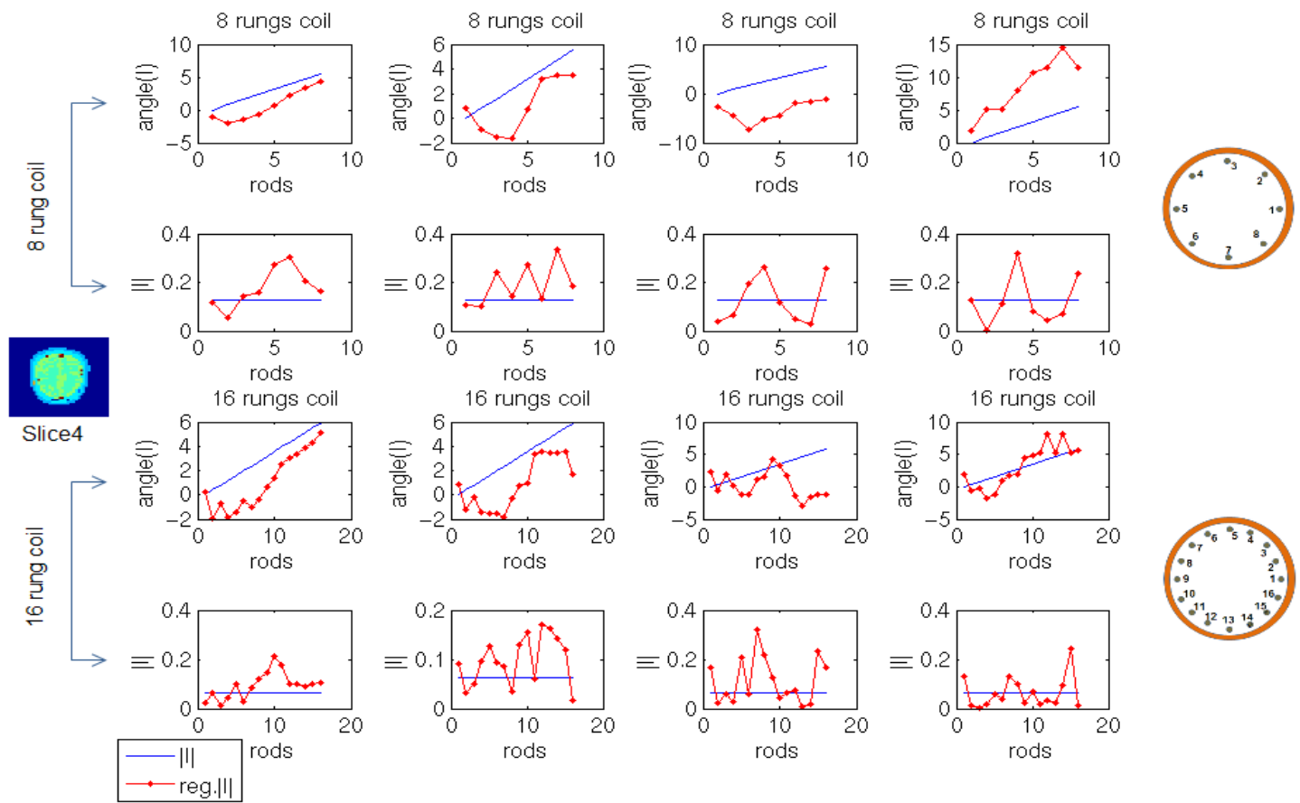
Figure 5.10: Currents and phases of the 8-rung coil, top two rows, and; of the 16-rung coil, bottom two rows, for the fourth slice using target fields (TG1, TG2, TG3 and, TG4) from left to right. The blue line represents the results of a standard coil and the red line represents the optimisation technique results (RF shimming).
