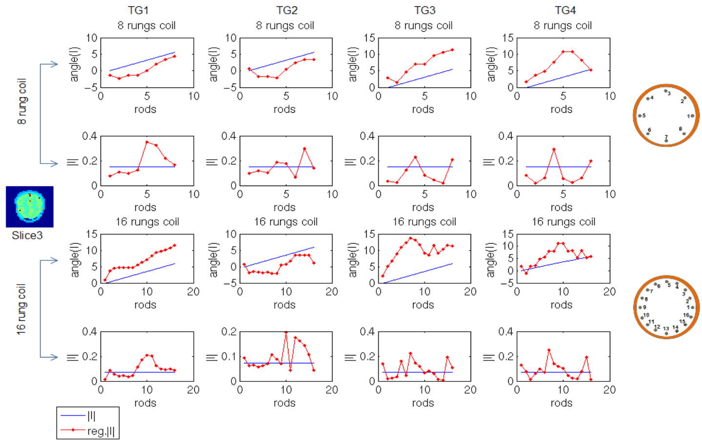
Figure 5.8: Currents and phases of the 8-rung coil, top two rows, and; of the 16-rung coil, bottom two rows, for the third slice using target fields (TG1, TG2, TG3 and, TG4) from left to right. The blue line represents the results of a standard coil and the red line represents the optimisation technique results (RF shimming).
