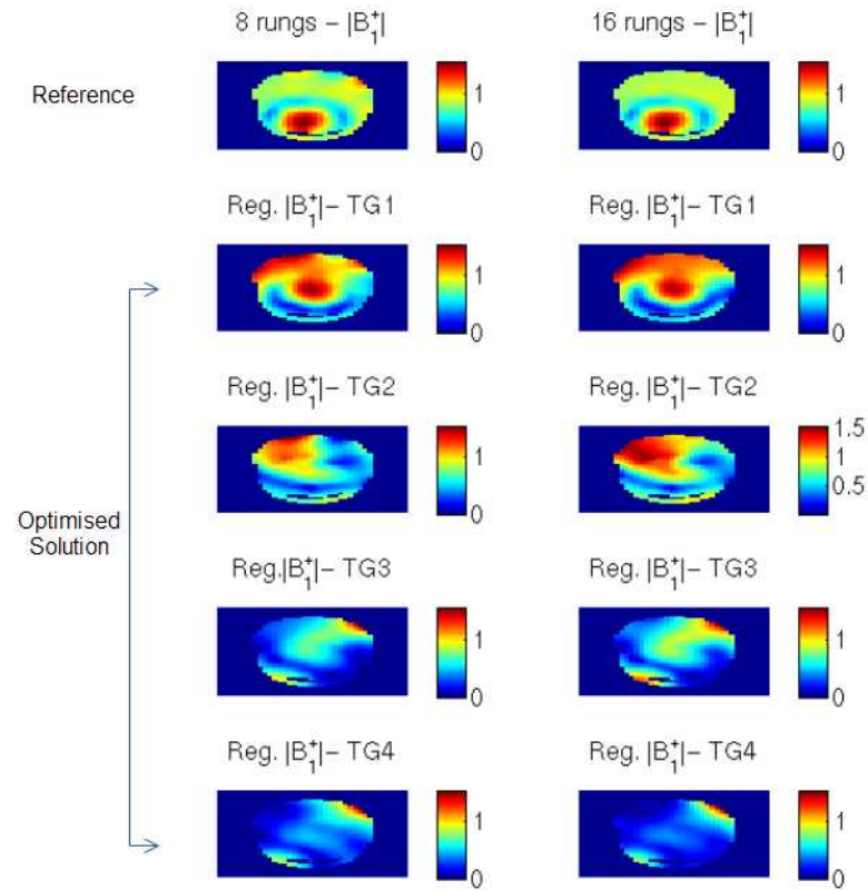
Figure 5.9: The field maps for the third slice: using 8-rung (left column) and 16-rung (right column) coils. The figure compares the results of a standard birdcage coil field maps (Top row) with optimised field maps using four target fields (RF shimming), (TG1) in the second row, (TG2) in the third row, (TG3) in the fourth row, (TG4) in the fifth row.
