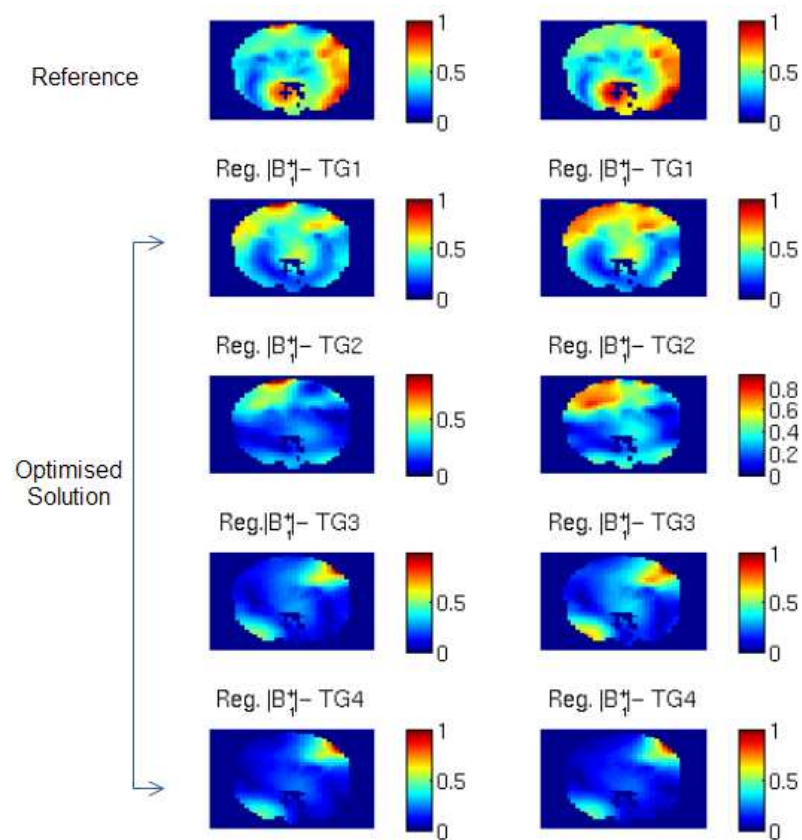
Figure 5.7: The field maps for the second slice: 8-rung (left column) and 16-rung (right column) coils. The figure compare the results of a standard birdcage coil field maps (Top row) with optimised field maps using four target fields (RF shimming), (TG1) in the second row, (TG2) in the third row, (TG3) in the fourth row, (TG4) in the fifth row.
