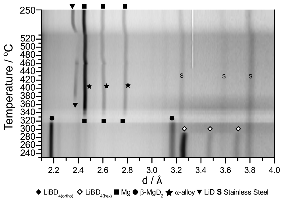
Figure 4.19. NPD data for 0.23\text{LiBD}_4 : \text{MgD}_2 through temperature ramp and cool under dynamic vacuum.
