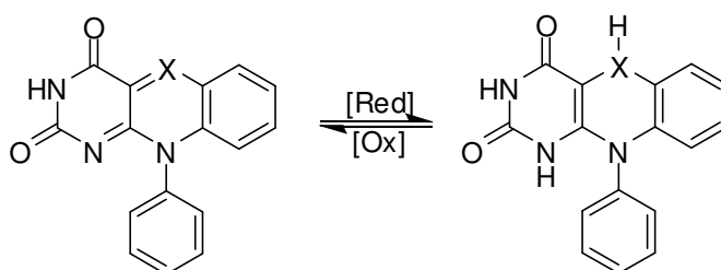
Figure 10. The redox system of the 5-deazaflavin and flavin compounds. X is a carbon atom for the 5-deazaflavins compound or a nitrogen atom for the flavin compound. Red stands for reduction. Ox stands for oxidation.
