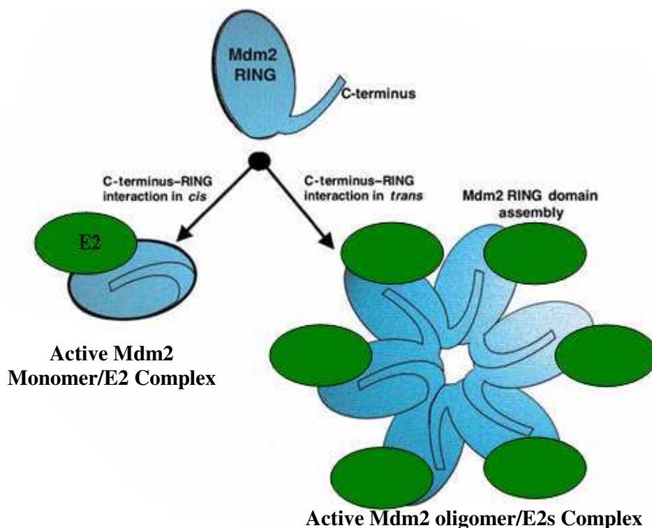
Figure 36. Schematic representation of the RING domain C-terminus of Mdm2 for the monomer and oligomer formation and role in ubiquitinylation. Blue oval represents Mdm2 with the tail respenting the RING domain C-terminus while the green oval represents E2. The extreme C-terminus of Mdm2 is able to form either intramolecular interactions forming a stable monomer that can interact with the required E2 or similar interactions with another Mdm2 RING domain which can lead to oligomer formation. Adapted from [289].
