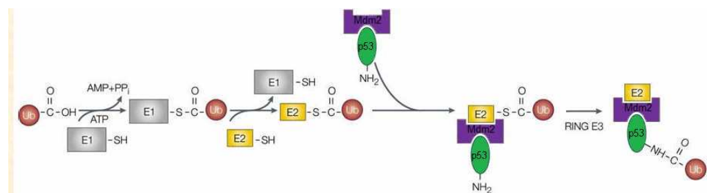
Figure 3. Ubiquitylation of p53. Where ubiquitin (ub, red), ubiquitin activating enzyme (E1, grey), ubiquitin conjugating enzyme (E2, yellow), Mdm2 (purple) acting as an E3 ubiquitin ligase and p53 (green), the substrate, are shown. Adapted from [150].
