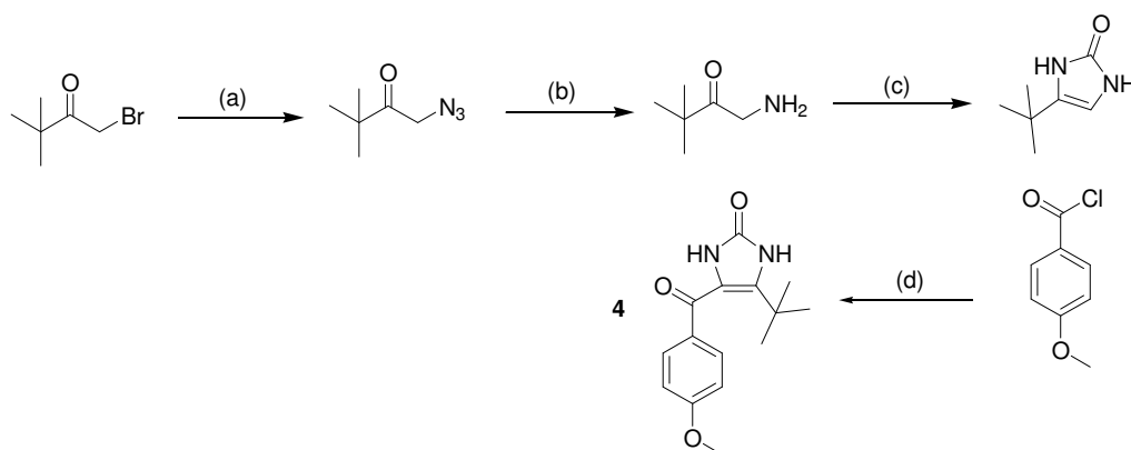
Figure 38. The synthetic pathway to produce the acylimidazolone compound, 4 . (a) NaN 3 , acetone, stirring (b) H 2 , Pd/C, conc HCl and ethanol (c) KOCN (aq) and Δ (d) AlCl 3 , nitrobenzene and Δ [293-297].
