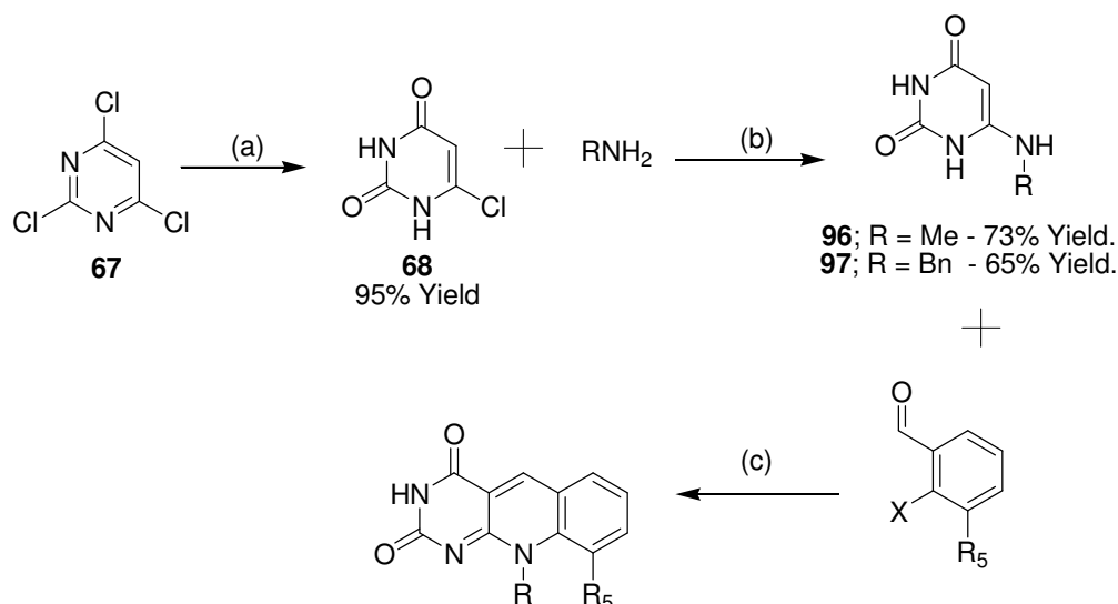
Figure 26. Synthesis of 10-substituted-5-deazaflavins analogues. (a) NaOH (aq) and 100 °C. (b) \Delta . (c) DMF and 160 °C. Where R = H, Me or Bn group, R 5 = H or CF 3 and X = F or Cl [241, 259-268].
