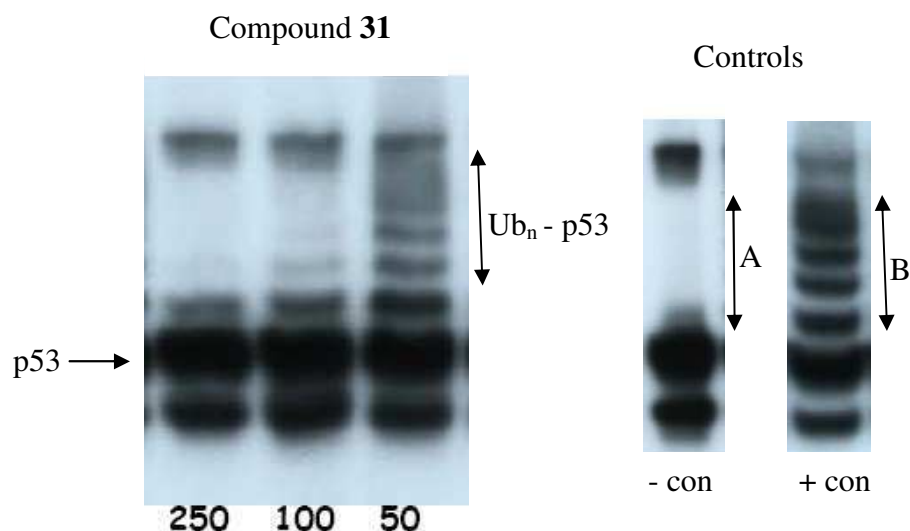
Figure 23. An example of the in vitro qualitative biological test on the inhibition of p53 ubiquitinylation for 31. The in vitro assay Western Blot of 31 at 250 \mu\text{M} , 100 \mu\text{M} and 50 \mu\text{M} concentration compared with the negative control (no ubiquitinylation of p53 seen and labelled as - con) and the positive control (ubiquitinylation or polyubiquitinylation of p53 seen and labelled as + con). A - represents no ubiquitinylation or polyubiquitinylation of p53 therefore no ubiquitinylation has occurred. B - represents ubiquitinylation or polyubiquitinylation of p53 therefore ubiquitinylation has occurred. All bands represent p53 protein, as identified by an anti-p53 antibody, with p53 or either the monoubiquitinylation or polyubiquitinylation, with different ubiquitin branching, forms of p53 ( \text{Ub}_n - \text{p53} ) shown and labeled. Compound 31 and the control blots shown from different Western Blots to ease comparison. At 250 \mu\text{M} concentration, the compound is stated as an excellent inhibitor. At 100 \mu\text{M} concentration, the compound is stated as a reasonable inhibitor. At 50 \mu\text{M} concentration, the compound is stated as inactive as an inhibitor of p53 ubiquitinylation [282].
