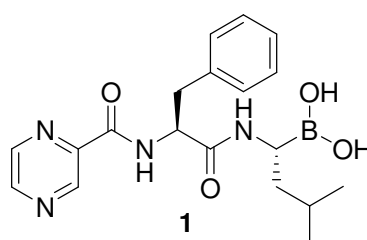
Figure 5. The chemical structure of Bortezomib, 1.
