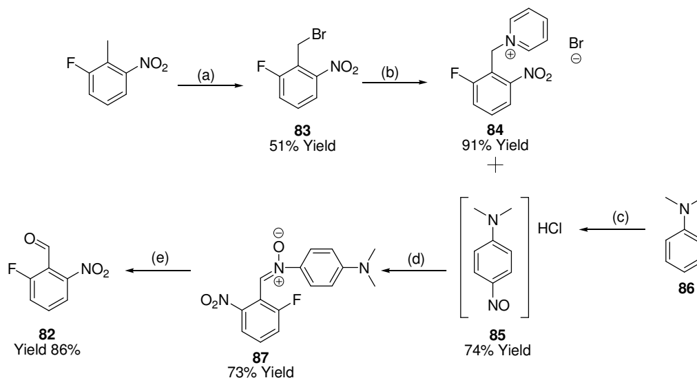
Figure 21. The Synthesis of 2-Fluoro-6-nitrobenzaldehyde, 82. (a) N-bromosuccinimide, benzoyl peroxide, CCl 4 and 80 °C. (b) EtOH, pyridine and 80 °C. (c) sodium nitrite and conc HCl. (d) EtOH and NaOH. (e) Conc H 2 SO 4 [277-279].
