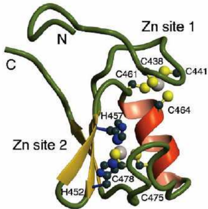
Figure 33. A ribbon representation of the lowest energy structure of Mdm2 RING domain. The diagram shows the distribution of regular secondary structure elements and the location of two Zn^{2+} -binding sites. The side chains of the zinc ligands are shown as spheres, coloured black (C), blue (N) or yellow (S) Where C = cysteine and H = histidine with the number meaning the number of the amino acid of the Mdm2 protein. This Figure was prepared using MOLMOL. Taken from [170].
