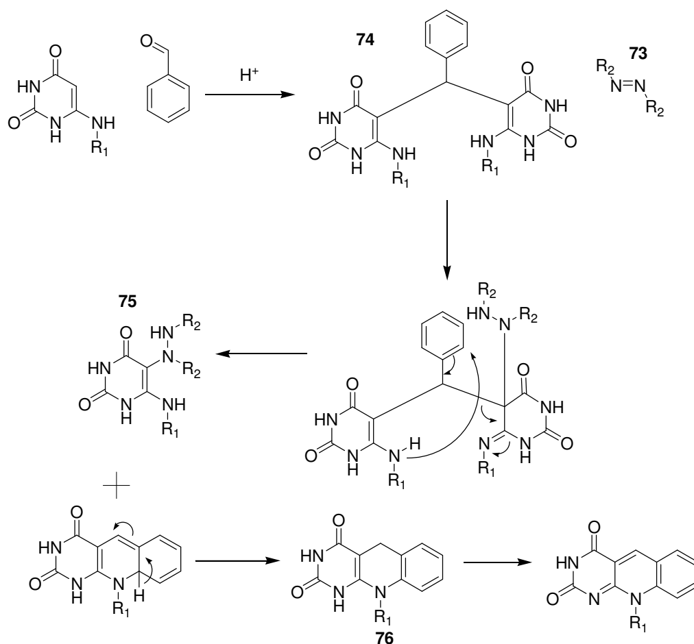
Figure 18. The mechanism of the DEAD method of 5-deazaflavin synthesis. Where R_1 = \text{Ph} and R_2 = \text{CO}_2\text{C}_2\text{H}_5 .
