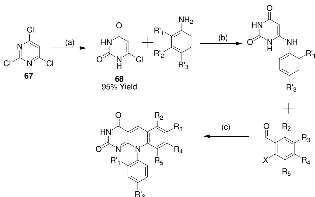
Figure 11. Synthesis of 5-deazaflavin analogues. (a) NaOH (aq) and 100 °C. (b) \Delta . (c) DMF and 160 °C where X = F or Cl [241, 259-268].
