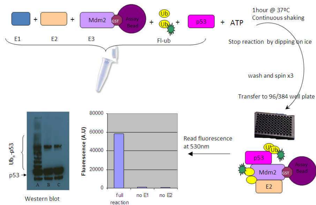
Figure 25. A diagram representing the new quantitative in vitro assay used to obtain IC_{50} data for inhibition of p53 ubiquitinylation. Where the E1 (blue square), E2 (cream square), Mdm2 (the E3, lilac square), GST (claret octagon), assay bead (purple circle), ubiquitin (yellow oval), fluorescently labelled ubiquitin (FI-ub, green explosion connected to ubiquitin) and p53 (fluorescent pink) are shown. The graph shows the full biochemical reaction and two negative controls, where ubiquitinylation could not occur do to the lack of E1 or E2 protein. The controls are preformed to calculate background fluorescents (or noise). The Western Blot of the washed and p53 labeled (by an anti-p53 antibody) assay is also shown for the full reaction (A), no E1 (B) and no E2 (C) controls. Ub_n - p53 stands for ubiquitin bound to p53 by either the monoubiquitinylated or polyubiquitinylated (with different ubiquitin branching) forms. Fluorecent obtained was converted to % inhibition of Mdm2 and used to yield IC_{50} data depending on whom carried out the biological assay (see data provided by the biological collabators in the Appendix titled IC_{50} In Vitro Assay Data 1, Mdm2 Auto-ubiquitinylation IC_{50} In Vitro Assay Data and IC_{50} In Vitro Assay Data 2). Diagram kindly provided by Dr Mezna from the Beatson Institute for Cancer Research [282].
