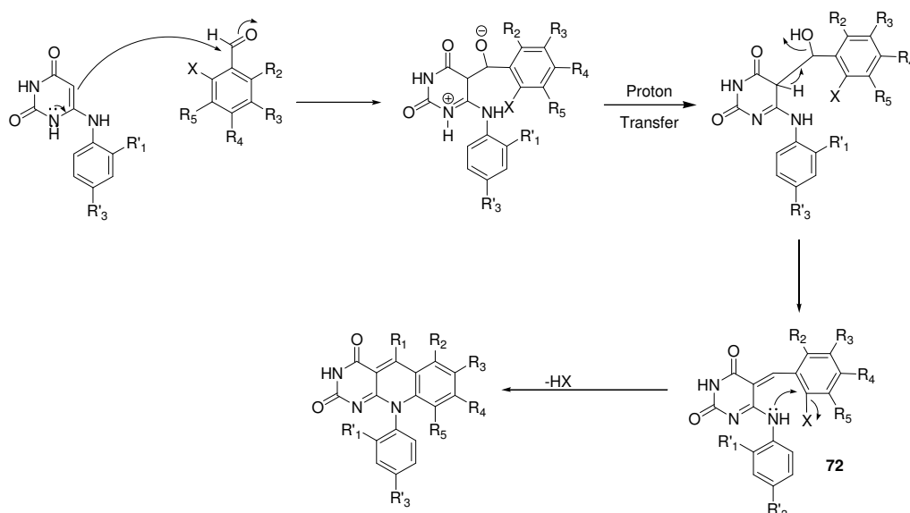
Figure 15. Another possible mechanism for the synthesis of 5-deazaflavin. Where X = F or Cl.
