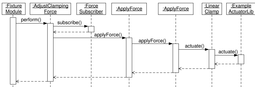
Figure 6-18: UML Sequence Diagram for the Force Adjustment in the Module Program
