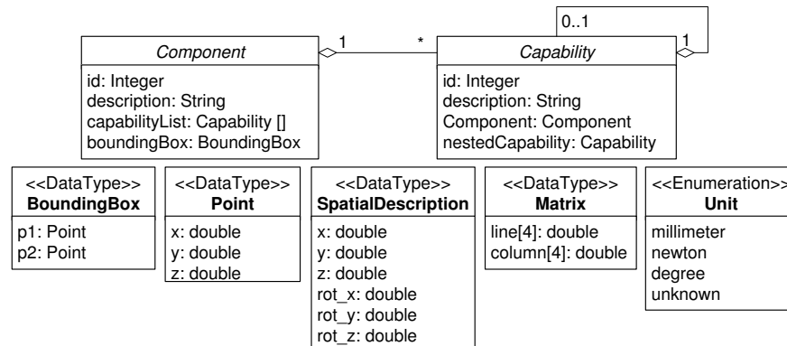
Figure 4-2: Model Elements of the Package “Common Elements”
