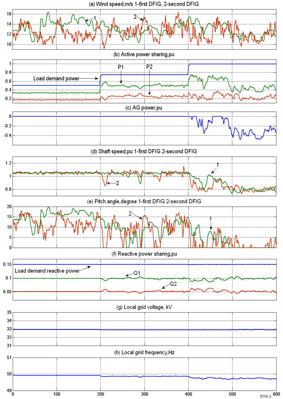
Figure 5.22. Sharing with the variable droop gain method
