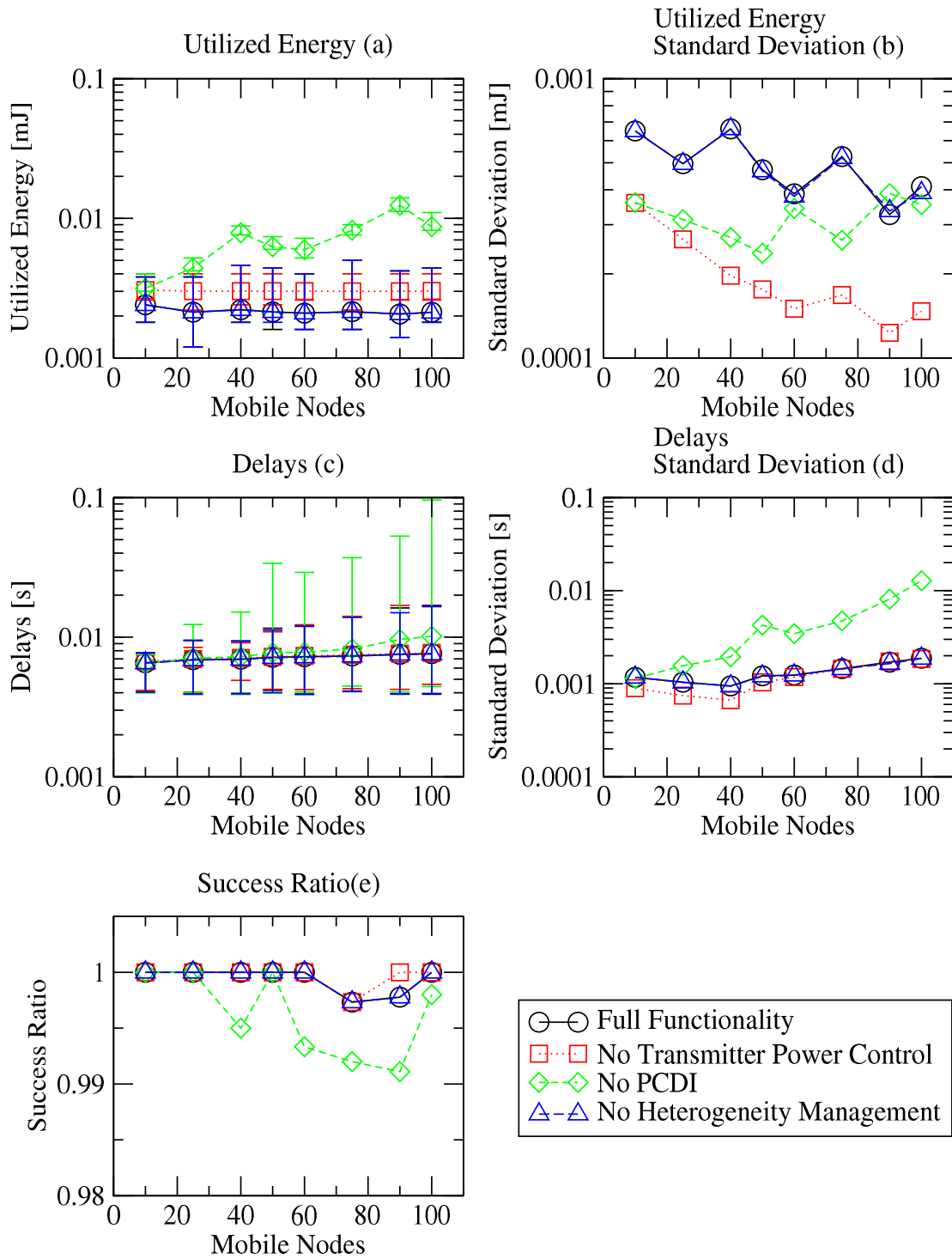
Figure 6.7. Evaluation of the utilized techniques – statistics for sending data to sinks
