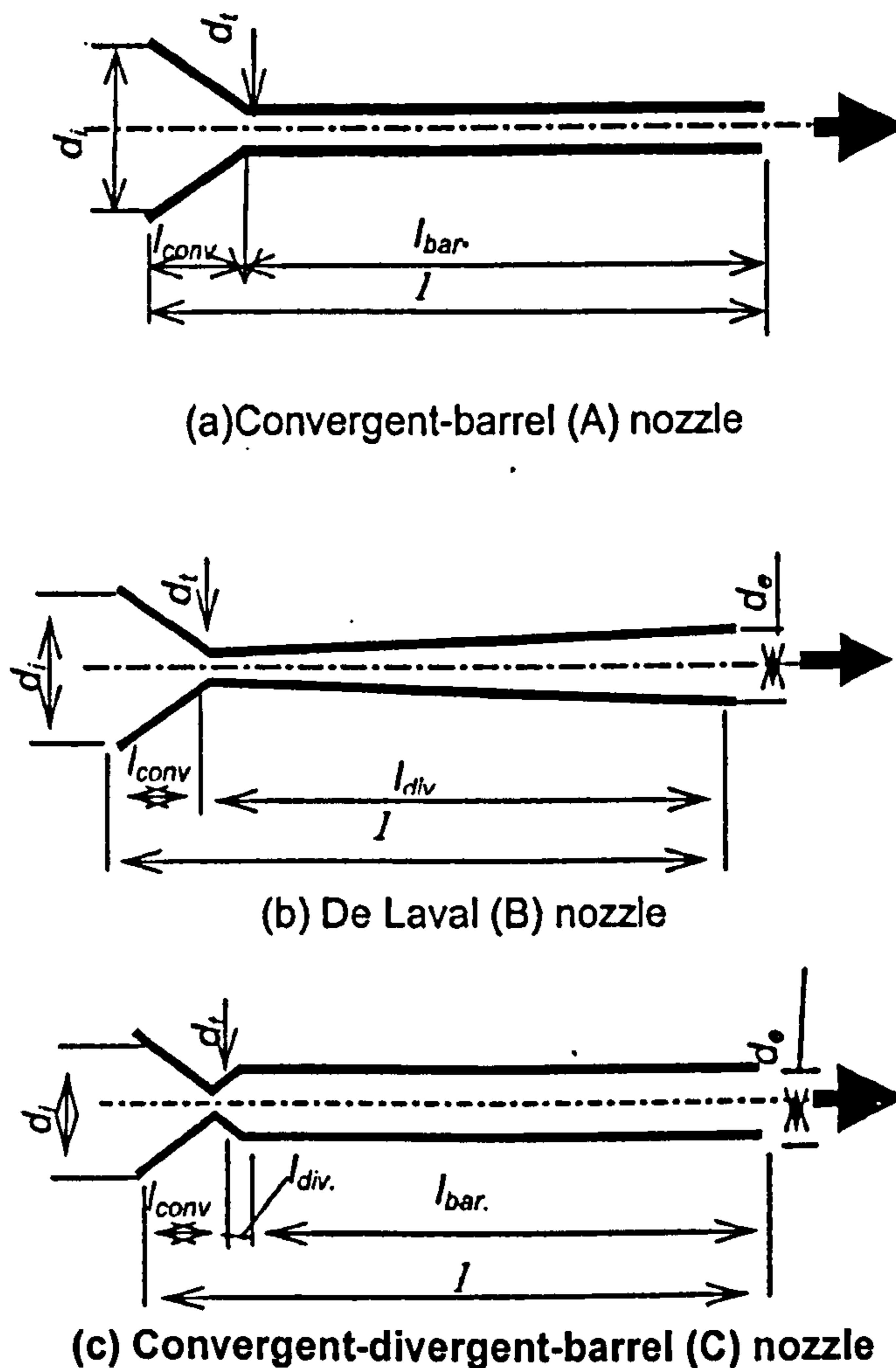
Figure 6.30: Schematic cross-section diagrams of the cold spray nozzles used by Sakaki et al.[63].
