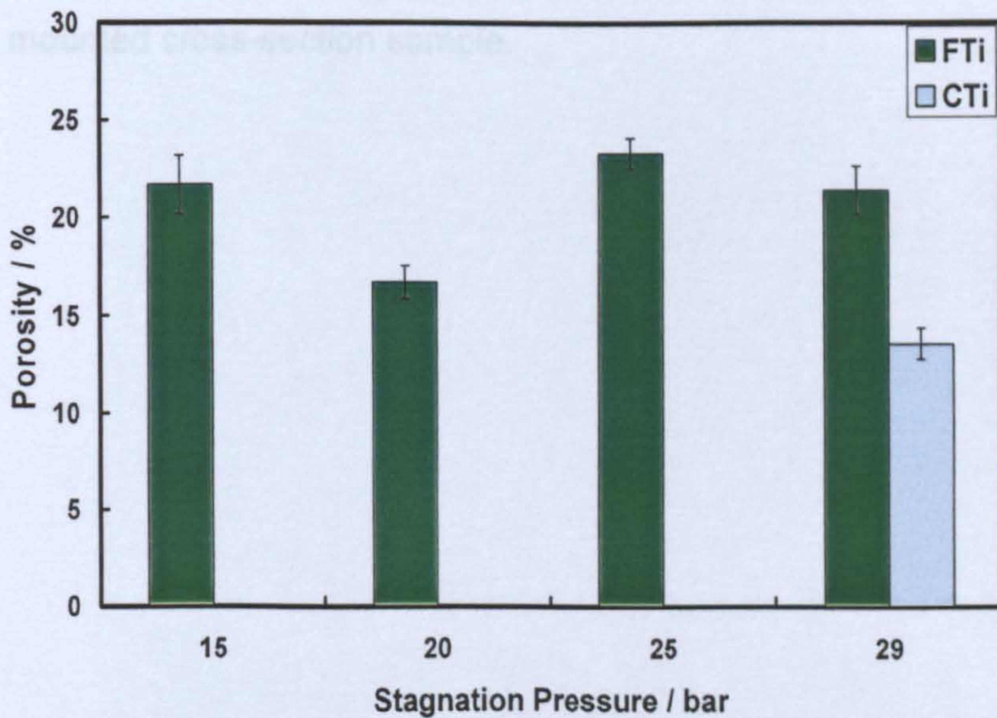
Figure 4.20: Porosity of deposits sprayed from FTi and CTi onto ground Ti6Al4V at different gas pressures; values were determined by image analysis, and error bars represent the standard error of the mean.
