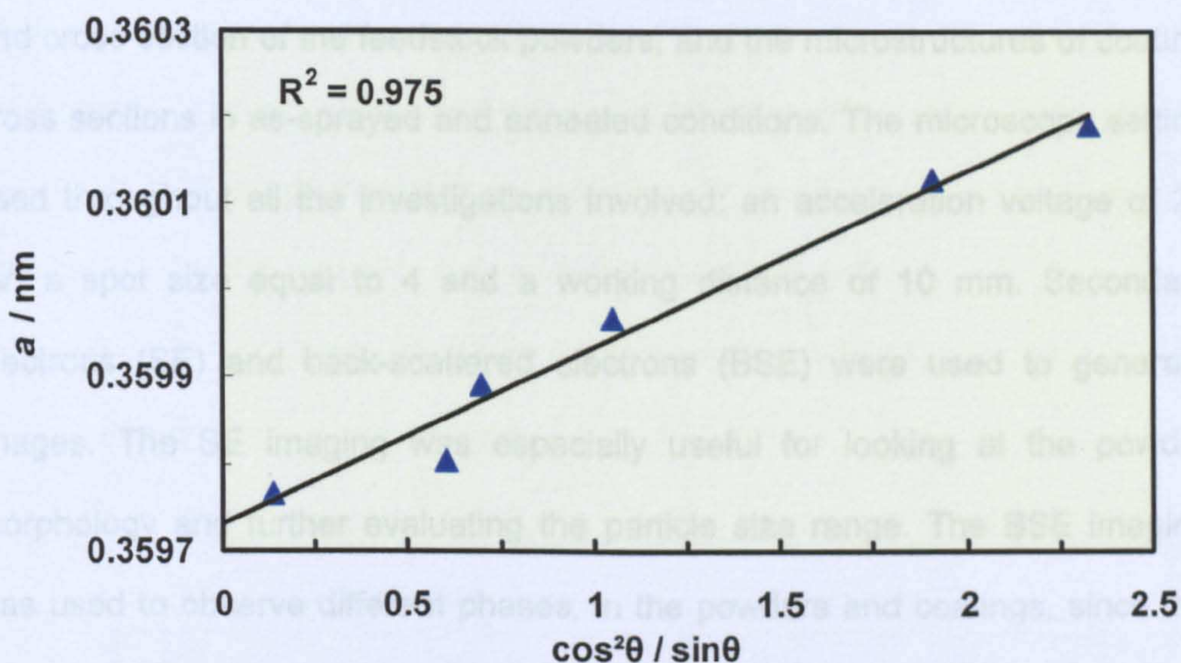
Figure 3.2: Example of extrapolation plot used to calculate the lattice parameters. Plot for powder C718.
