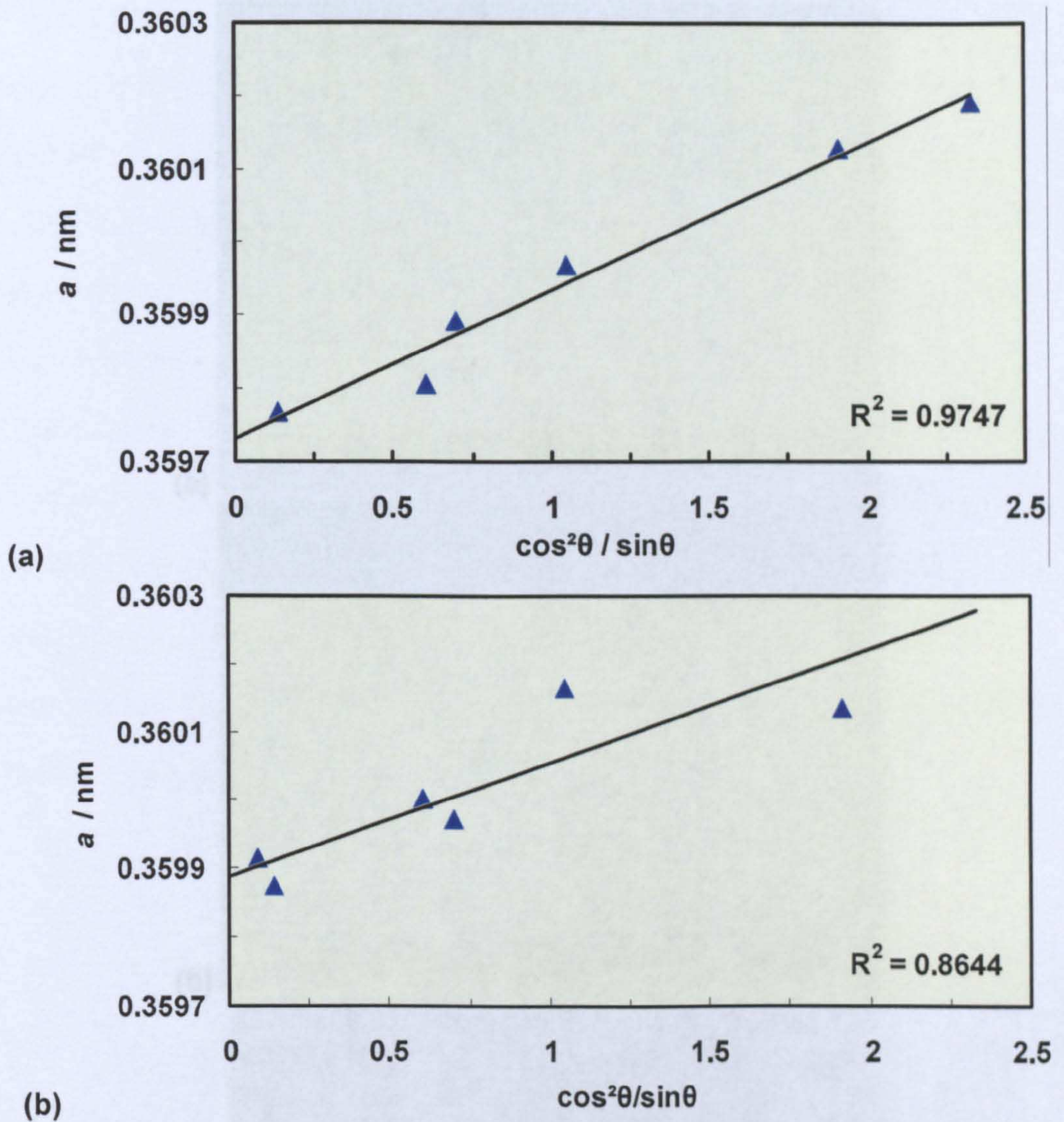
Figure 6.19: Extrapolation plots used to calculate the lattice parameter for (a) powder C718 and (b) coating LFHO.
