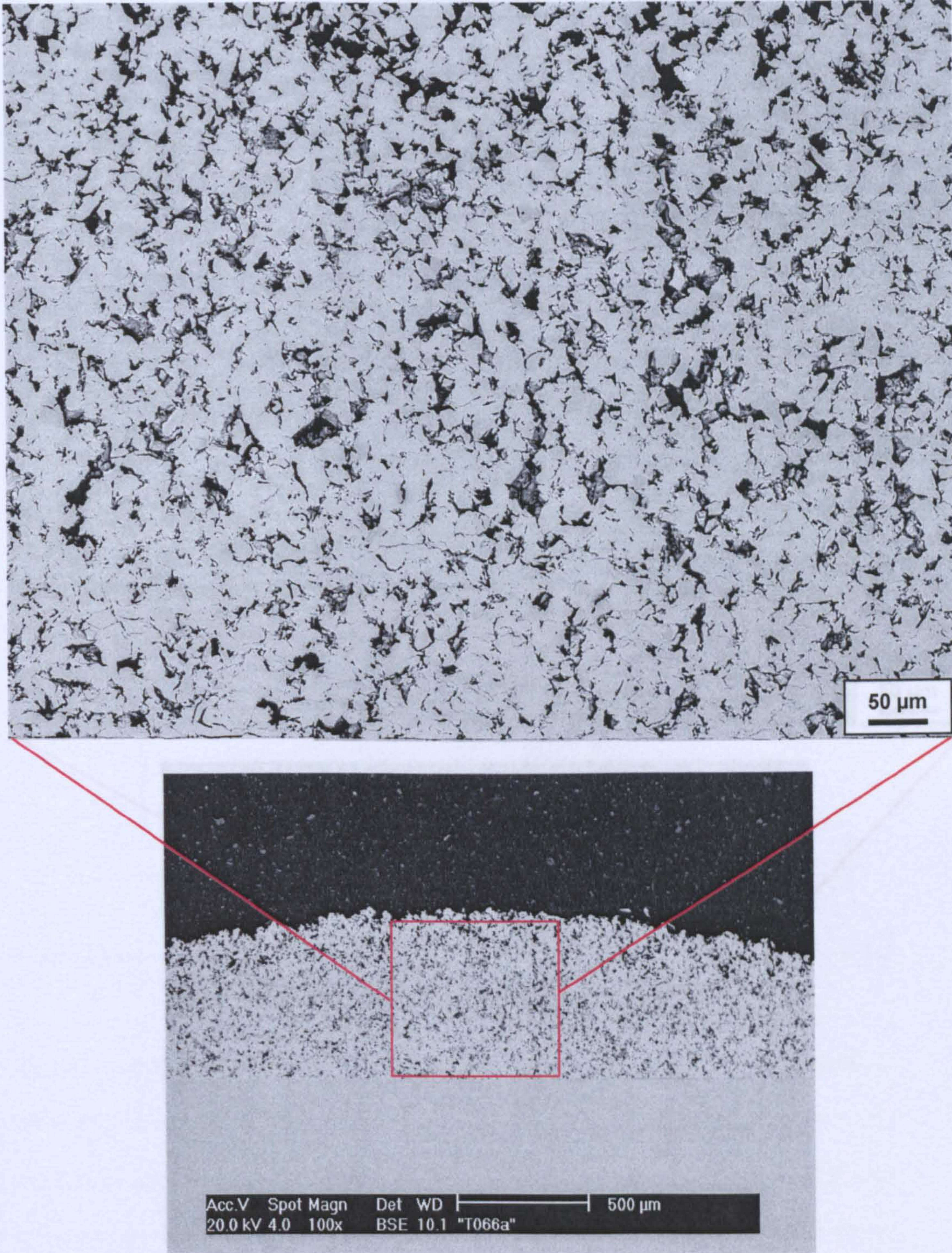
Figure 4.21: BSE-SEM image of Ti deposit sprayed at 29 bar using the FTi powder (substrate: Ti6Al4V).
