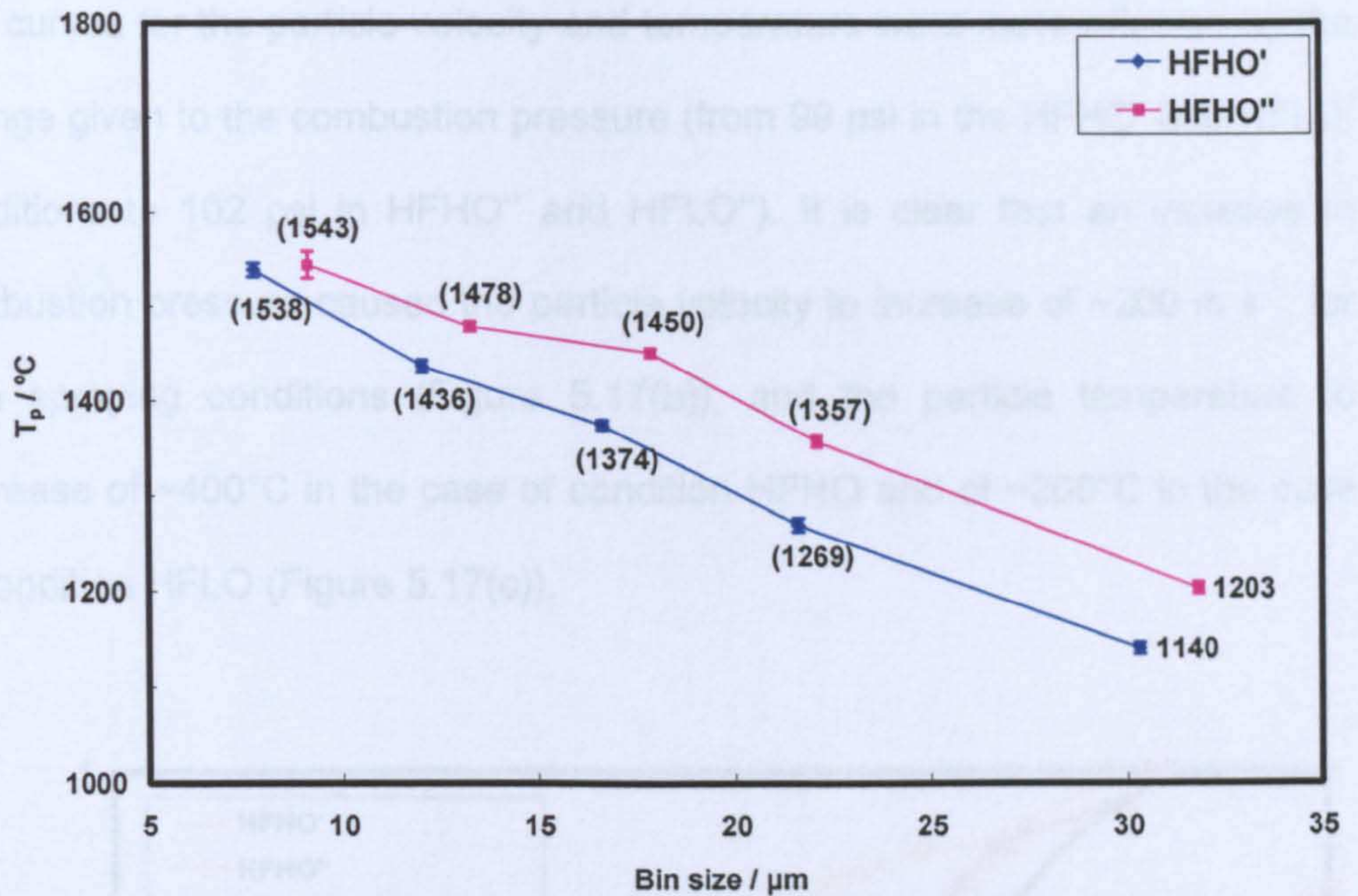
Figure 5.16: Particle size distribution (a), velocity (b) and temperature (c) as function of the bin size in two separate spraying sessions (in the graph labelled as 'prime' and 'double prime'). Spray condition: HFHO. SOD= 350 mm. The error bar represents the standard error of the mean.
