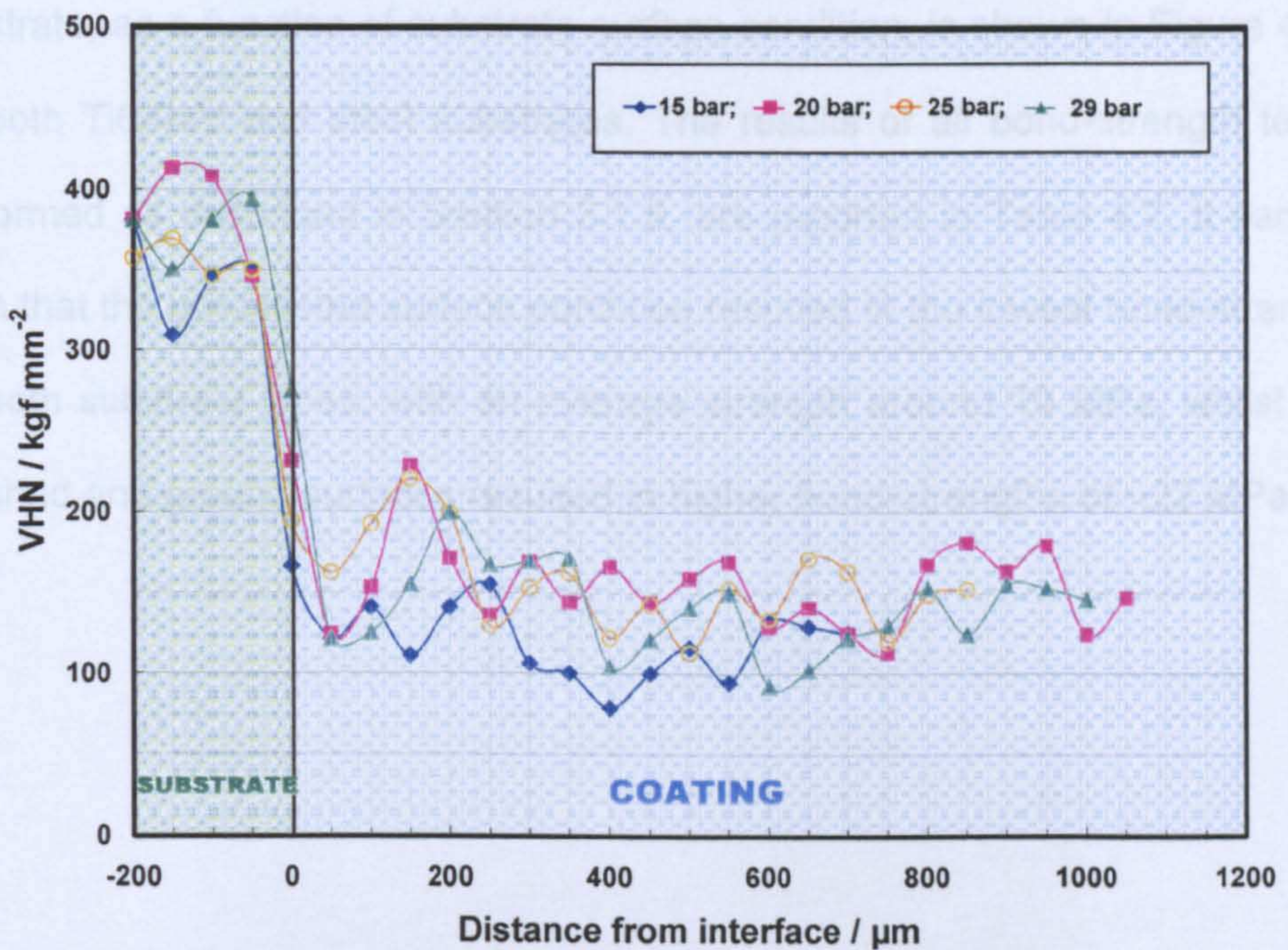
Figure 4.16: Microhardness profile of the coating sprayed from FTi at different gas pressures.
