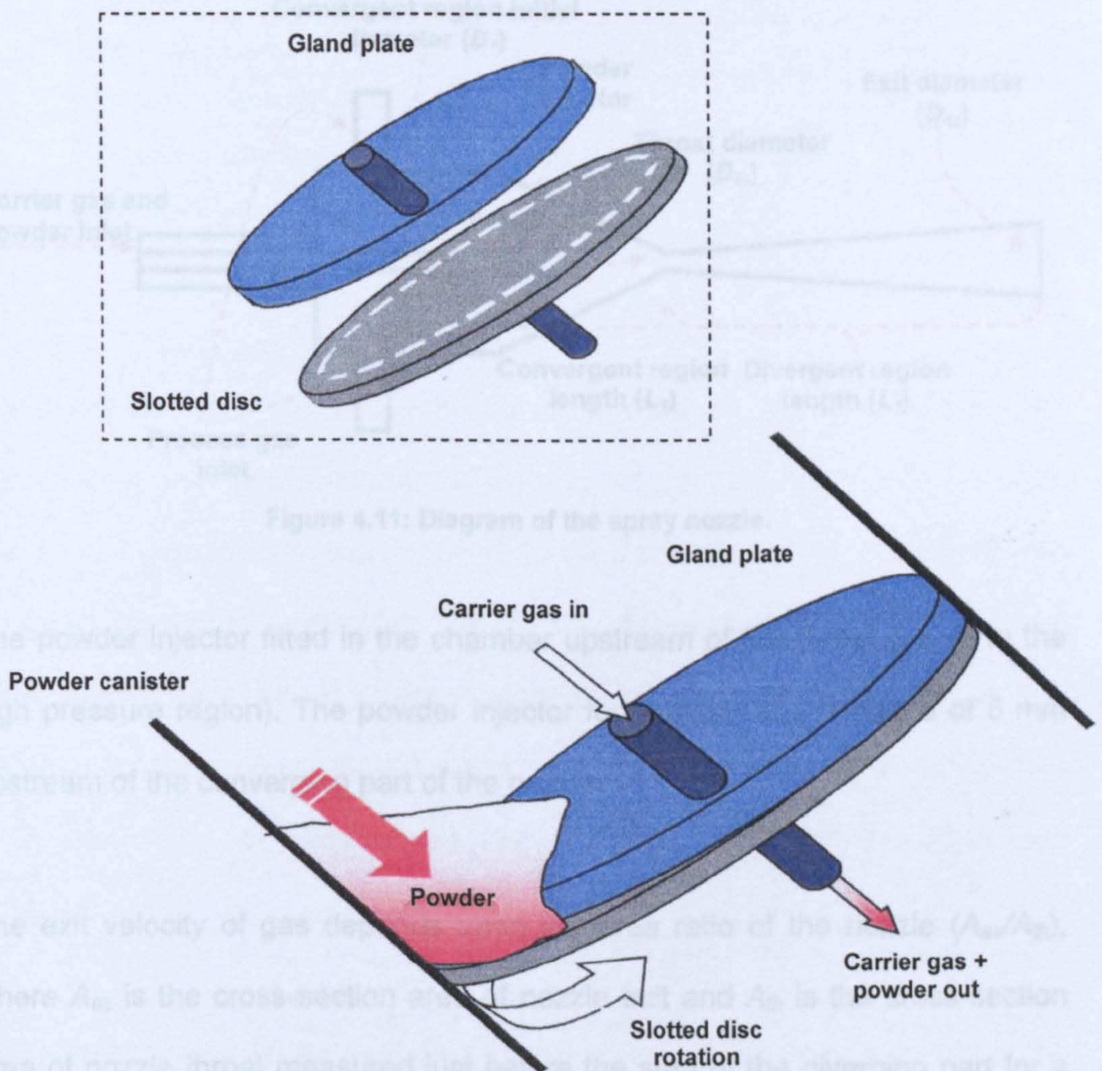
Figure 4.10: Schematic diagram showing the principle of operation of the powder feeder.
