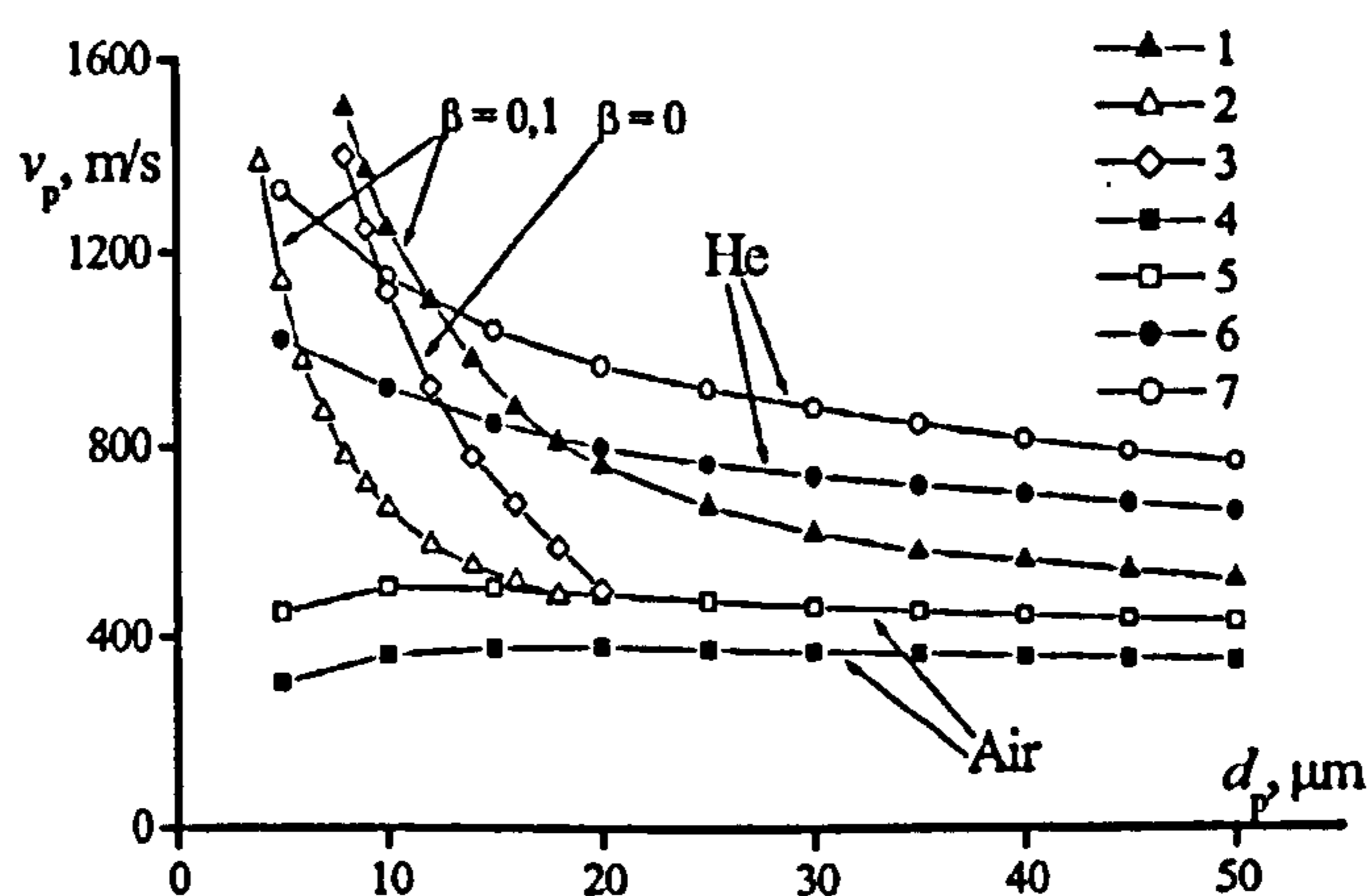
Figure 3.27: Diagram showing the particle velocity at which, upon impact, a Al particle achieves melting temperature as function of the particle size ( \beta is the coefficient of localisation of intensive deformation in the particle, 0 \leq \beta \leq 1 ) [55].
