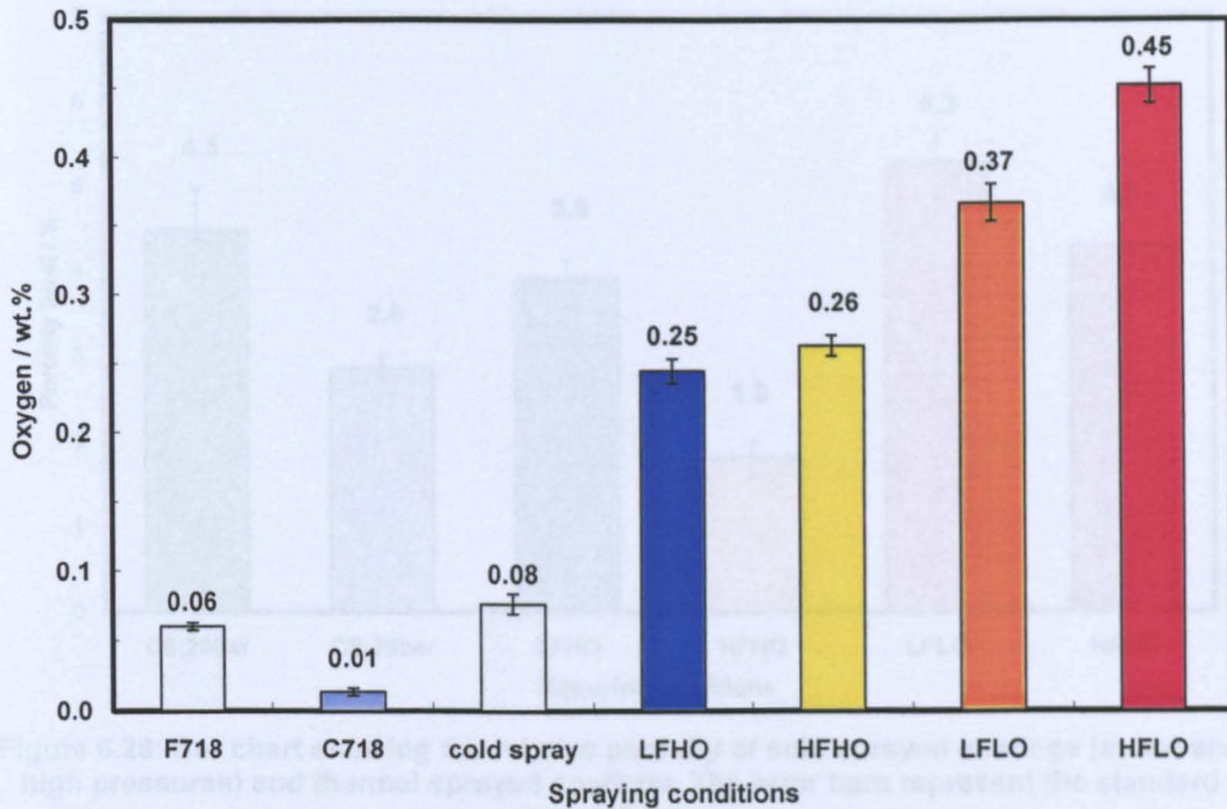
Figure 6.27: Bar chart showing the oxygen content of the feedstock powders, cold sprayed and thermal sprayed coatings. The error bars represent the standard error of the mean.
