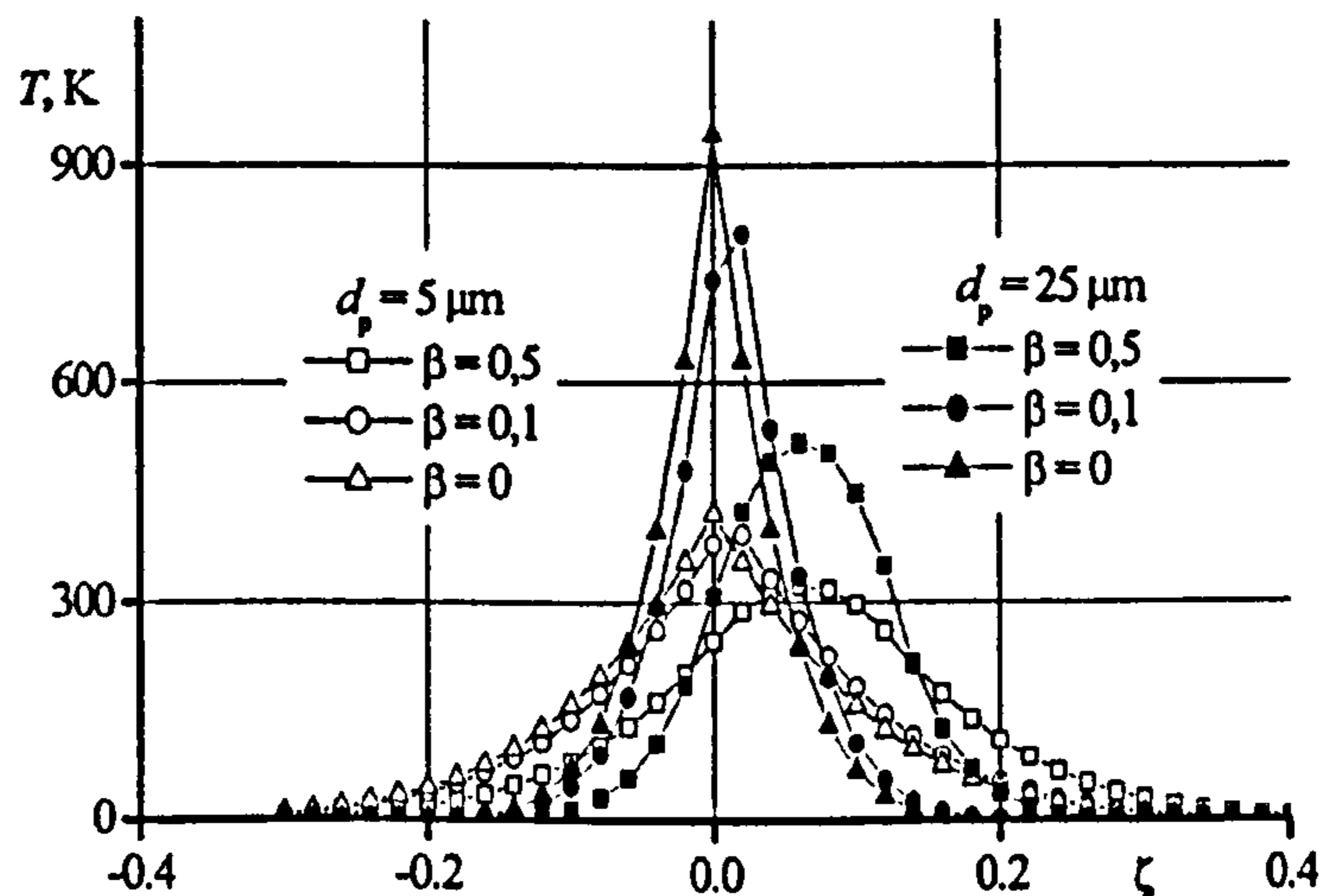
Figure 2.26: Distribution of temperature in the contact zone as a function of the size of a particle ( v_p = 1000 \text{ m s}^{-1} ; \beta is the coefficient of localisation of intensive deformation in the particle, 0 \leq \beta \leq 1 ) [55].
