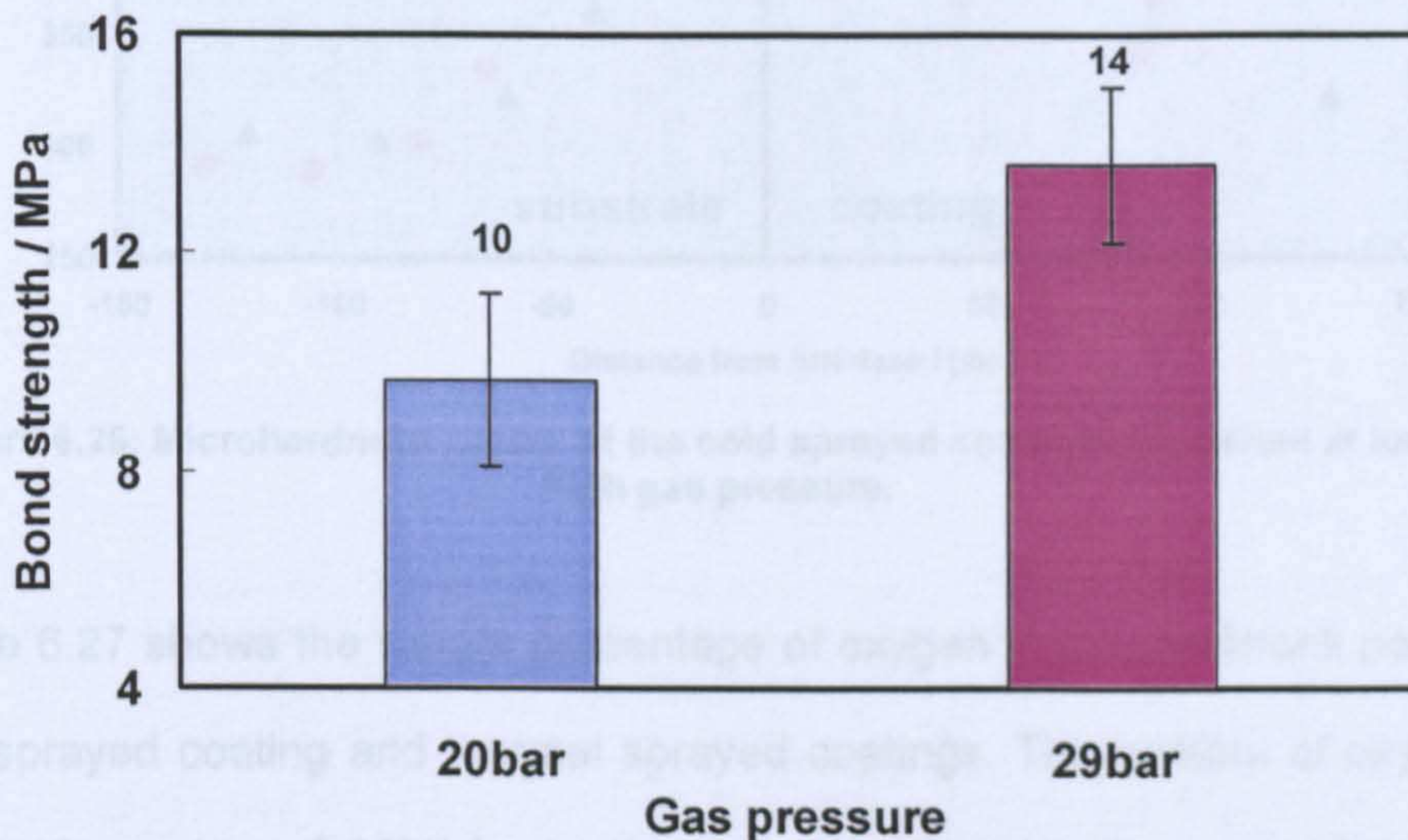
Figure 6.25: Bar chart showing the effect of gas pressure on the bond strength of cold sprayed deposits using F718 powder (The error bars represent the standard error of the mean).
