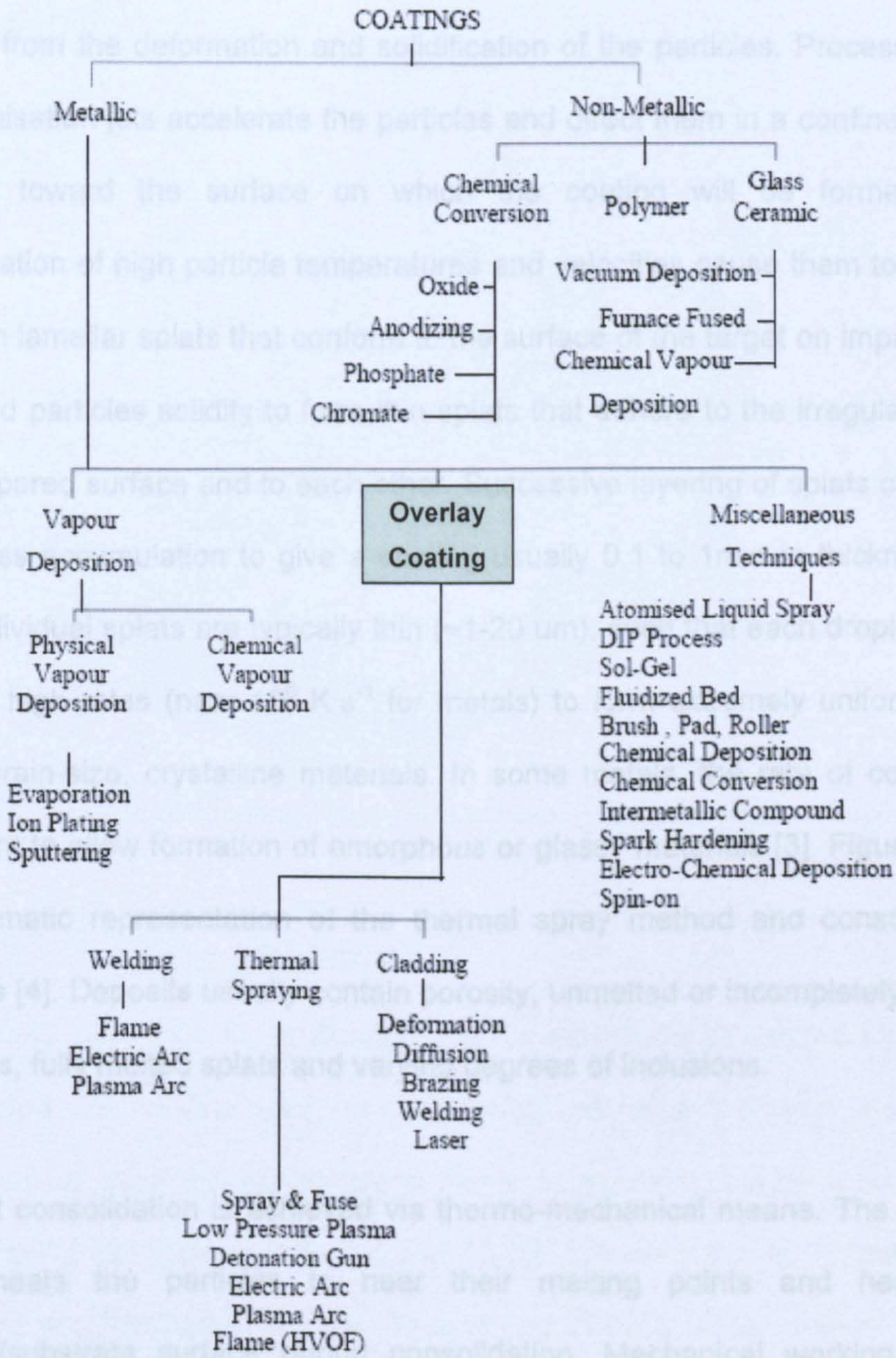
Figure 2.1: Coating deposition technologies [2].
