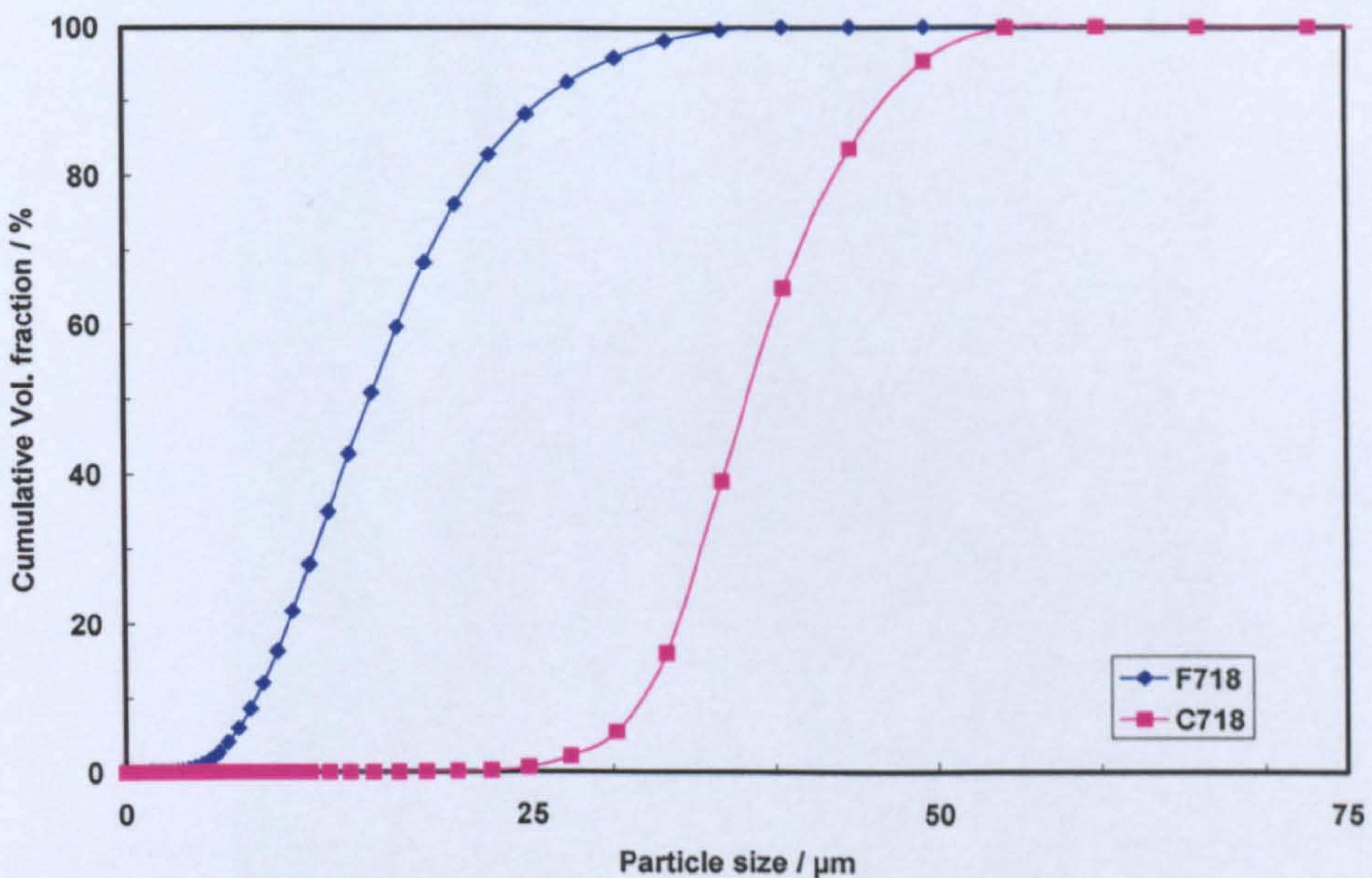
Figure 6.16: IN718 powder size distributions.
