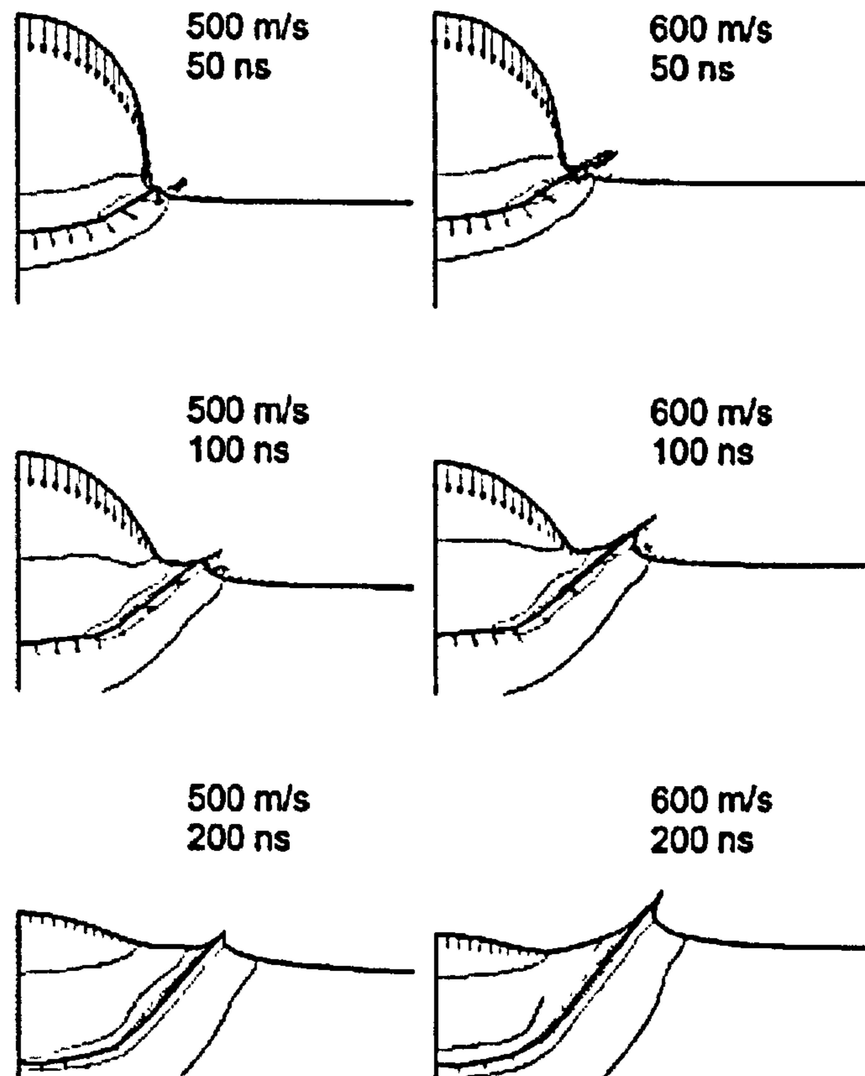
Figure 1.25: Simulated impact of a copper particle on a copper substrate, for the initial particle velocities of 500 and 600 \text{m s}^{-1} . The arrows represent the velocities of nodes at the respective surfaces of particle and substrate, and the contours indicate temperature distribution [45].
