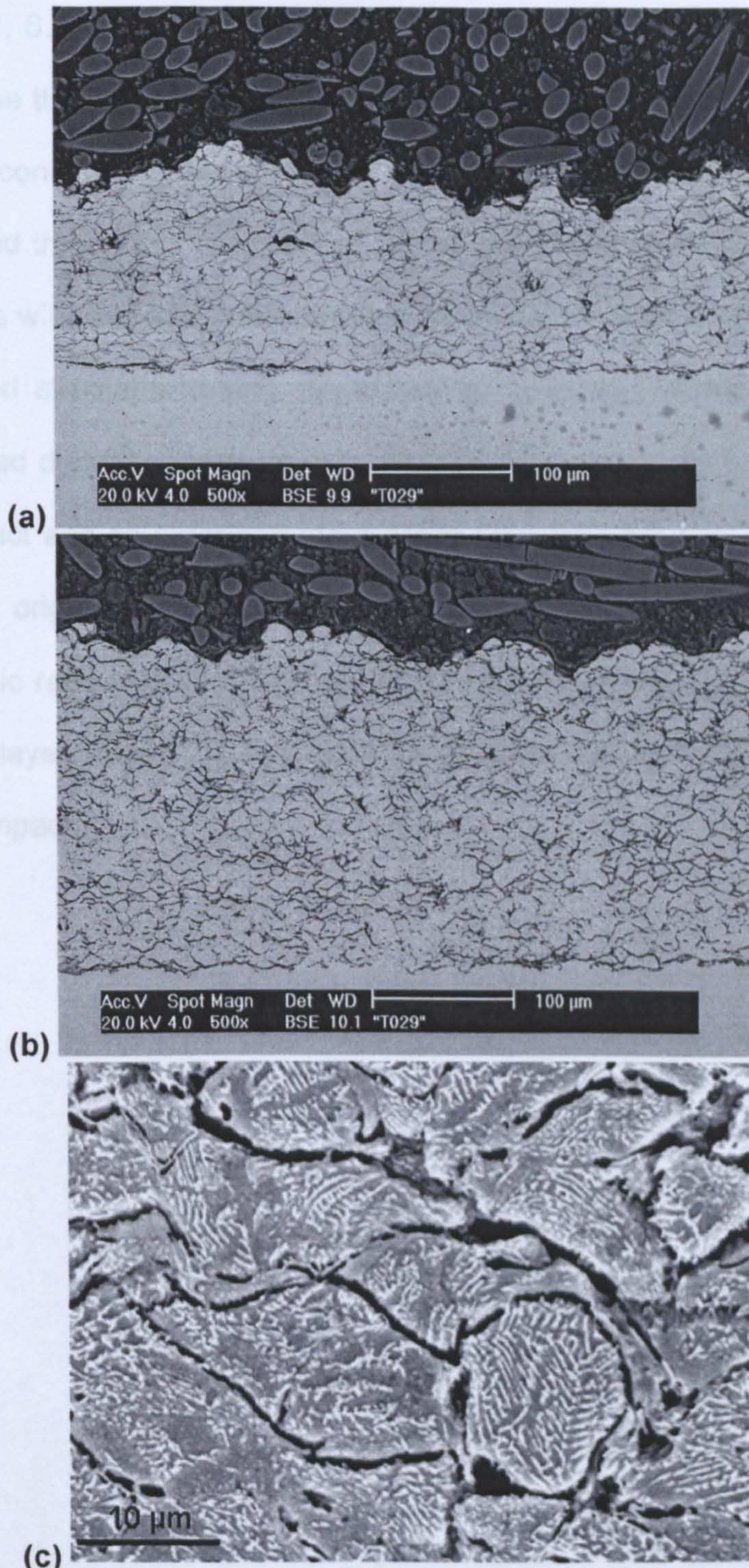
Figure 6.20: BSE images of the etched coatings cold sprayed at (a) 20 (thickness \sim 130 \mu\text{m} ); (b) and (c) 29 bar (thickness \sim 250 \mu\text{m} ). Kalling's Reagent 2 was used to etch the polished cross-sections.
