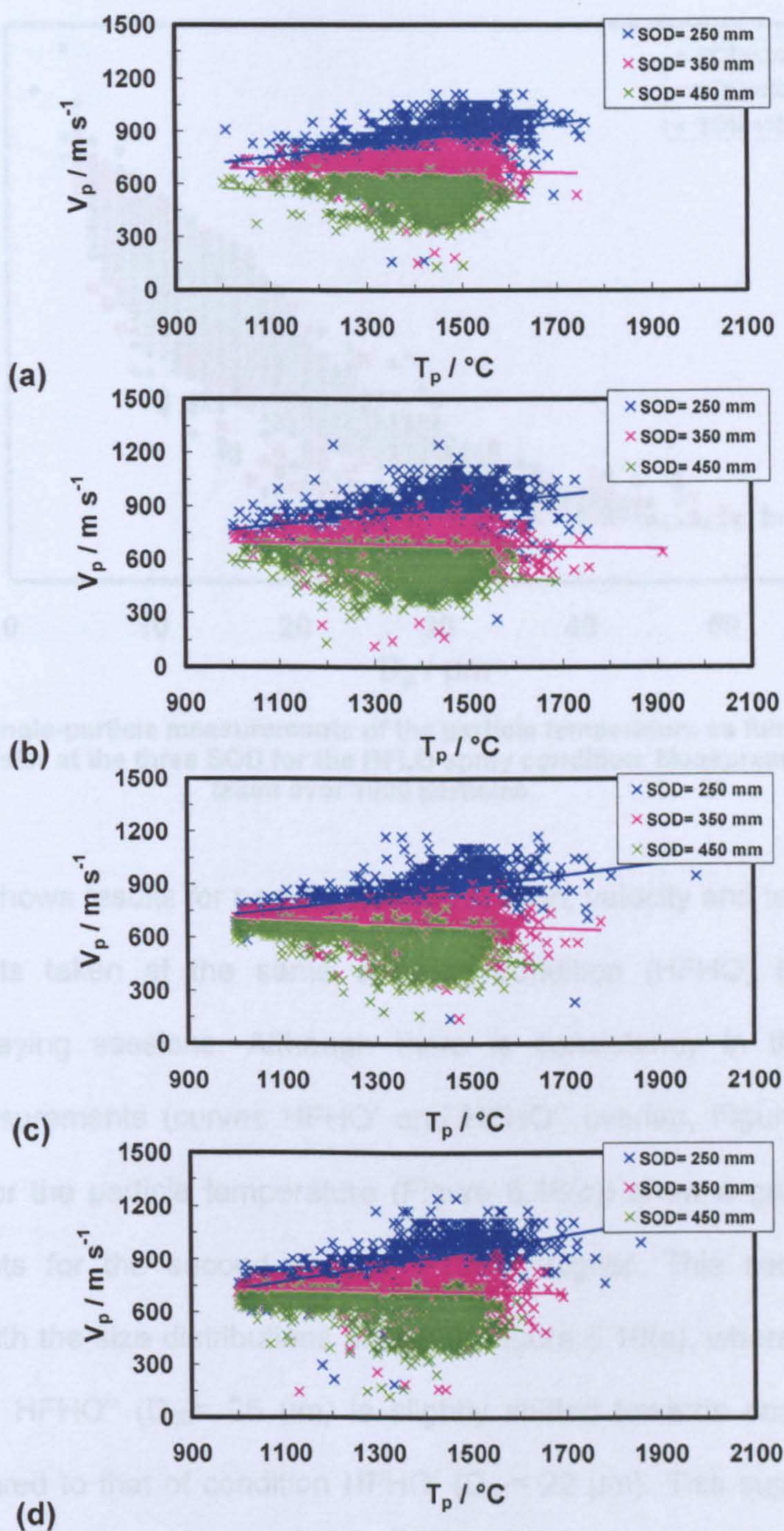
Figure 5.14: Single-particle measurements of the particle velocity as function of the particle temperature at the three SOD for the four spray conditions: (a) LFHO, (b) HFHO, (c) LFLO and (d) HFLO. The measurements were taken over 1000 particles.
