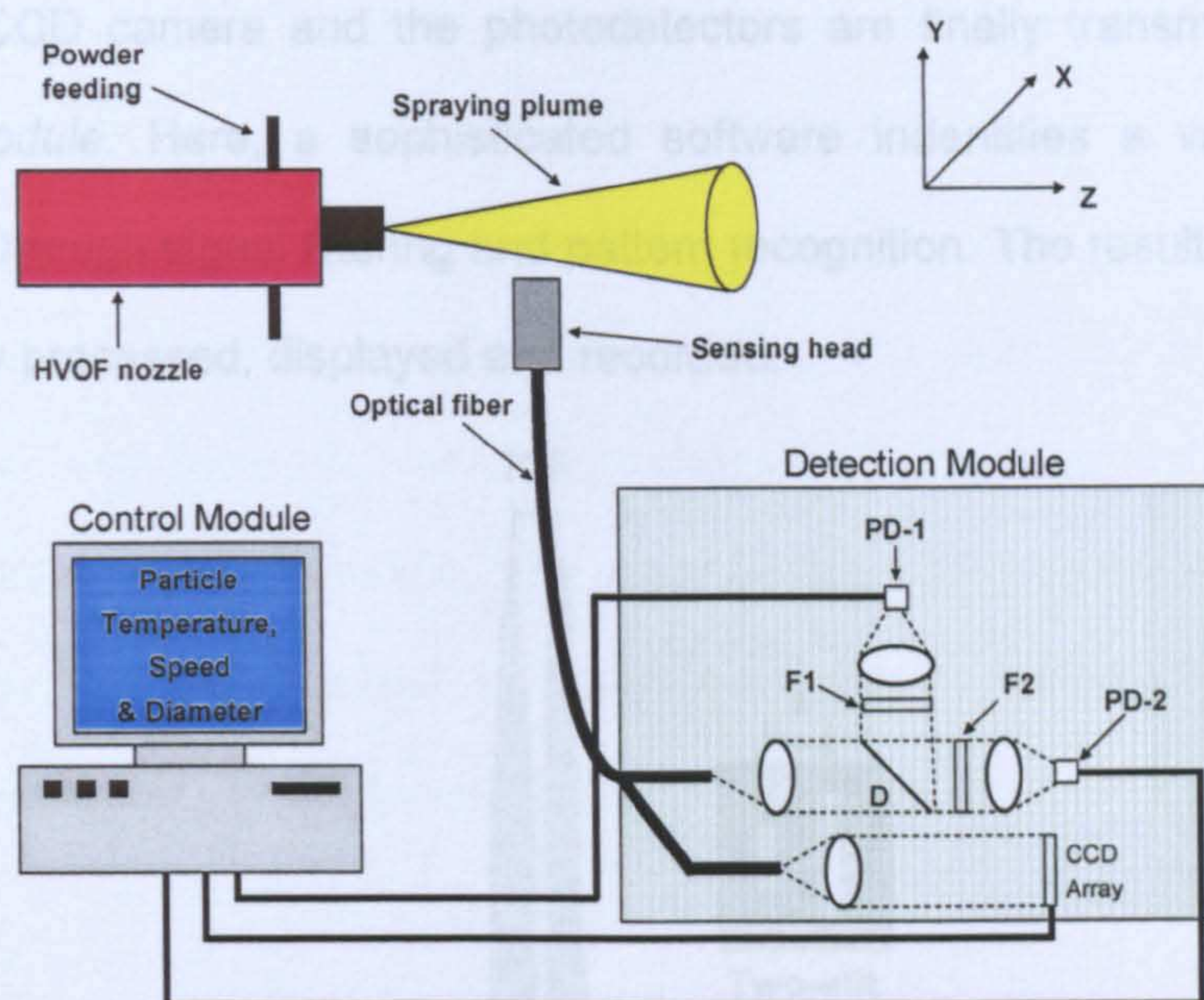
Figure 5.6: DPV – 2000 operating principles.
